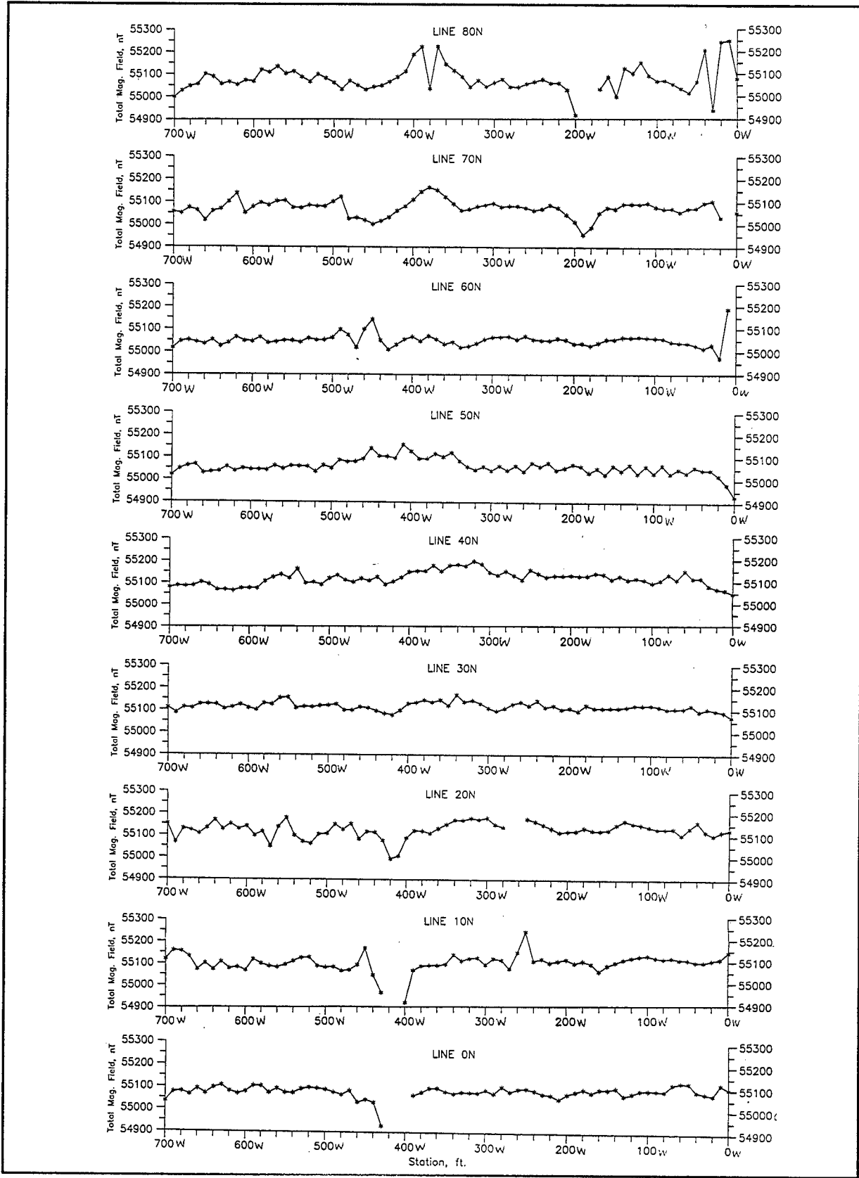
Figure 29. Total magnetic field test results, profile lines
