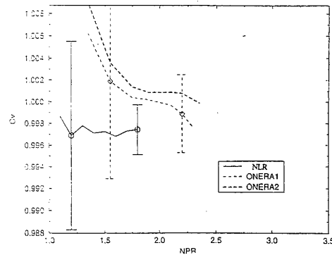
Figure 37 DNW 3" starboard cubic nozzle Velocity coefficient
