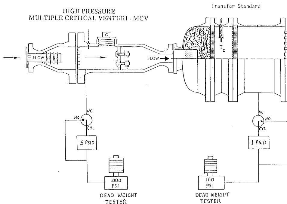
Figure 10 MCV airflow calibration Instrumentation schematic
