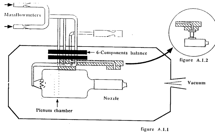
Figure A.1 Sketch of one of the ONERA test benches located in S4B
