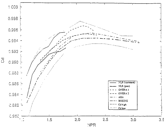
Figure 38 3" cubic nozzle Flow coefficient
