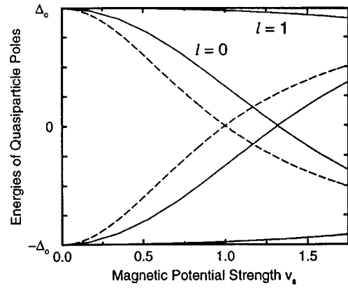
FIG. 1. Localized excited state poles for angular momentum channels \ell = 0 and 1 (solid lines). Dashed lines show results of Ref. [3]. At v_s = v_{s0} , the character of the \ell = 0 state changes from spin up to spin down.
