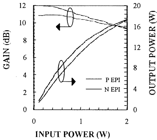
Fig.17(a) P_{in} - P_{out} data for bulk devices
