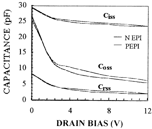
Fig. 13(a) Comparison of C-V plots for bulk devices
