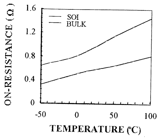
Fig.18 variation in on-resistance with temperature
