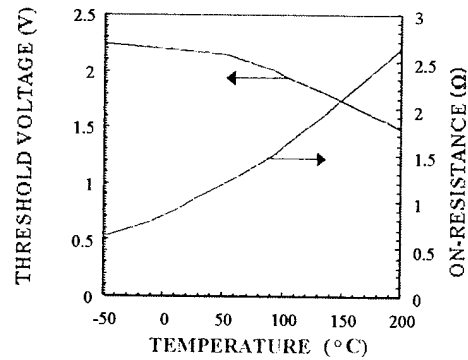
Fig.6 Variation of On-Resistance and V_{th} with temperature
