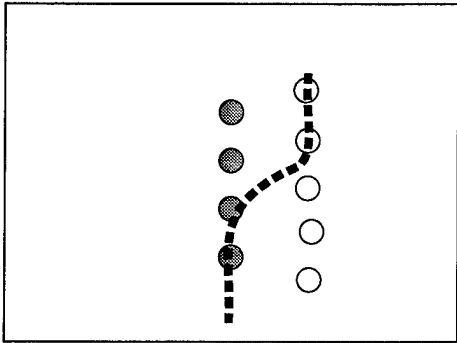
Figure 6.31 An overhead view of the real world locations of two sets of points chosen in two identical images, and the vehicle path through those points. When the vehicle receives the second set of points, it makes a sharp turn to the right to get on to the new path.
