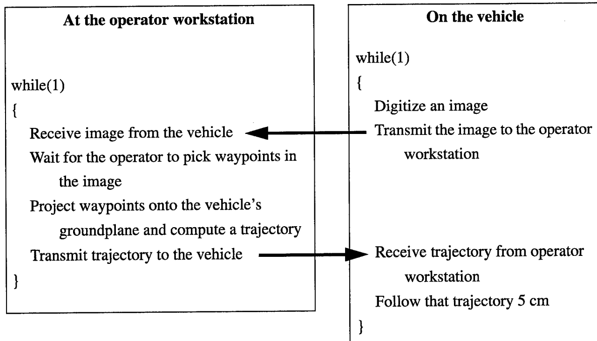
Figure 3.1 A Simple Discrete and Delayed Teleoperation Algorithm
