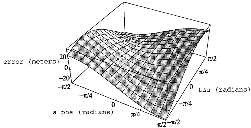
Figure 4.27 Y component of error in vehicle to camera yaw at d = 25m .
