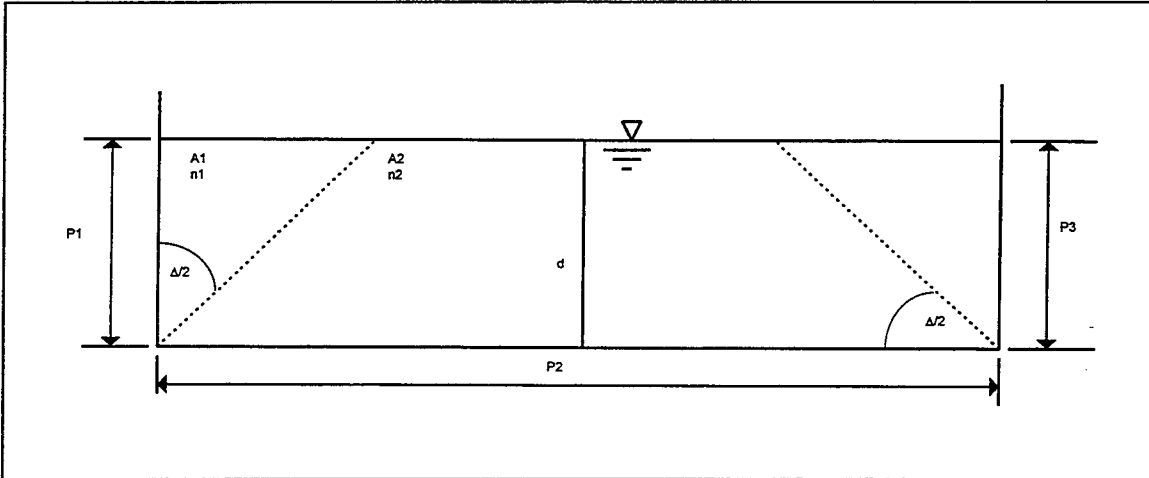
Figure 7. Definition sketch for Los Angeles District and Colbatch methods
