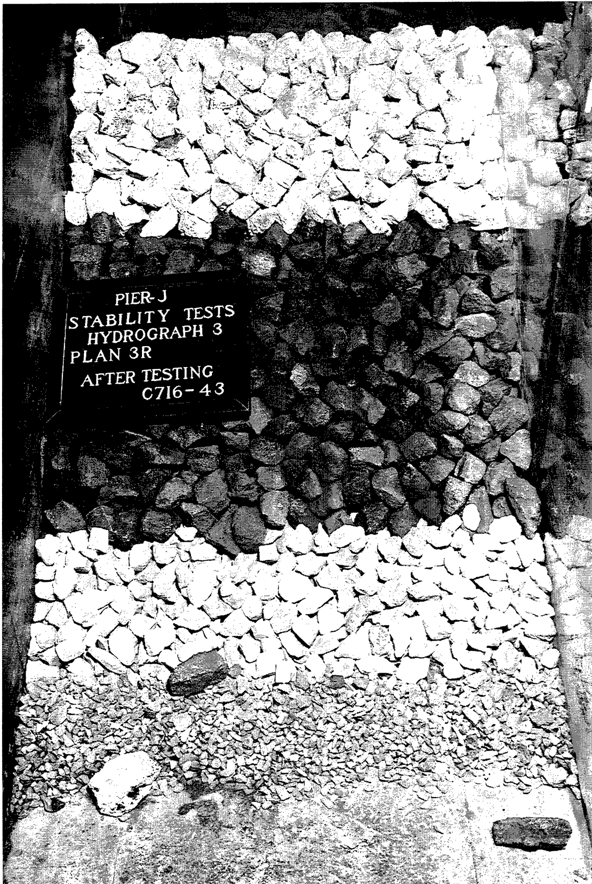
Photo 35. Sea-side view of Plan 3R at the conclusion of testing
