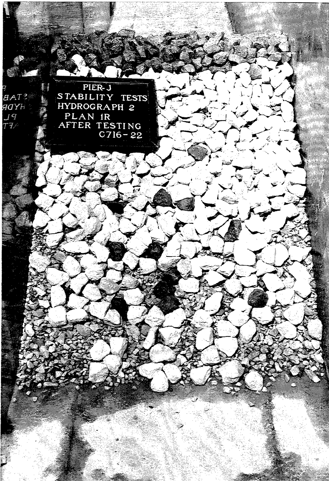
Photo 16. Harbor-view of Plan 1R at the conclusion of testing
