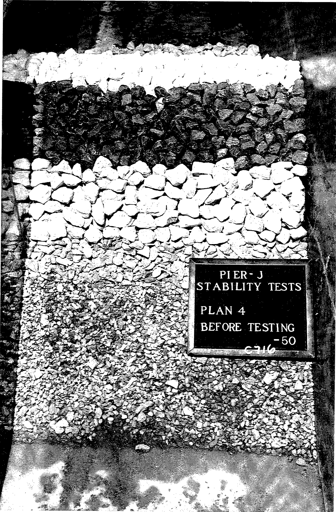
Photo 42. Harbor-side view of Plan 4 before wave attack
