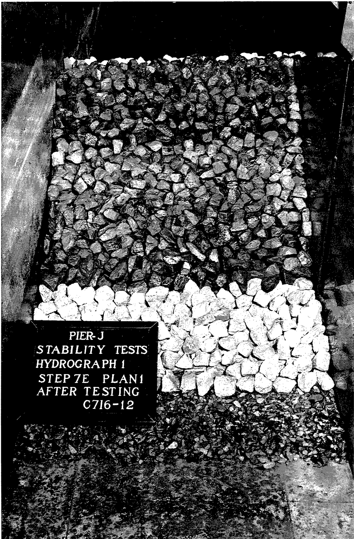
Photo 9. Sea-side view of Plan 1 after testing step 7 of Hydrograph 1
