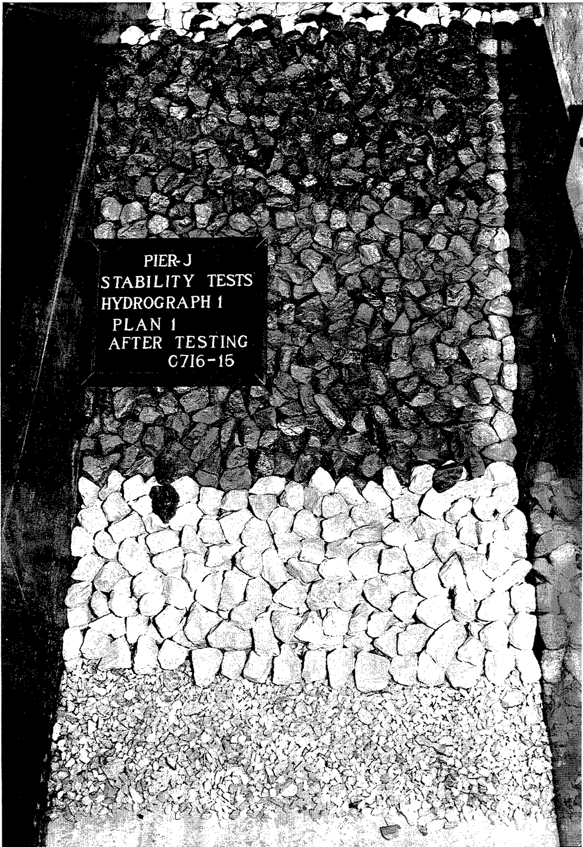
Photo 11. Sea-side view of Plan 1 at the conclusion of testing
