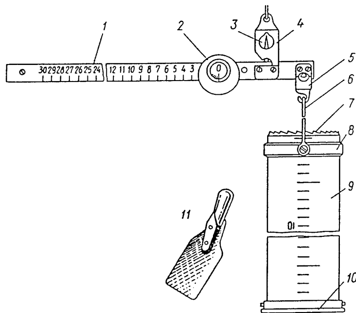
Figure 2. Model VS-43 snow-density gauge. 1 - index beam; 2 - movable weight; 3 - level indicator; 4 - fulcrum; 5 - hook; 6 - shackle; 7 - serrated cutting edge; 8 - movable ring; 9 - cylinder; 10 - cover; 11 - trowel.
