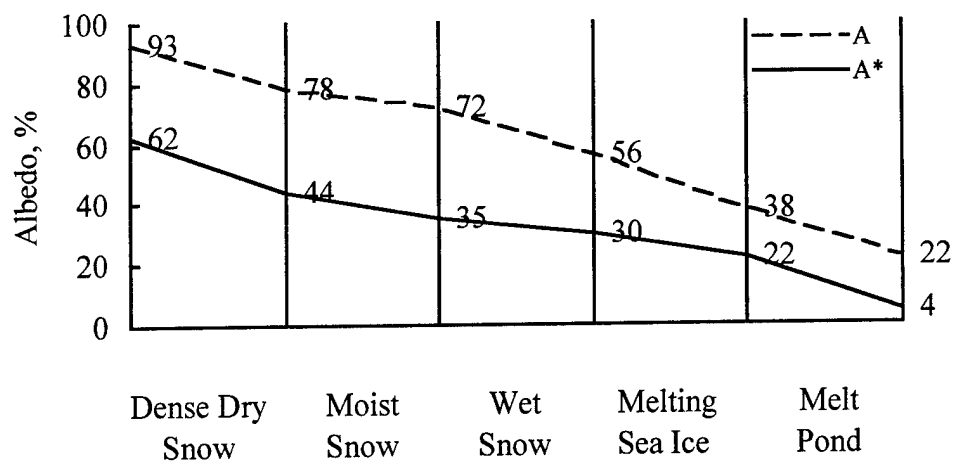
Figure 16. The limits of variability for the mean values of the integral albedo, A , and "spectral" albedo, A^* , for various surface types.
