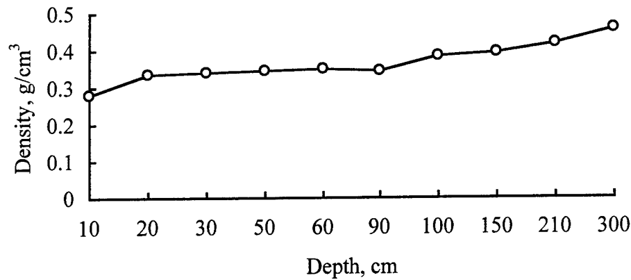
Figure 9. Mean snow density versus depth from the observations at NP-6.
