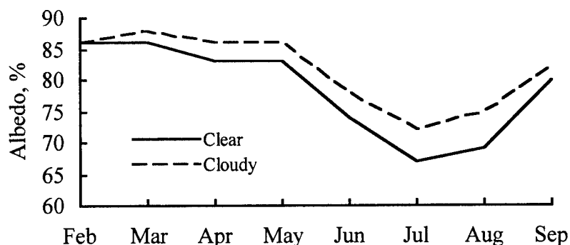
Figure 13. Multiyear mean monthly albedo values for clear and cloudy skies versus month.
