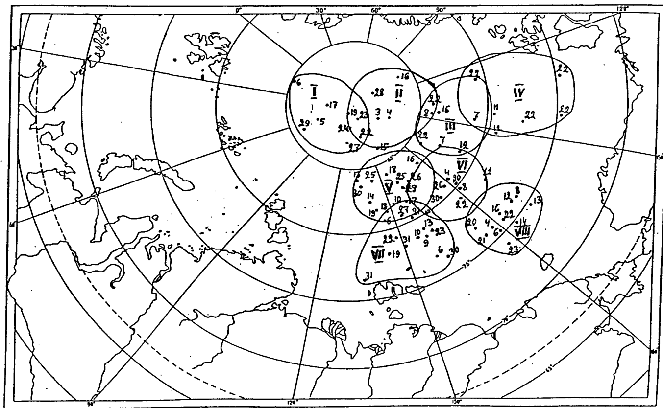
Figure 18. Eight groups of stations used for calculating multiyear mean values of the meteorological parameters for May. Arabic numbers associated with the points in each group indicate the numbers of the drifting stations.
