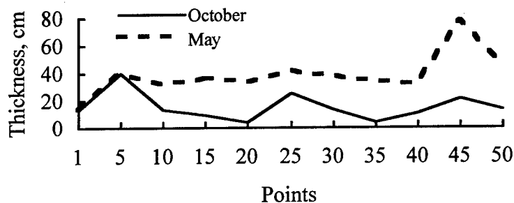
Figure 3. Snow depth data from the snow-line measurements at station NP-22.
