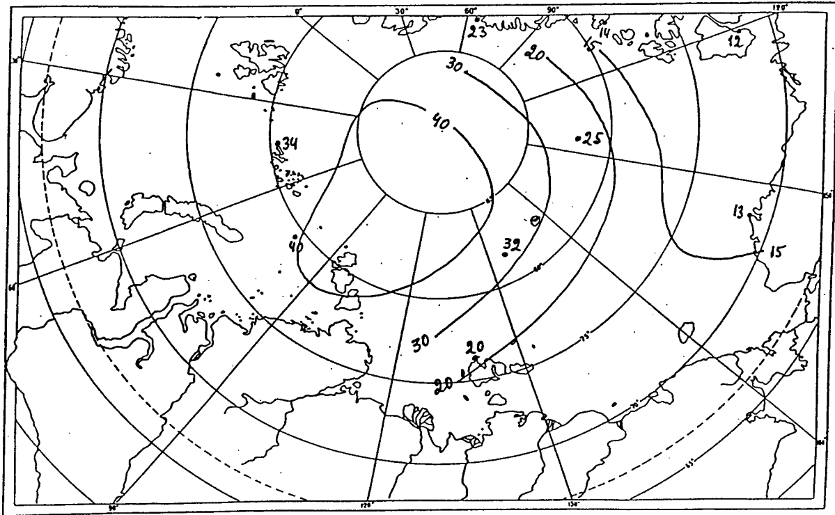
Figure 26. Map of the snow cover depth for May 1958 referenced to the central point of the drift of all NP stations.
