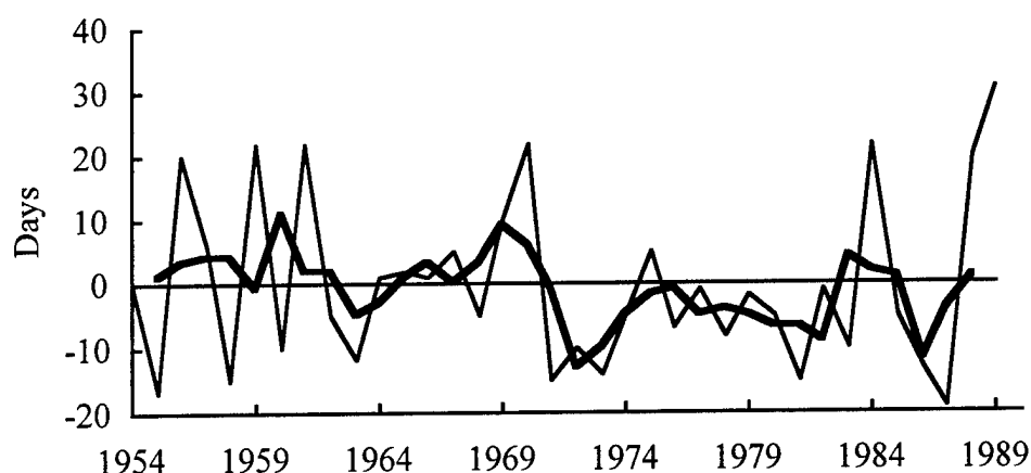
Figure 29. Anomalies [variations about the mean] in the dates of snow-cover destruction; the thick line denotes a 3-year running mean.
