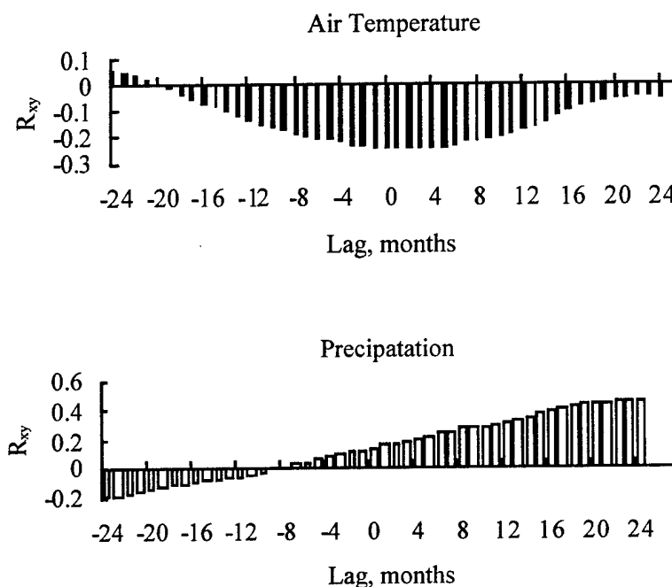
Figure 33. Correlation functions ( R_{xy} ) between variations of the smoothed intermonthly anomalies for (top) air temperature and snow thickness and (bottom) amount of precipitation and snow thickness.
