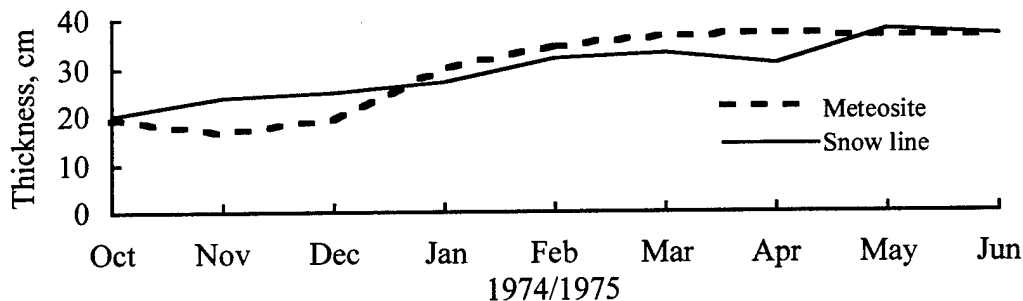
Figure 4. Snow-depth data from the meteosite and from the NP-22 snow-line survey for the period October 1974 to June 1975.
