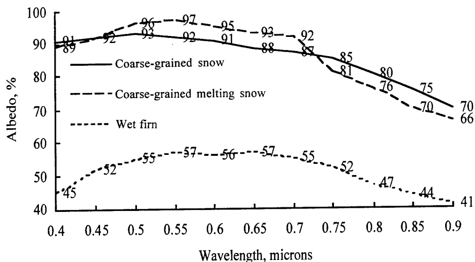
Figure 17. Spectral albedo of different types of snow surfaces versus wavelength.
