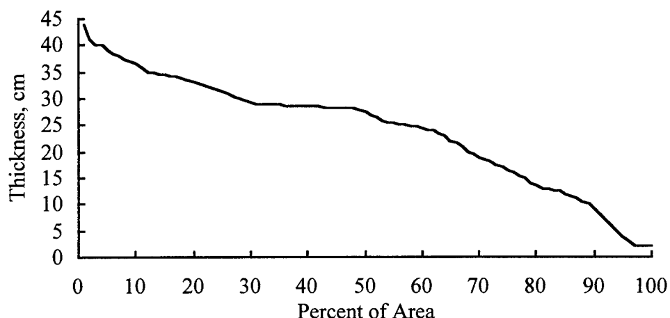
Figure 22. Curve showing the integrated (cumulative) snow-depth distribution.
