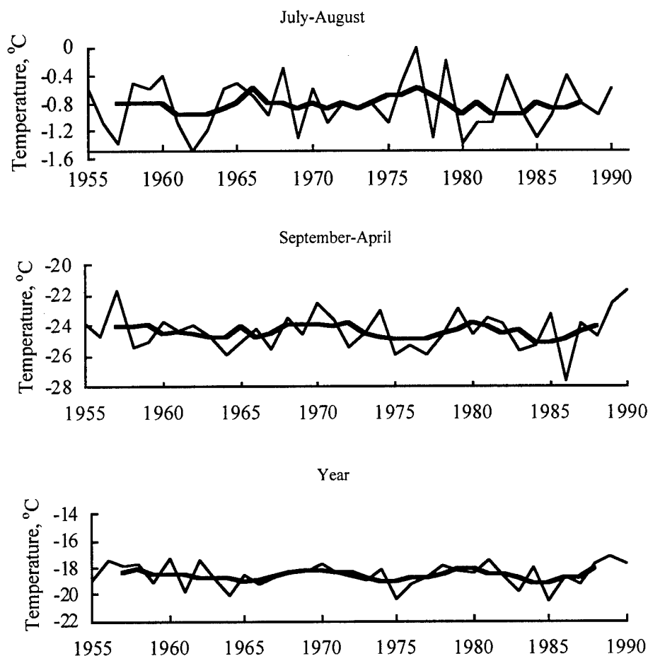
Figure 32. Interannual variability and 5-year running means of air temperatures in the Arctic Basin for the warm season, the cold season, and the annual average.
