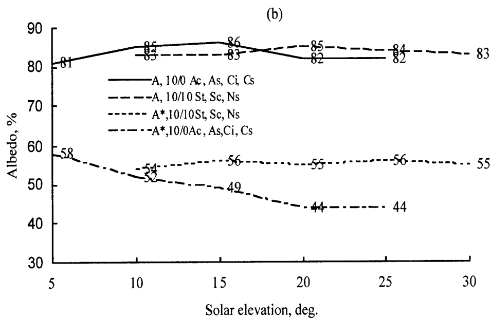
Figure 15. Diurnal variations of integrated albedo, A , and "spectral" albedo, A^* , for clear skies (a) and for cloudy skies (b).
