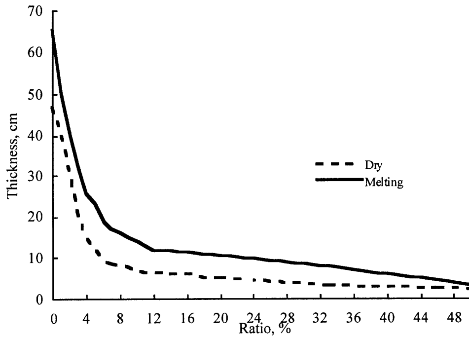
Figure 11. Snow depth versus ratio of outgoing to incident solar radiation (%)
