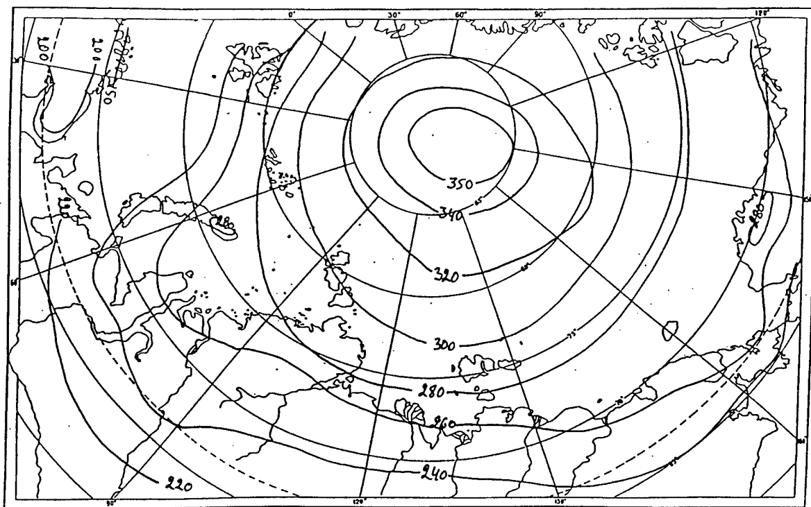
Figure 25. Number of days with a snow cover (per year).
