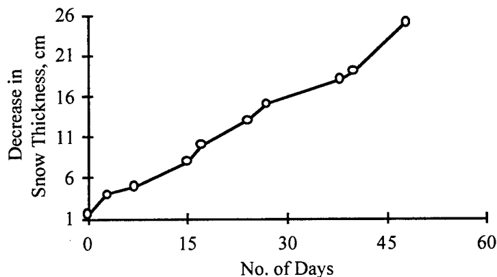
Figure 7. The relation between decrease in snow thickness and the total number of days with a positive mean temperature.
