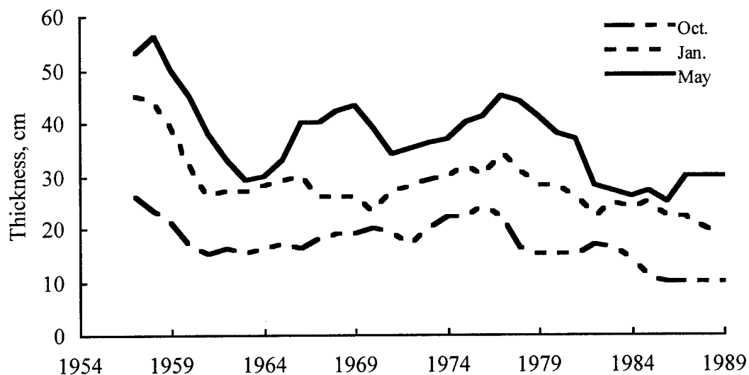
Figure 30. Snow-cover depth smoothed with a 5-year running mean.
