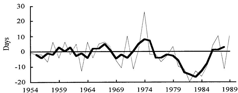
Figure 28. Anomalies [variations about the mean] in the dates of snow-cover formation; the thick line denotes a 3-year running mean.
