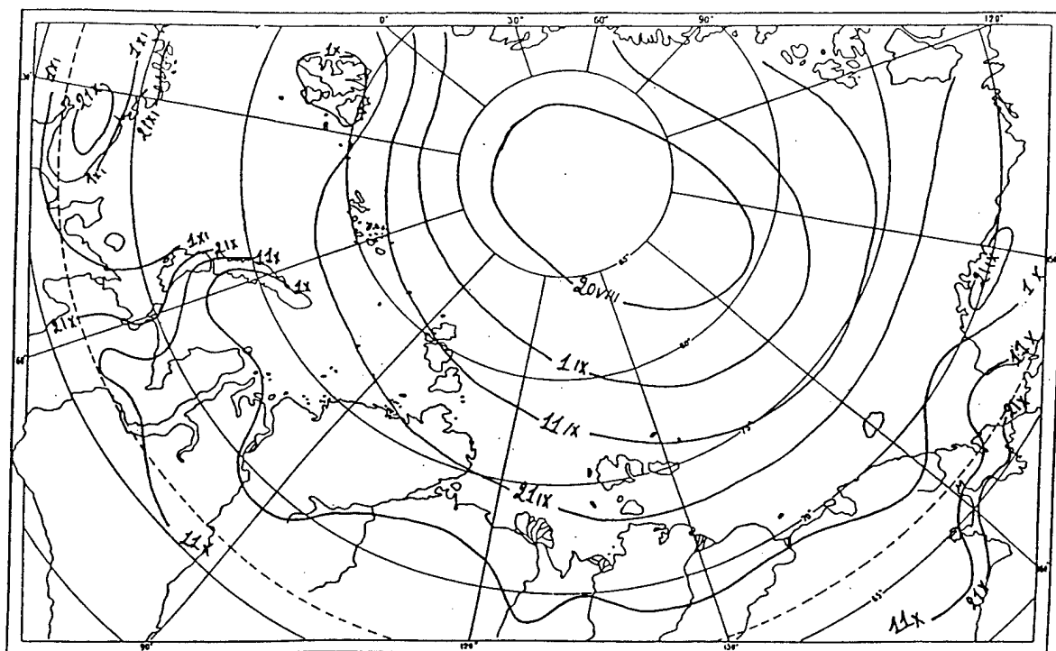
Figure 23. Dates of stable snow-cover formation. [Roman numerals denote the month; i.e., 21IX = 21 September.]
