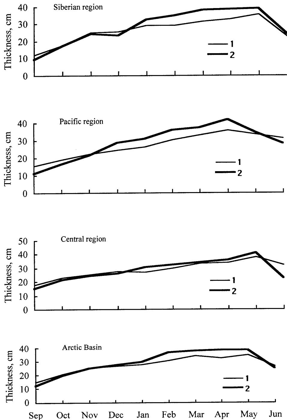
Figure 20. Annual progression of snow depth (cm) as calculated from the snow-line data and from the observations at the meteorological sites in the various regions of the Arctic Basin. 1- Thicknesses on the snow-line surveys. 2 - Thicknesses at the meteorological sites.
