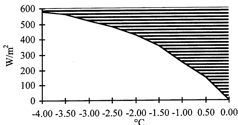
Figure 6. Onset of melting in the snow cover (shaded region) as a function of air temperature and the intensity of the incident solar radiation.
