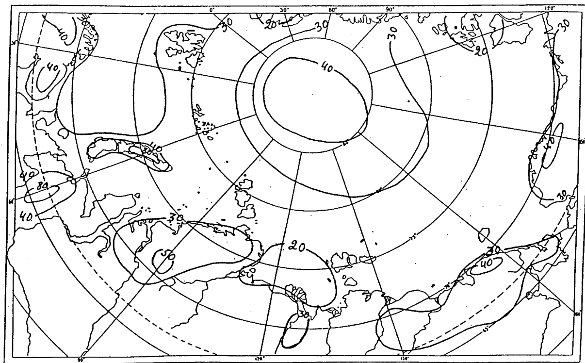
Figure 19. Distribution of the snow-cover depth (cm) in the Arctic during May.
