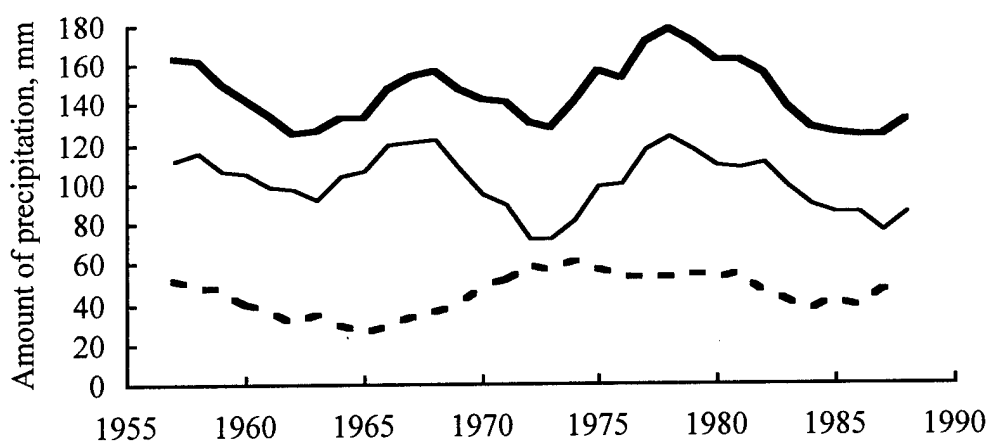
Figure 31. Amounts of precipitation smoothed with a 5-year running mean. The thick solid line is the yearly total, the thin solid line is the total for the cold season, and the dashed line is the total for the warm season.
