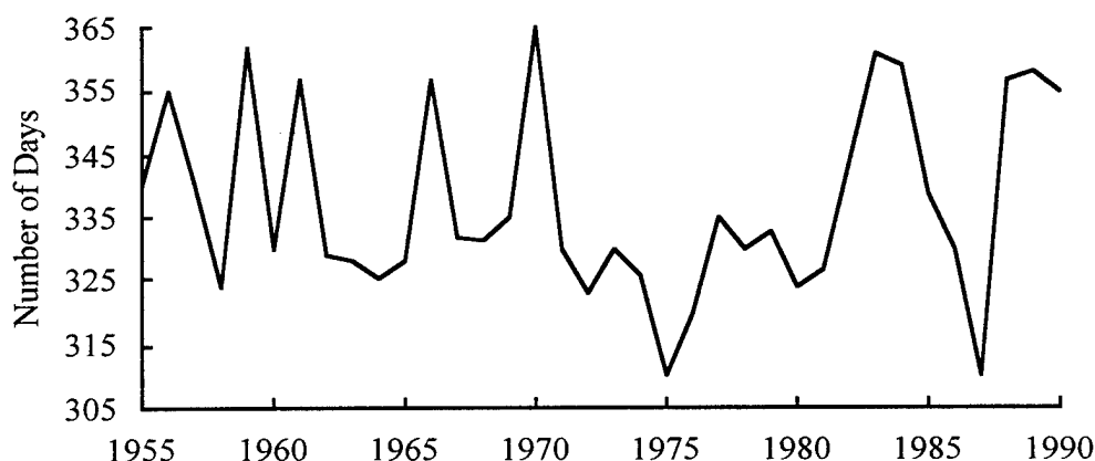
Figure 27. Number of the days with a snow cover in the Arctic Basin.
