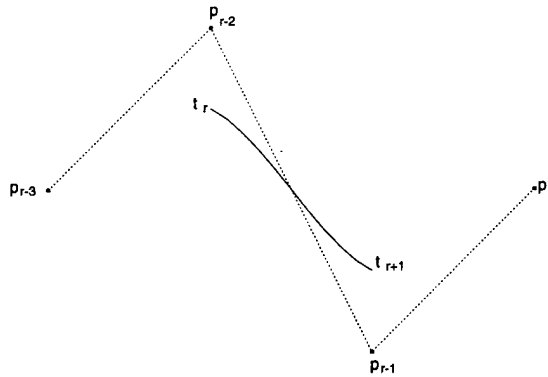
Figure 3-5: A Cubic B-spline Curve Segment with Control Polygon
