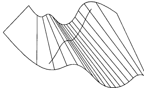
Figure 6-3: Geodesic on a Degree (4,1) Developable Surface
