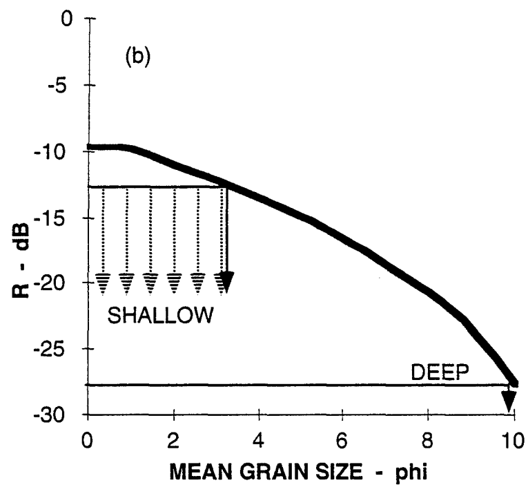
Figure 10. Reflection loss predictions by BOGGART v.3 as functions of (a) porosity and (b) grain size.
