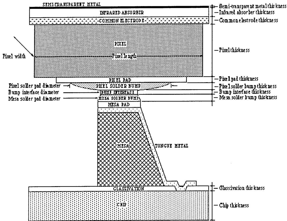
Uncooled infrared focal planar array model.
