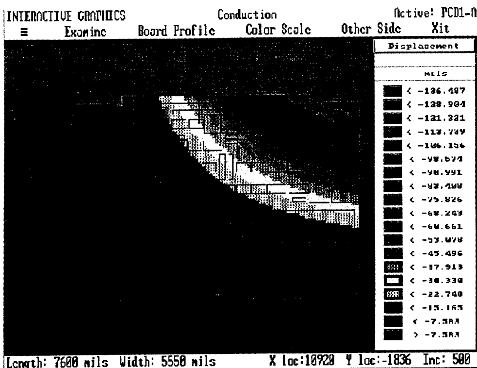
Graphical display of PWB in-plane motion analysis.
