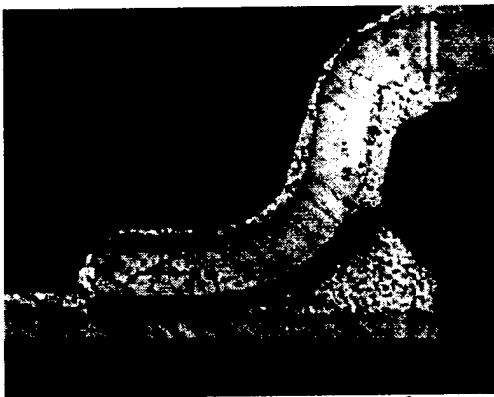
TSOP Solder Joint Fatigue Failure
