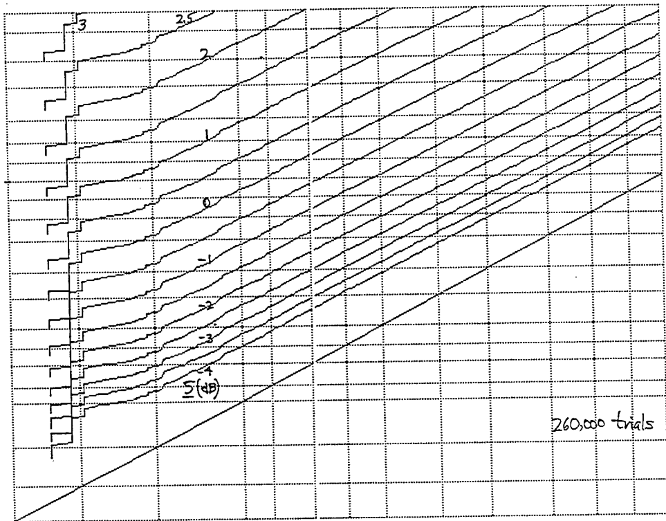
Figure F-19. ROC for M = 256 , \nu = 2.5 , \mu = 0 , N = 1024
