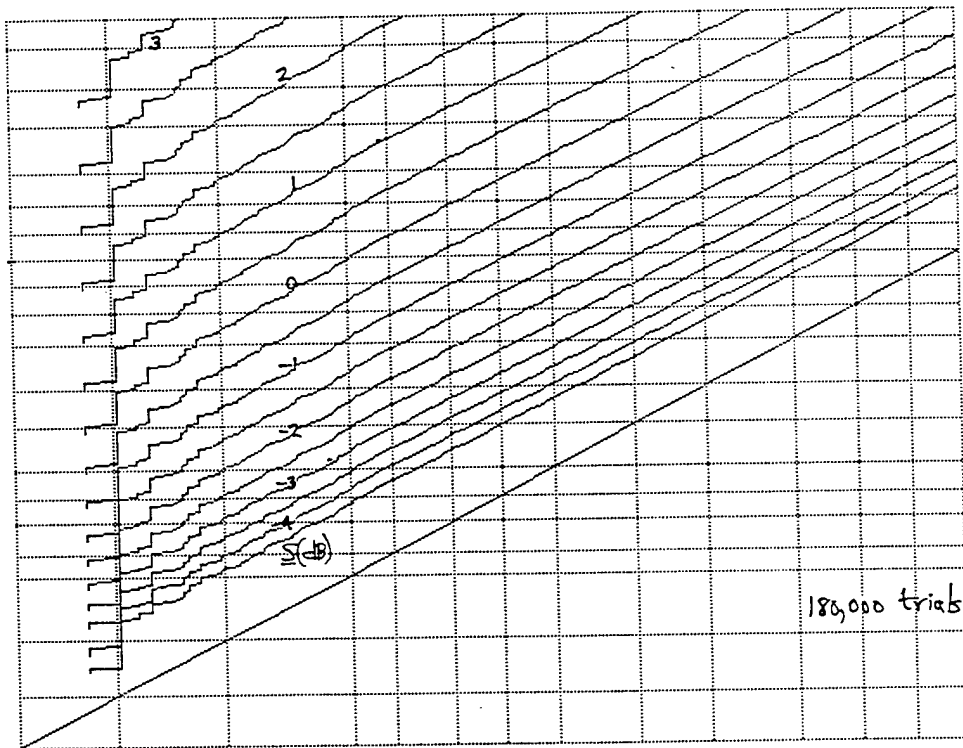
Figure F-11. ROC for M = 256 , v = 1.75 , \mu = 1.5 , N = 1024
