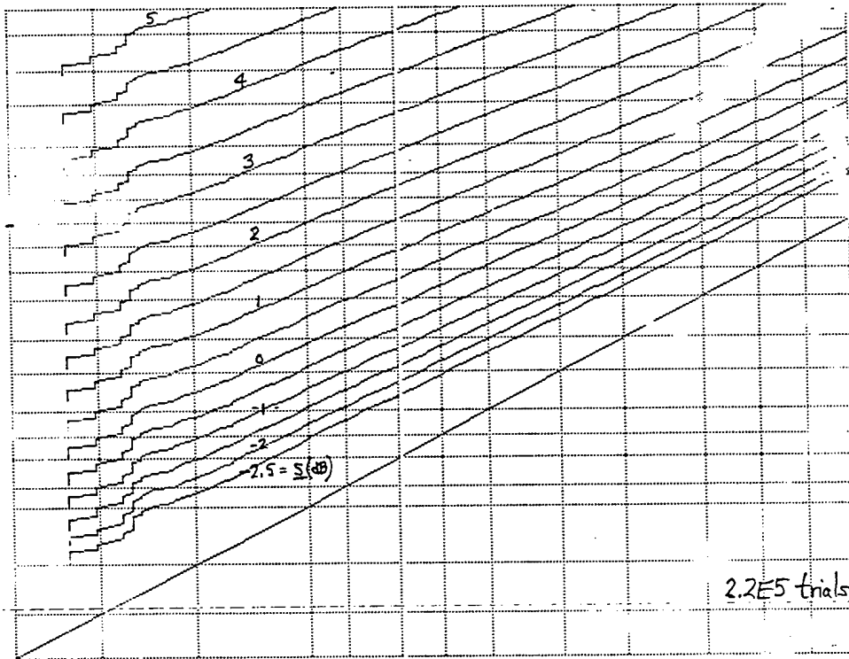
Figure D-19. ROC for M = 64 , v = 2 , \mu = 1 , N = 1024
