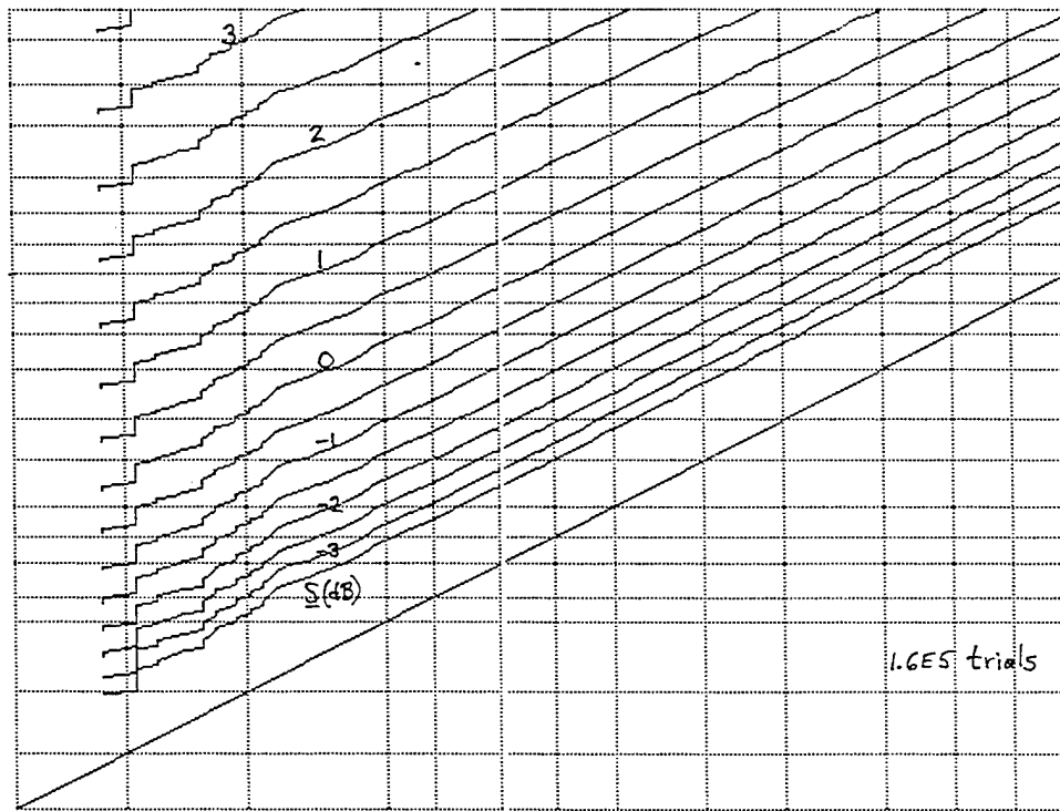
Figure F-26. ROC for M = 256 , v = 1 , \mu = 0.3 , N = 1024
