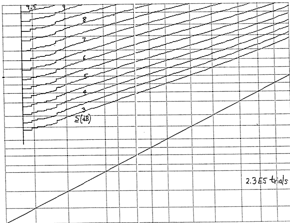
Figure D-12. ROC for \underline{M} = 16 , \nu = 3 , \mu = 1 , N = 1024
