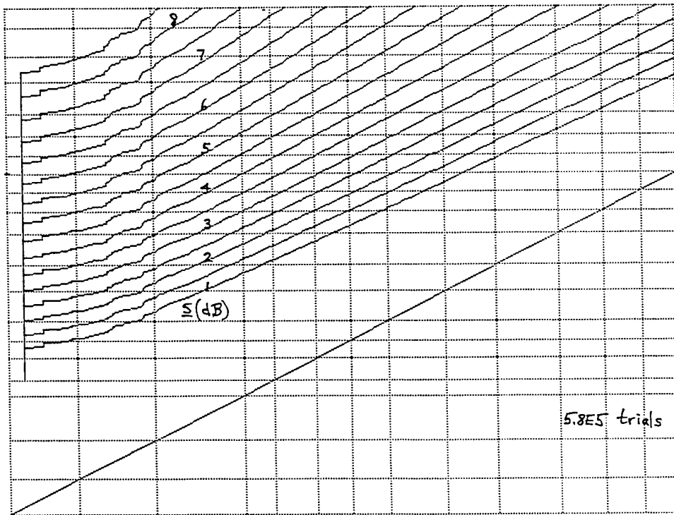
Figure D-16. ROC for M = 64 , v = \infty , \mu = 1 , N = 1024
