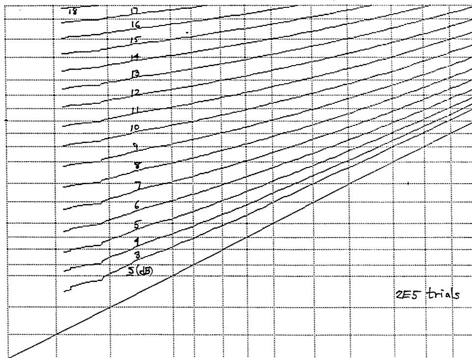
Figure D-10. ROC for \underline{M} = 4, v = 1, \mu = 1, N = 1024
