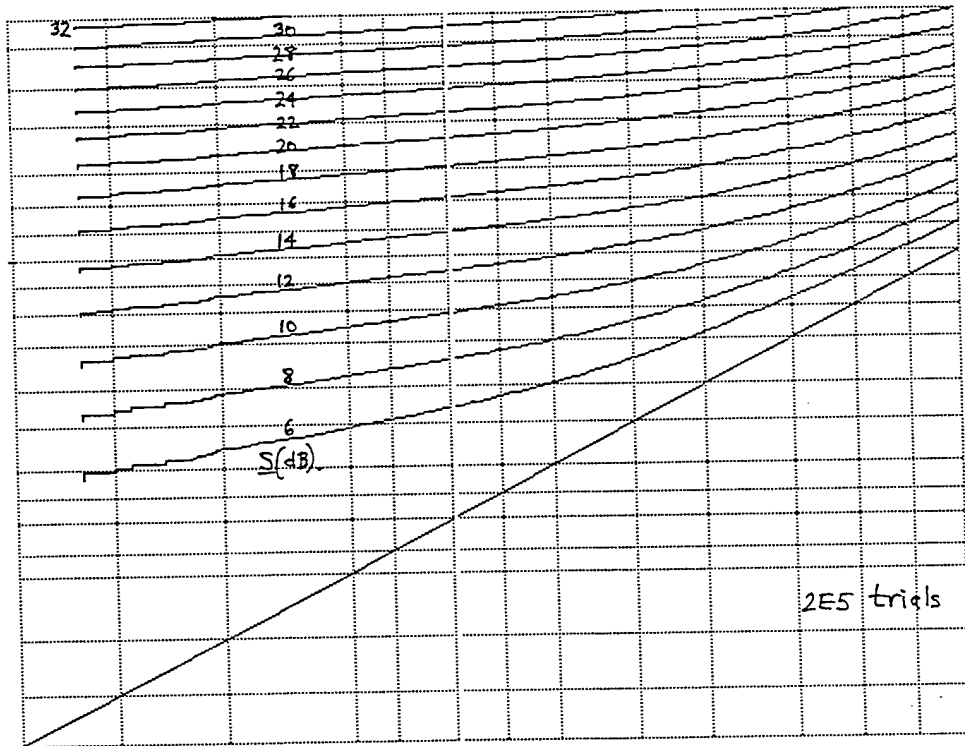
Figure D-3. ROC for \underline{M} = 1 , \nu = 2.5 , \mu = 1 , N = 1024
