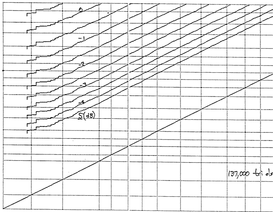
Figure G-2. ROC for M = 256 , v = 1.5 , \mu = 1 , N = 1024 , (17)
