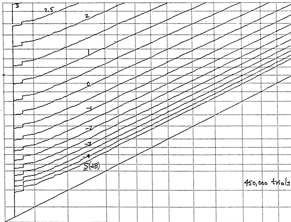
Figure F-14. ROC for M = 256 , v = 1.5 , \mu = 0.5 , N = 1024
