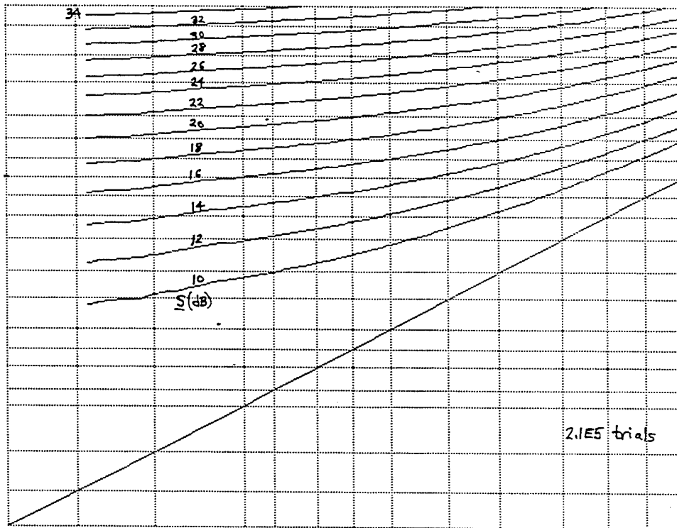
Figure D-5. ROC for \underline{M} = 1 , \nu = 1 , \mu = 1 , N = 1024
