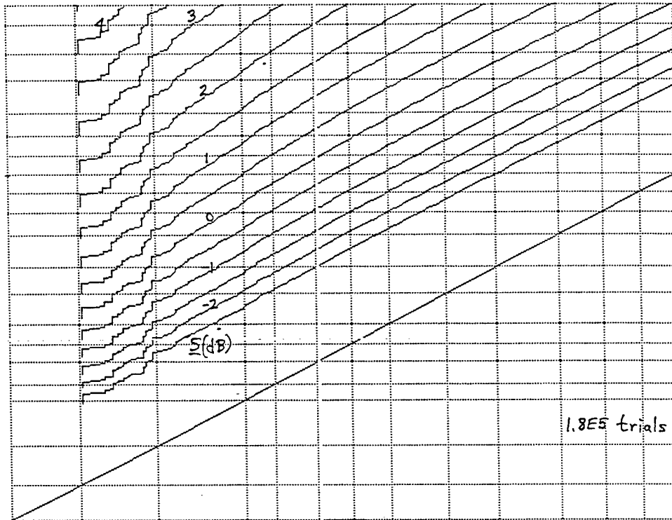
Figure F-25. ROC for M = 256 , v = 2 , \mu = 2 , N = 1024
