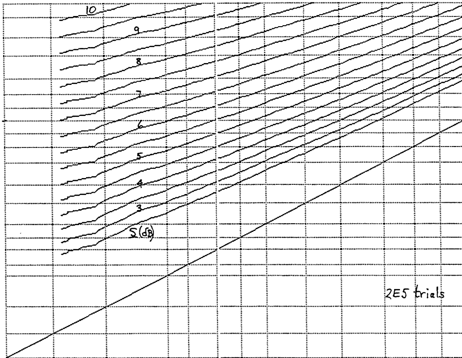
Figure D-15. ROC for M = 16 , v = 1 , \mu = 1 , N = 1024
