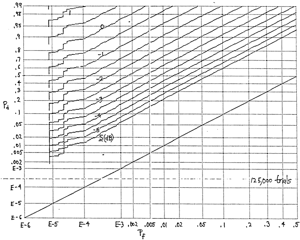
Figure G-1. ROC for M = 256 , v = 1 , \mu = 1 , N = 1024 , (17)
