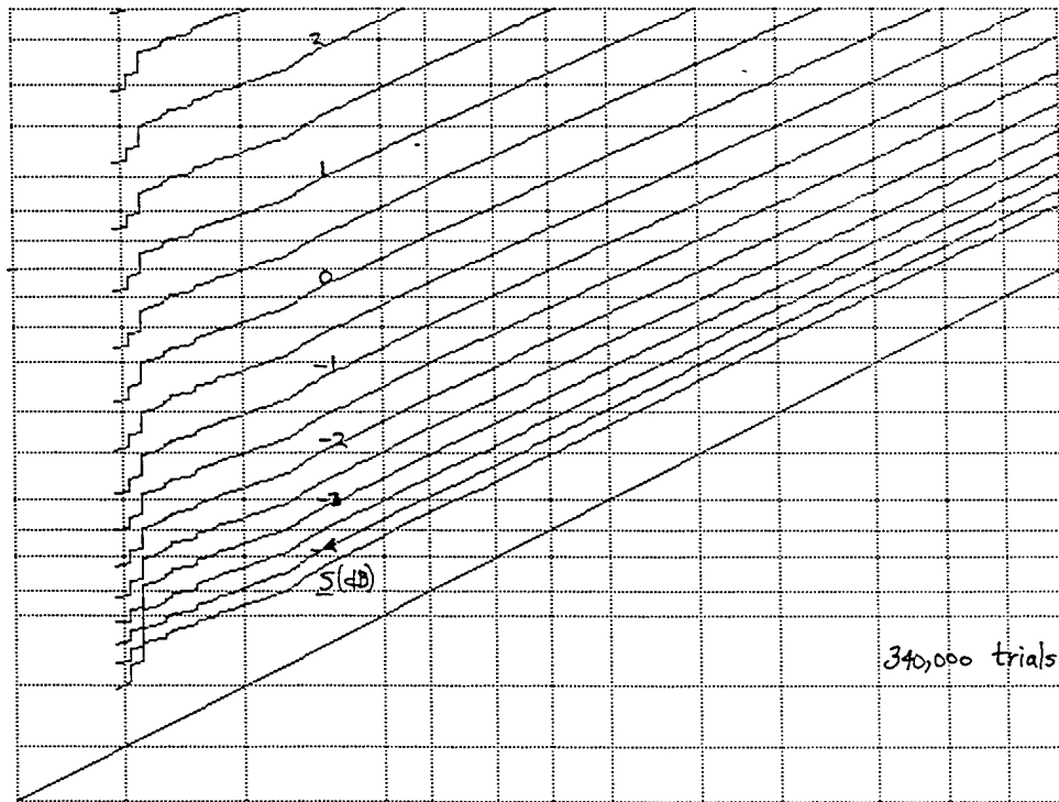
Figure F-2. ROC for M = 256 , \nu = 1.5 , \mu = 1.25 , N = 1024
