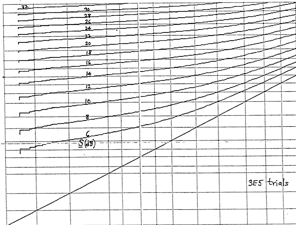
Figure D-4. ROC for \underline{M} = 1 , \nu = 2 , \mu = 1 , N = 1024
