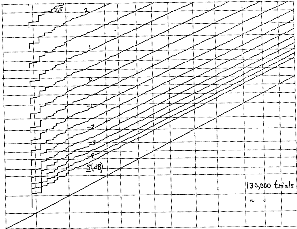
Figure F-3. ROC for M = 256 , \nu = 1.25 , \mu = 1.25 , N = 1024
