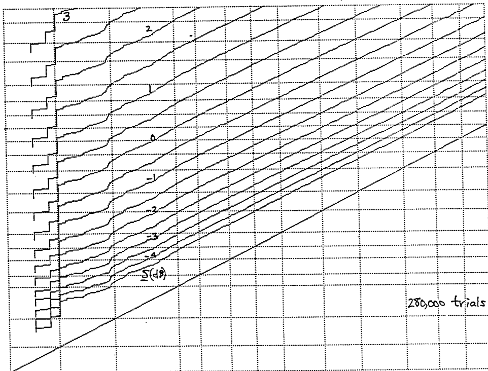
Figure F-12. ROC for M = 256 , v = 2.5 , \mu = 0.5 , N = 1024
