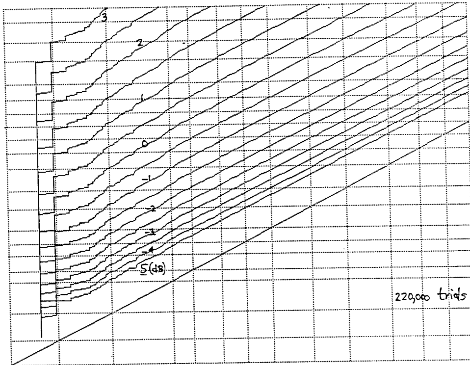
Figure F-15. ROC for M = 256 , v = 2 , \mu = 1.5 , N = 1024
