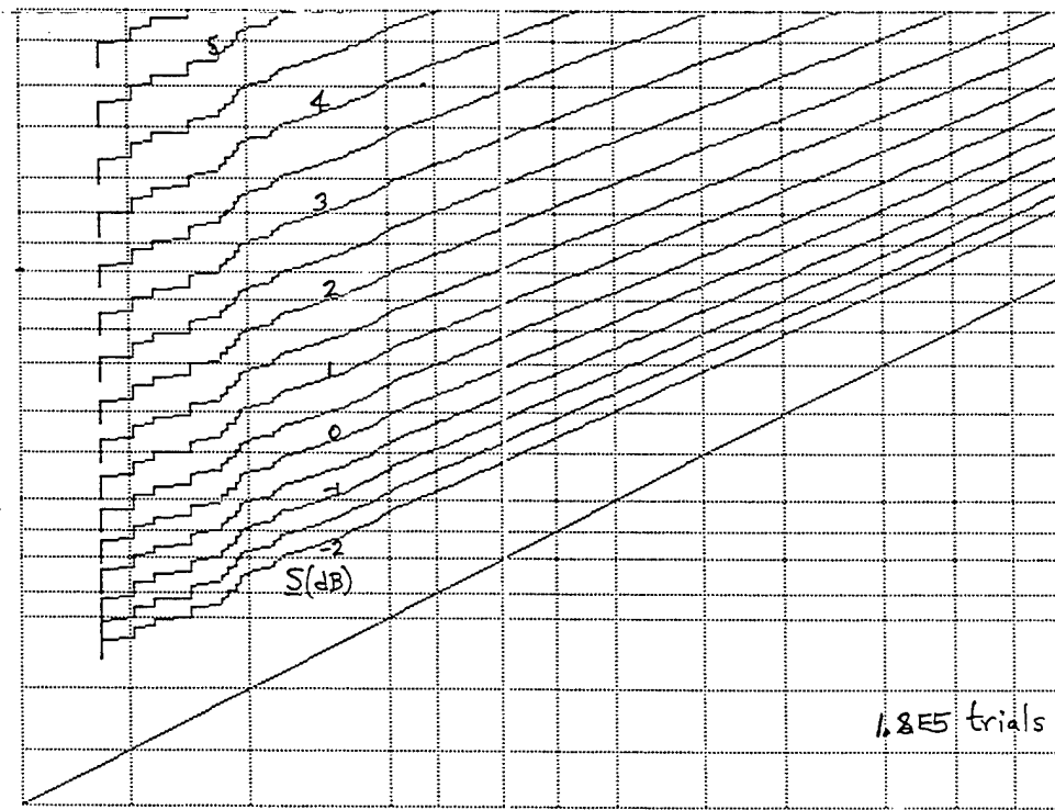
Figure D-18. ROC for M = 64 , v = 2.5 , \mu = 1 , N = 1024
