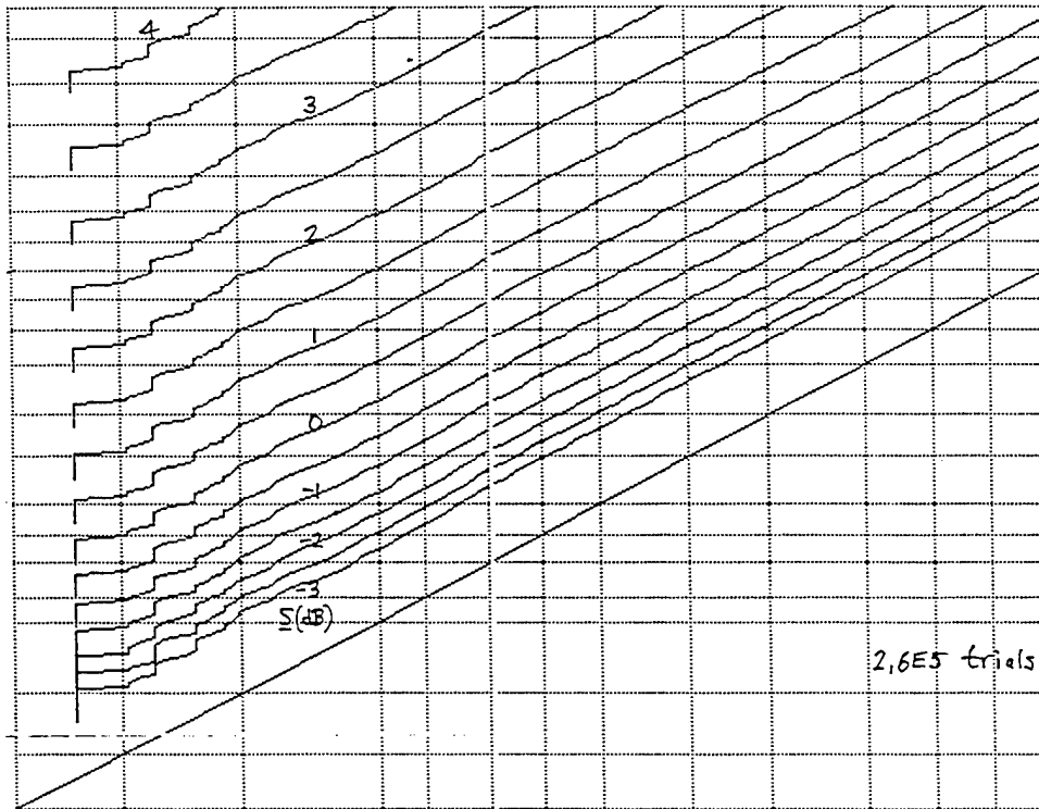
Figure F-29. ROC for M = 256 , v = 1 , \mu = 0 , N = 1024
