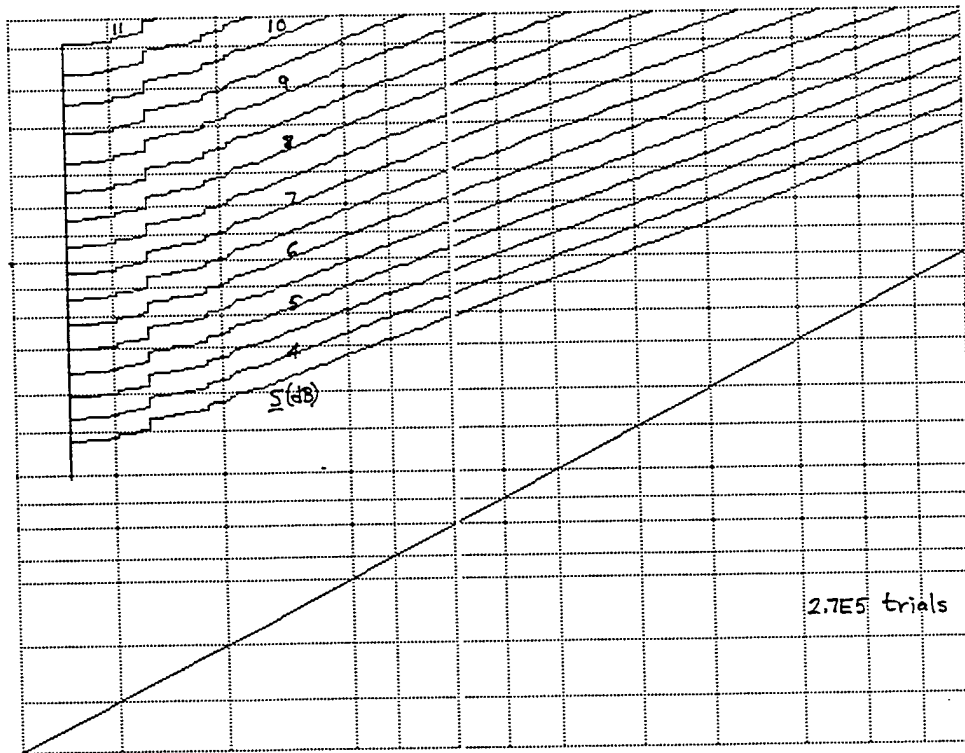
Figure D-11. ROC for \underline{M} = 16 , \nu = \infty , \mu = 1 , N = 1024
