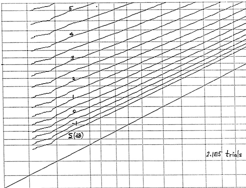
Figure D-20. ROC for M = 64 , v = 1 , \mu = 1 , N = 1024
