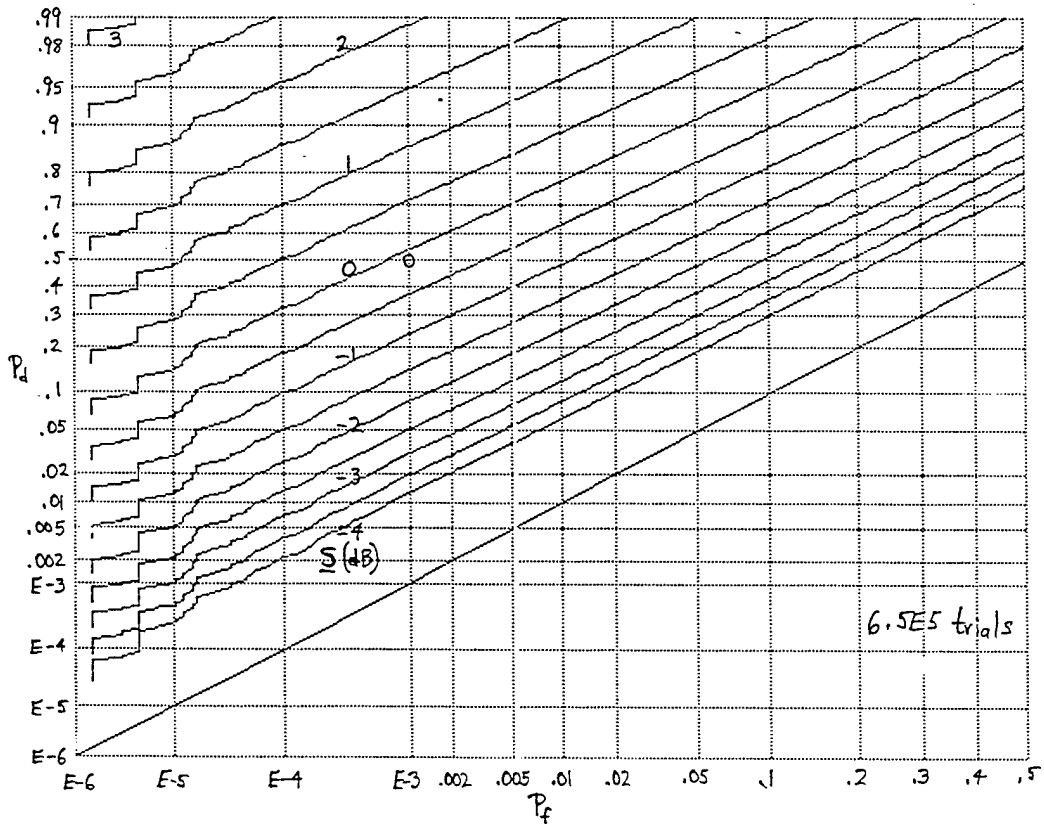
Figure F-1. ROC for M = 256 , \nu = 1.5 , \mu = 1 , N = 1024
