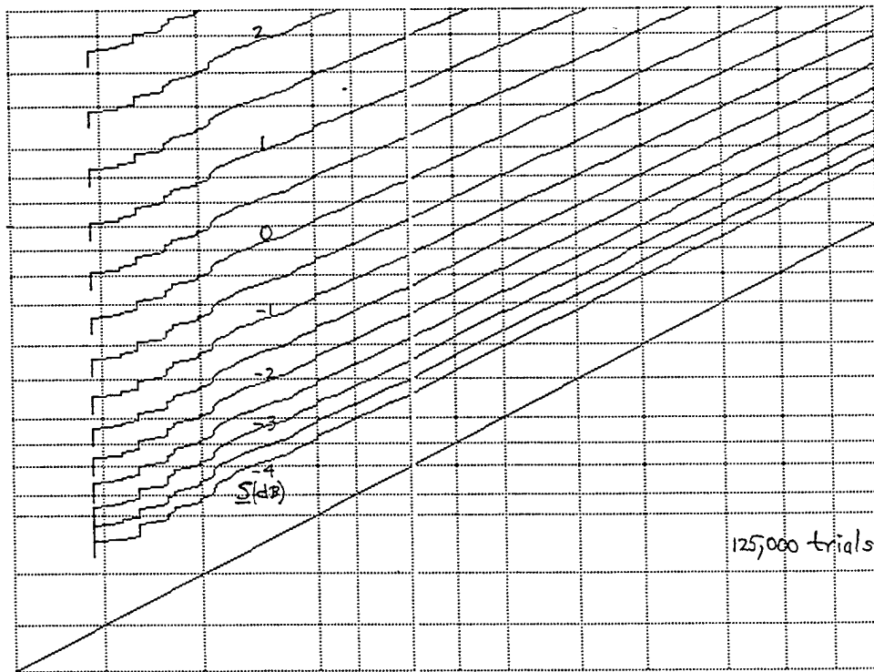
Figure F-4. ROC for M = 256 , \nu = 1.25 , \mu = 1 , N = 1024
