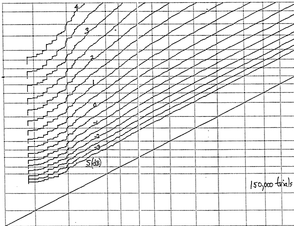
Figure F-28. ROC for \underline{M} = 256 , \nu = 3 , \mu = 1.5 , N = 1024
