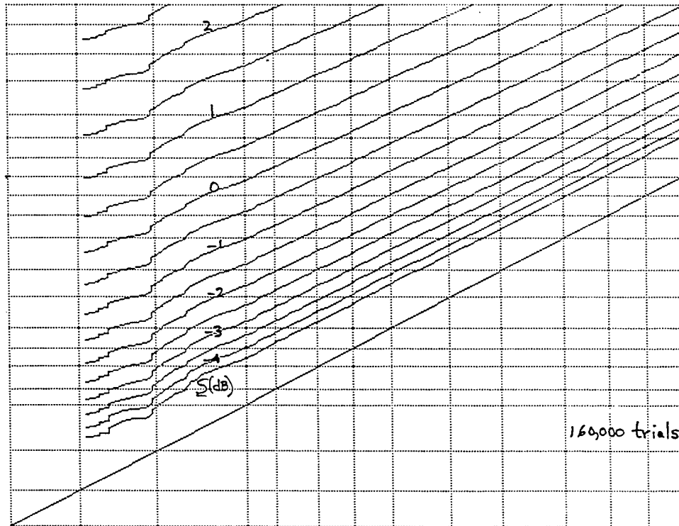
Figure F-13. ROC for M = 256 , v = 1 , \mu = 1 , N = 1024
