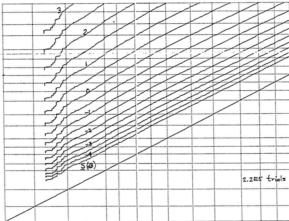
Figure F-20. ROC for M = 256 , \nu = 3 , \mu = 0.5 , N = 1024
