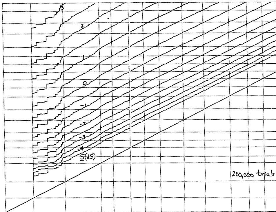
Figure F-16. ROC for M = 256 , v = 2.5 , \mu = 1 , N = 1024
