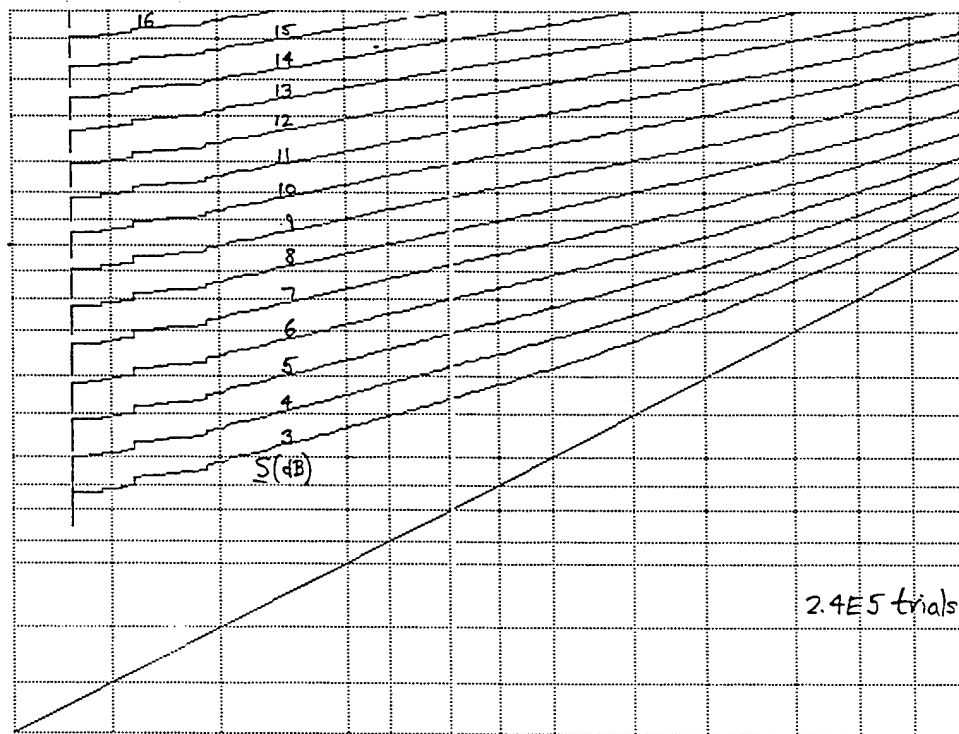
Figure D-6. ROC for \underline{M} = 4 , \nu = \infty , \mu = 1 , N = 1024
