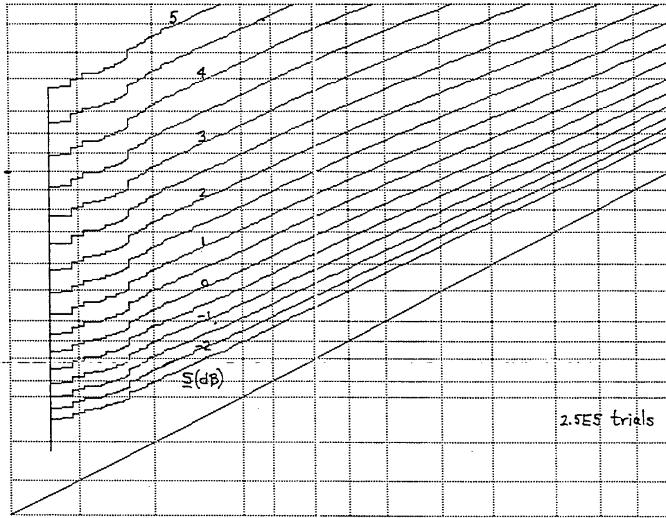
Figure D-17. ROC for M = 64 , v = 3 , \mu = 1 , N = 1024
