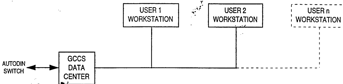
Figure 4.2. AMHS Functional Block Diagram
