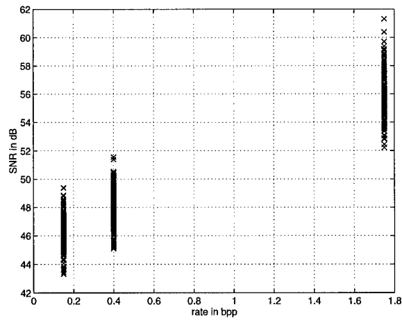
Figure 2: Scatter plot of SNR.
