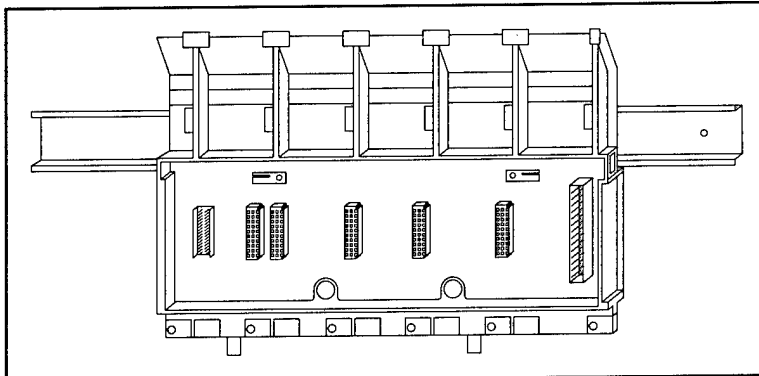
Figure 6. PLC backplate.
