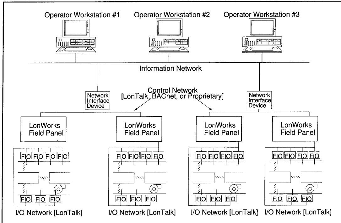
Figure 12. Utility controls with LonTalk.
