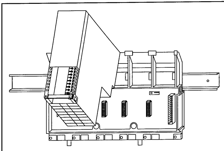
Figure 7. Module insertion.
