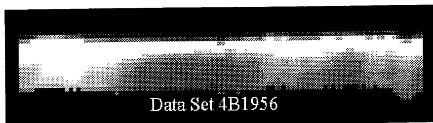
Figure 3.4. Monochromatic images in O_2 (0,0) from STS-69, MET day 4. The last four digits in each label give the MET times in hours and minutes.
