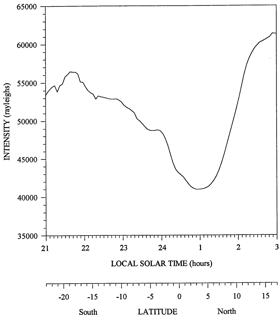
Figure 3.12. Intensity of the O_2(0,0) emission averaged over orbits 71 through 99 as a function of local solar time. Note the pronounced intensity minimum near 1.0 LST, a few degrees north of the equator.
