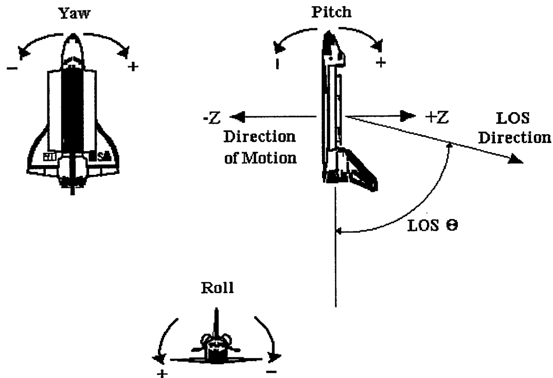
Figure 2.6. Shuttle pitch, roll, and yaw axes.
