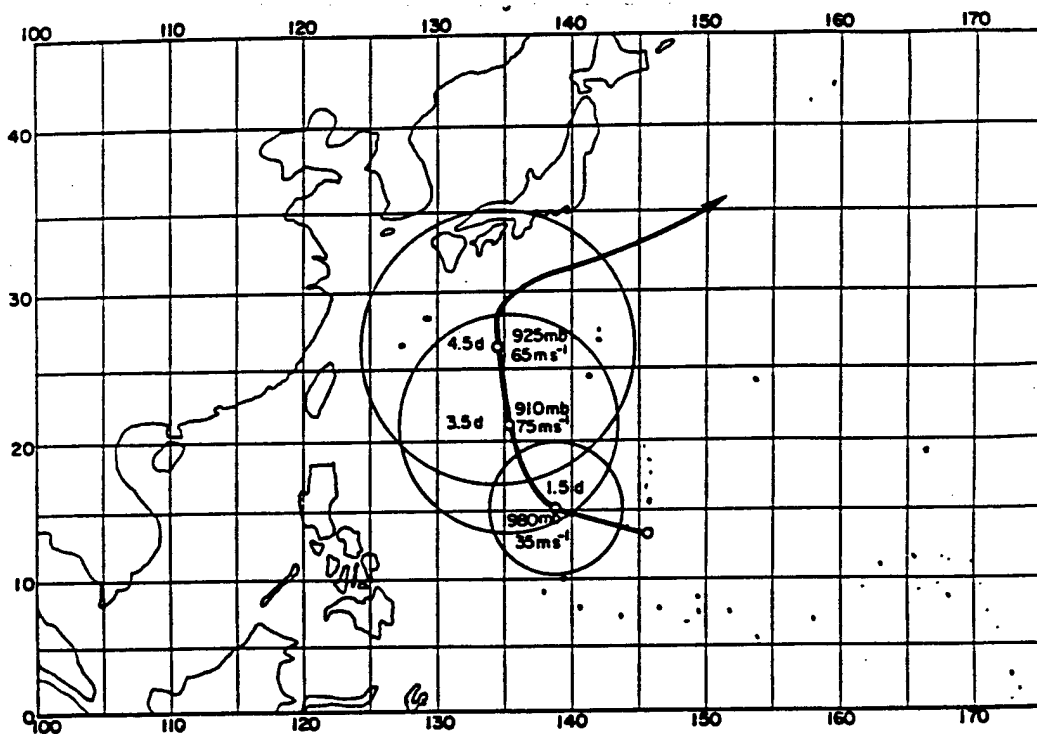
Figure 1.1: (b) Same as Fig. 1.1a except for six October supertyphoons (from Merrill 1982).
