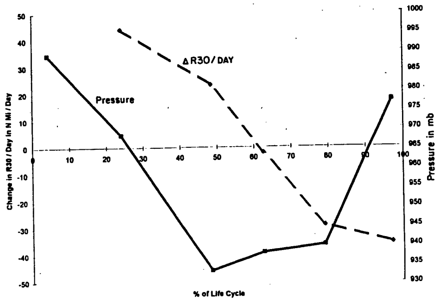
Figure 6.1: The change in R30 in \text{nmid}^{-1} and central pressure (mb) versus cyclone life cycle for simultaneous cyclones.
