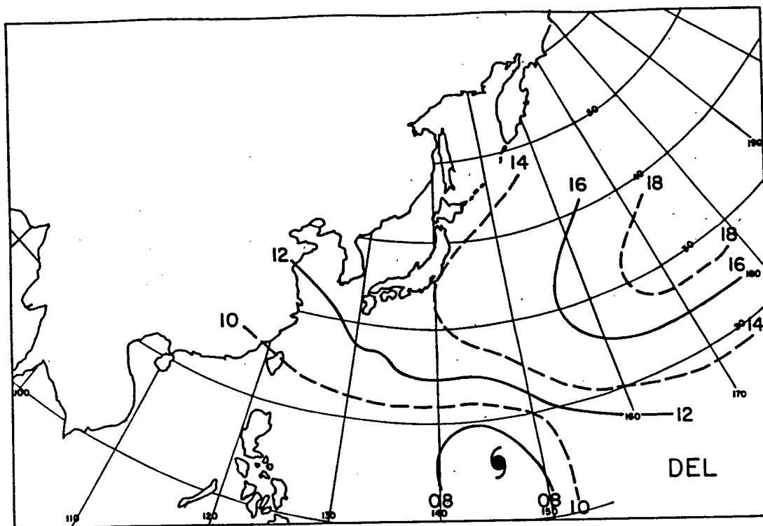
Figure 4.16: Surface synoptic pressure pattern for delayed cyclones two days prior to maximum intensity (MI).
