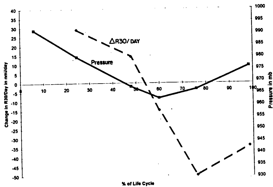
Figure 6.2: Same as Fig. 6.1 except for gyre cyclones.
