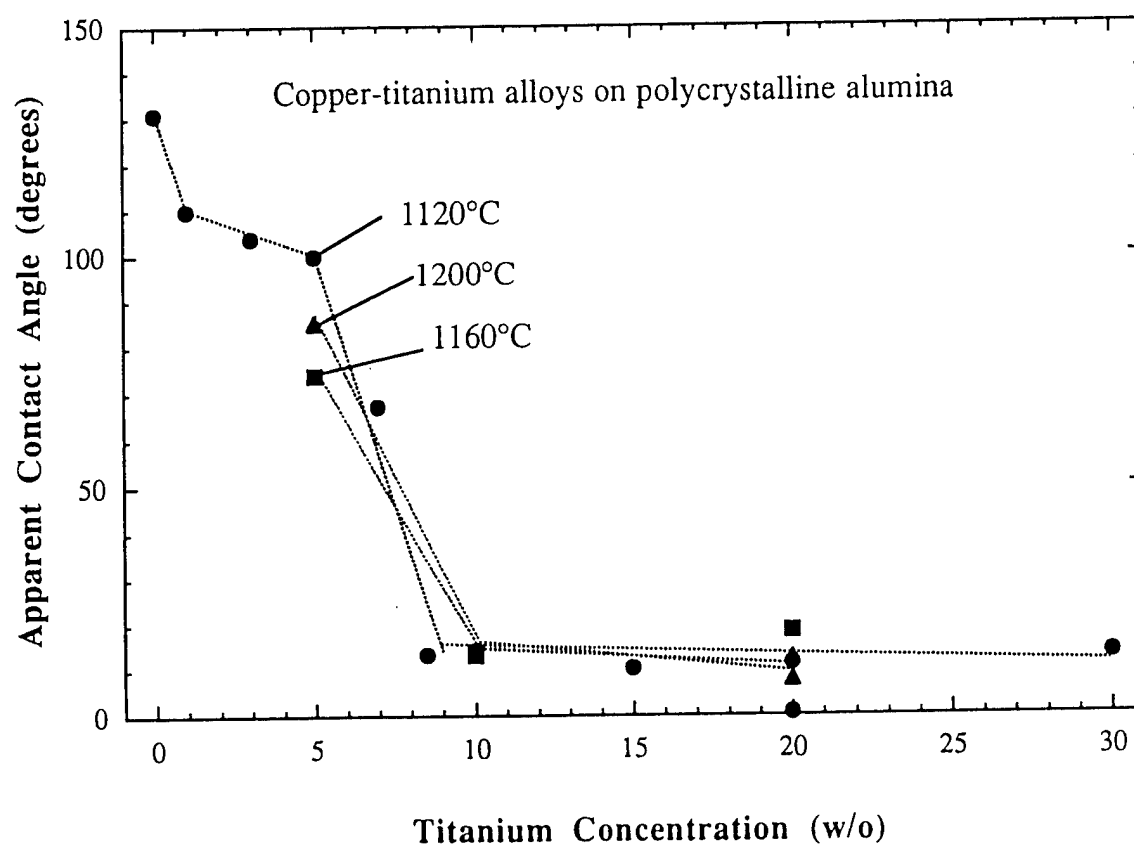
Figure 15: The apparent equilibrium contact angle ( q ) versus titanium concentration for copper-titanium alloys on alumina.
