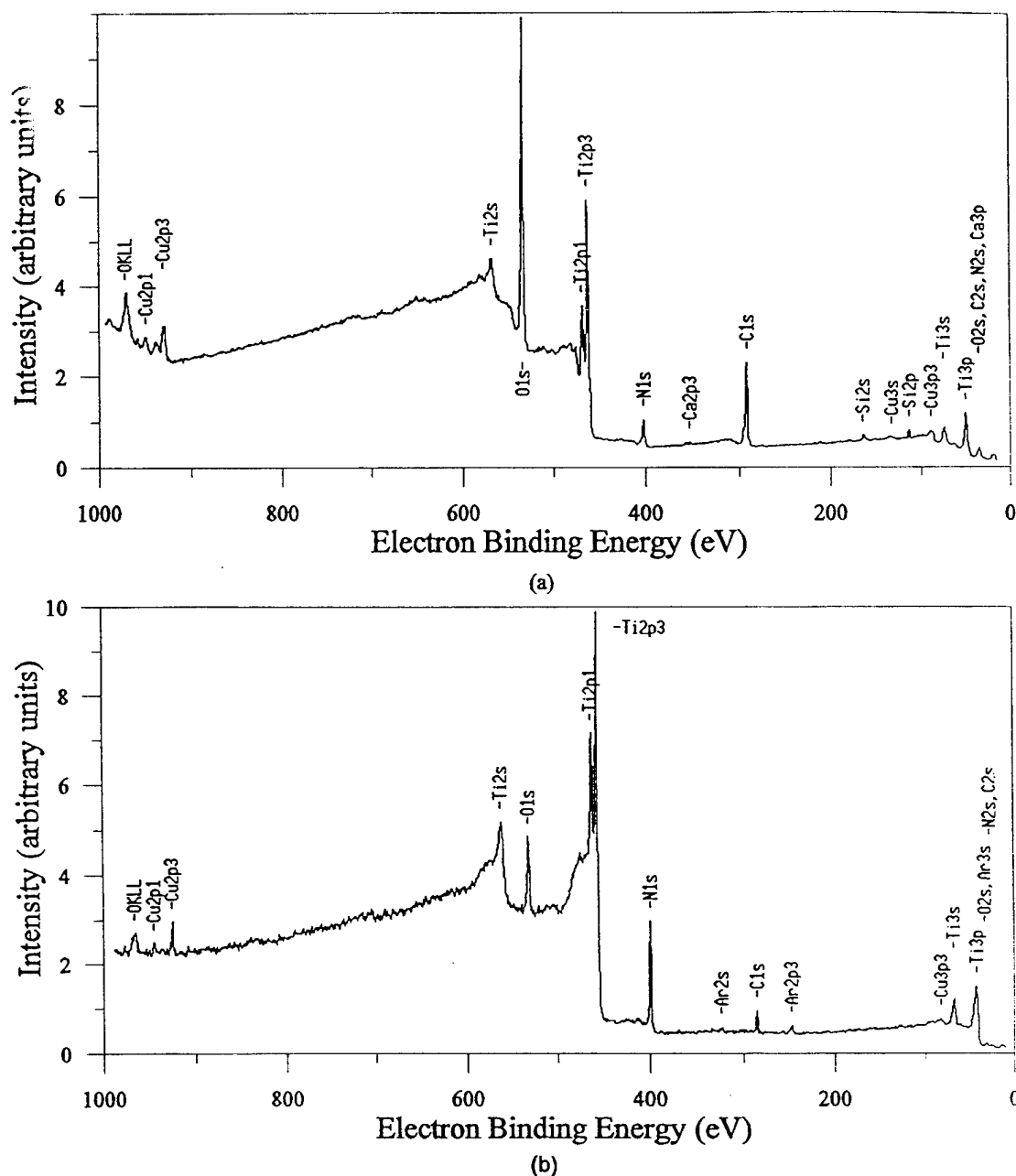
Figure 8: Overall photoemission spectra, corresponding to the metal side interfacial region of the Cu-Ti alloy/gas interface displayed in Figure 7. Processing conditions: Cu-Ti 4 at. %, no nitrogen control, oxygen partial pressure = 10^{-27} atm., 1150°C; 15 min., oxygen bulk concentration = 860 ppm; (a) as received, (b) after 3 min. sputtering.
