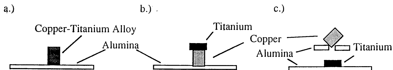
Figure 6: Initial room temperature sample configurations for sessile drop experiments(copper-titanium alloys on alumina), a.) pre-alloyed copper-titanium on alumina, b.) stacked titanium on copper on alumina, and c.) titanium on alumina with copper suspended above titanium.
