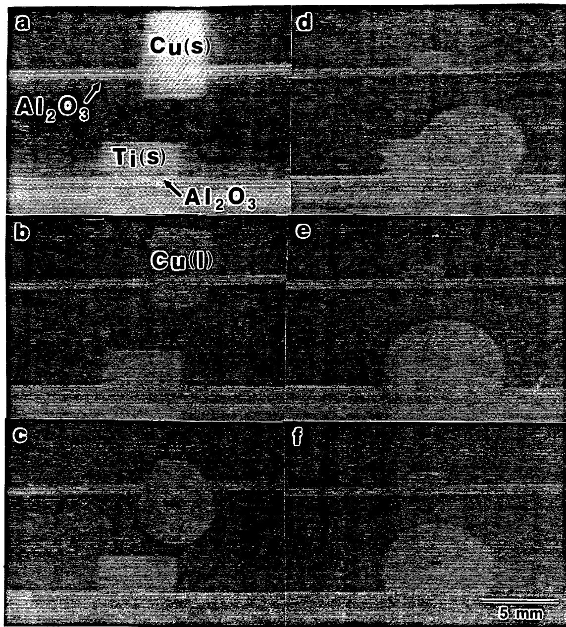
Figure 52: Formation of copper-20 w/o titanium alloy using the improved sessile drop configuration: a.) initial configuration, b.) copper melts ( \approx 1100^\circ\text{C} ), c.) liquid copper creeps through gap between plates, d.) copper falls onto Ti ( 1200^\circ\text{C} ), e.) Cu dissolves Ti ( \sim 8\text{s} after contact), and f.) dissolution is complete ( \sim 24\text{s} after contact).
