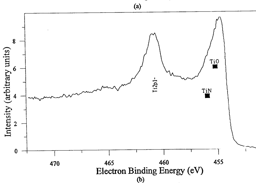
Figure 12: Titanium 2p3 photoemission spectra corresponding to the overall spectra displayed in Figure 11. Processing conditions: Cu-Ti 4 at. %, no nitrogen control, oxygen partial pressure = 10^{-27} atm., 1150°C; 15 min., oxygen bulk concentration = 860 ppm; (a) as received, (b) after 1 min. sputtering.
