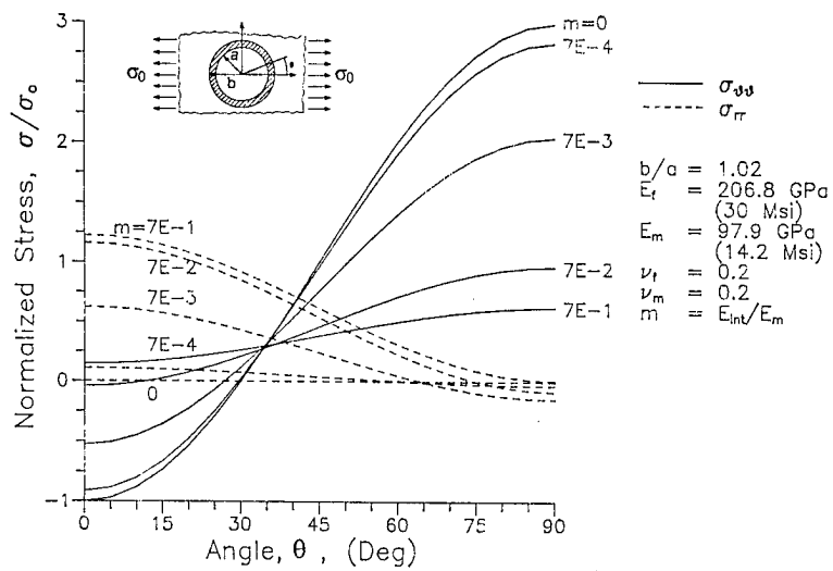
Stresses Around Inclusion with Interphase Liner in Infinite Elastic Medium. (Relative inclusion and matrix properties are those of the SiC/CAS material investigated)
