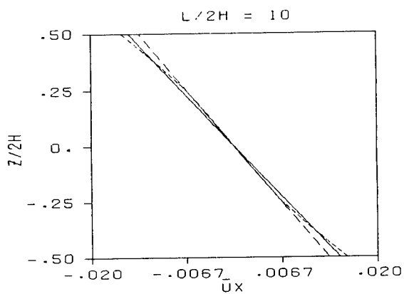
U_X DISTRIBUTION ACROSS THICKNESS
