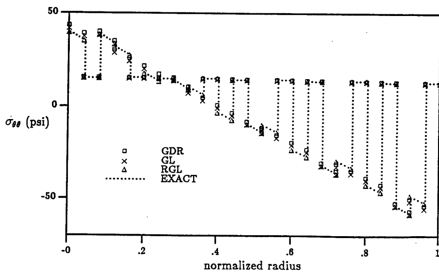
Hoop stress \sigma_{\theta\theta} in [75/15/90/-75/-15]_5 for \Delta T = -1^\circ\text{F}
