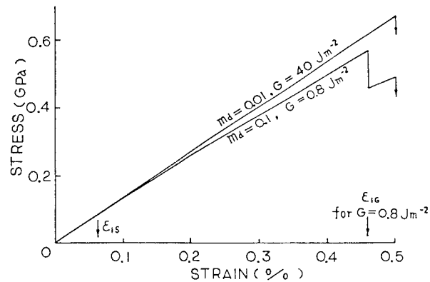
Fig. 8. Theoretical stress-strain curves. Union carbide P55S carbon fibres, with aspect ratios of 125, P_1 = 7 MPa, V_f = 0.4 , s_c = 90 .
