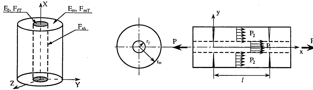
Geometry and Loading in Ceramic Composite
