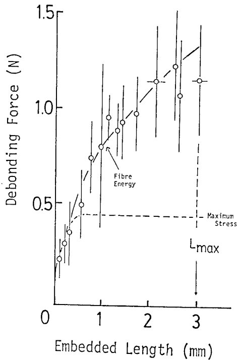
Fig. 3. Variation of debonding force, F_d , with fibre embedded in polyester resin. A curve going through points is F_d \propto L^{1/2} . Dashed line is estimated result for maximum shear stress at interface high enough to equal shear strength of the polyester resin.
