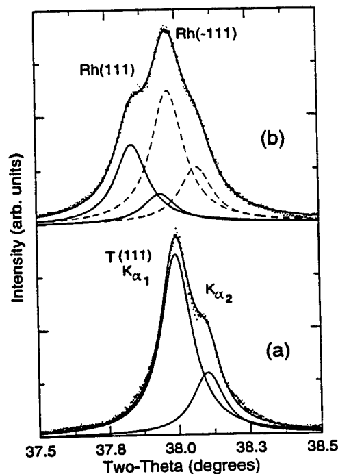
FIG. 4. Room temperature \theta-2\theta x-ray diffraction spectrum for PLSnZT ceramic sample at (a) E_{\text{appl}}=0 and (b) E_{\text{appl}}=E_{\text{AFE-FE}}=26 kV/cm showing the zero-field AFE line profile fit with a single tetragonal structure and the electric-field-induced FE spectrum fit to a single rhombohedral structure.
