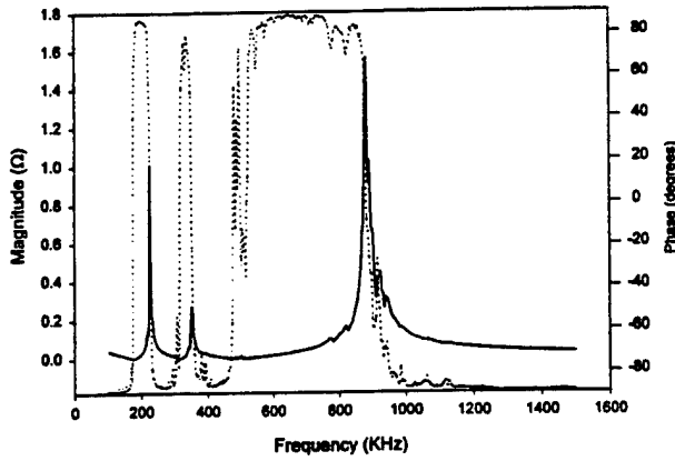
Fig 2. Impedance plot for a <001> poled and [100] aligned PZN 8% PT k_{\text{bar}} mode sample. The k_{\text{bar}} mode is the highest frequency mode present. The low frequency mode is k_{31} .
