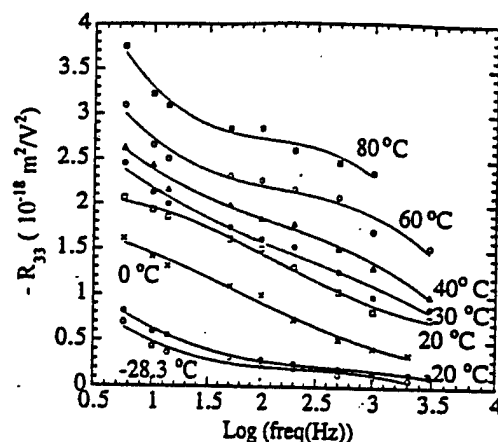
FIG. 7. R_{33} as a function of frequency at different temperatures (from top to bottom): 80 °C (solid squares), 60 °C (open circles), 40 °C (open triangles), 30 °C (solid circles), 20 °C (open squares), 0 °C (crosses), -20 °C (solid circles), and -28.3 °C (open circles). The solid lines are drawn to guide eyes.
