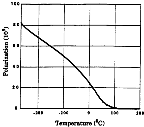
Fig.4. The temperature dependencies of the mean polarization of the PZT/STO superlattice with a total thickness of 0.573\mu\text{m} . a_n=a_{n+1}=10\text{nm} .
