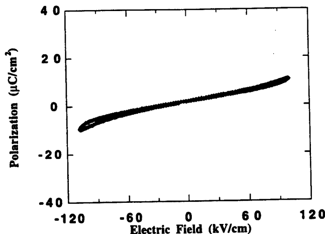
Fig. 4. Polarization vs electric field for composition C7.
