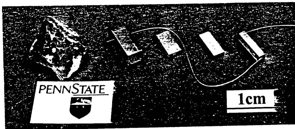
Figure 4. As grown crystal, an aligned sample using the Laue camera, a cut and polished sample, an electroded sample for direct strain observation as well as for low field planar mode resonant sample, and a low field longitudinal mode resonant sample, for PZN-9.5%PT, (from left to right).
