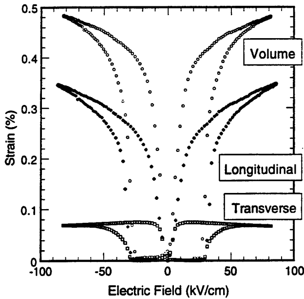
Fig. 2 Field-induced longitudinal, transverse, and volume strain for composition B1.
