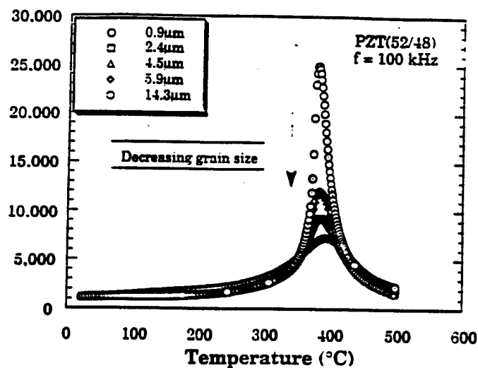
Fig. 6. Suppression of the maximum dielectric constant for PZT 52/48.
