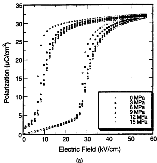
Fig. 5 (a) Polarization and (b) strain behaviors of composition B1 under various pre-stresses.
