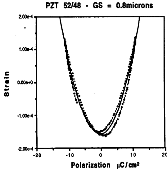
Fig.4 Strain vs. Polarization results for PZT 52/48, grain size = 0.8 microns.
