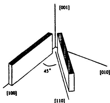
Fig 2. Resonant samples prepared. Axes are parallel to the \langle 001 \rangle family.
