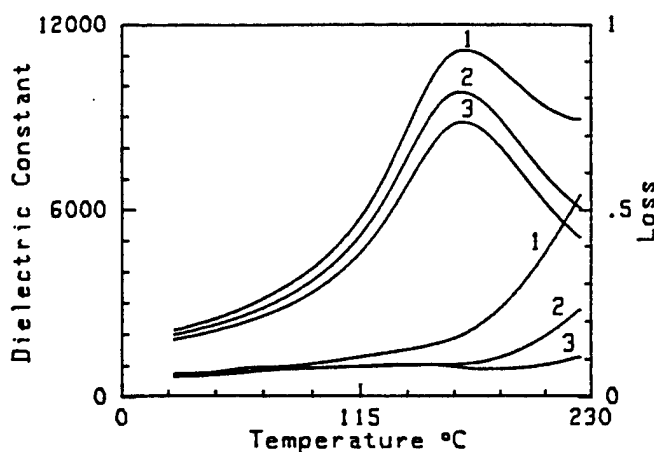
FIGURE 6 Dielectric constant and dielectric loss vs temperature for PZN ceramics processed at 20 Kbar, 2 hr: (1) 1 kHz; (2) 10 kHz; (3) 100 kHz.
