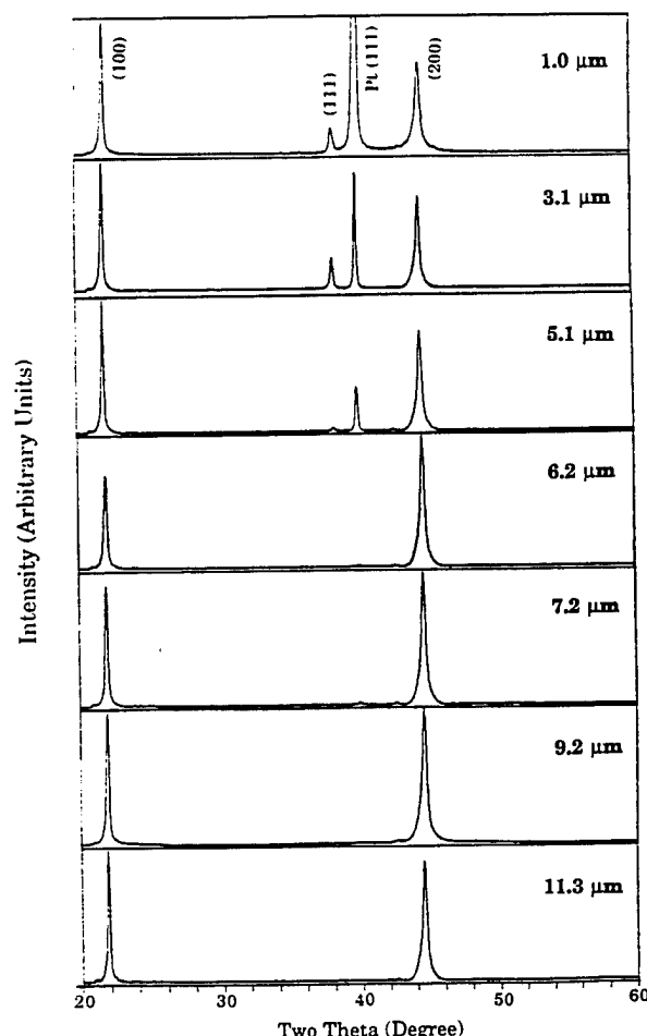
Fig. 1. Evolution of (100) planar orientation with thickness as evidenced by X-ray diffraction patterns of films of increasing thickness.
