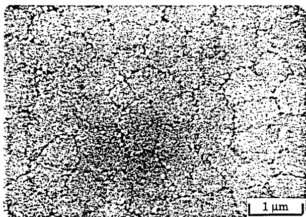
Fig. 2. SEM micrographs of surface and cross-sectional morphologies of a 11.3- \mu\text{m} -thick PZT film.
