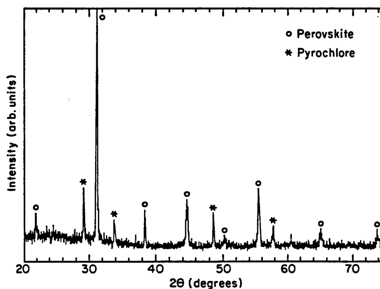
FIGURE 1 X-ray powder diffraction pattern of PZN-BT ceramics processed at 800°C, 35 Kbar.
