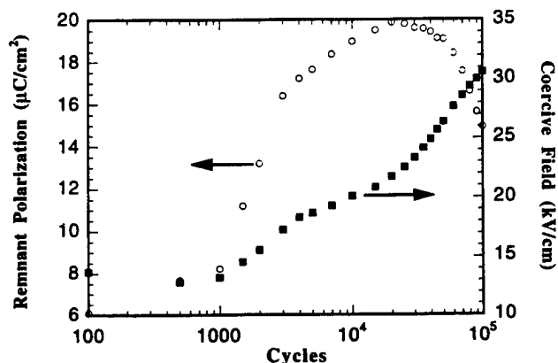
Fig. 4. Remnant polarization and coercive field during the gas evolution.
