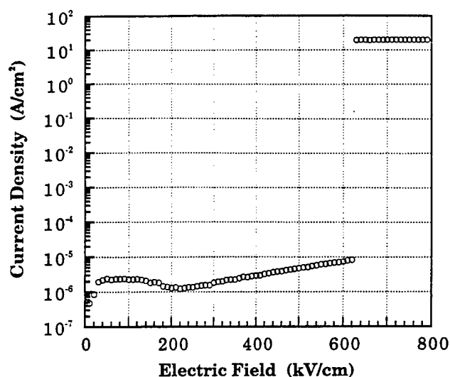
Fig. 9. I - V plot of a 8.2- \mu\text{m} -thick film to determine the dielectric breakdown strength of the film.
