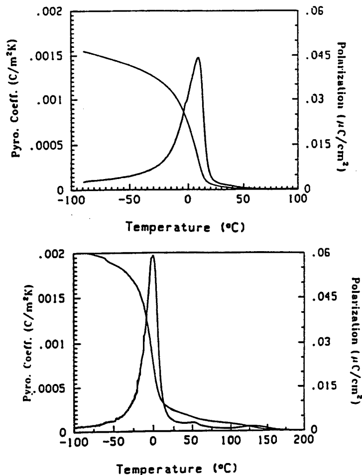
FIGURE 10 Pyroelectric constant and remnant polarization of (a) PIN:PST (97.5) and (b) PIN:PST (2.5).
