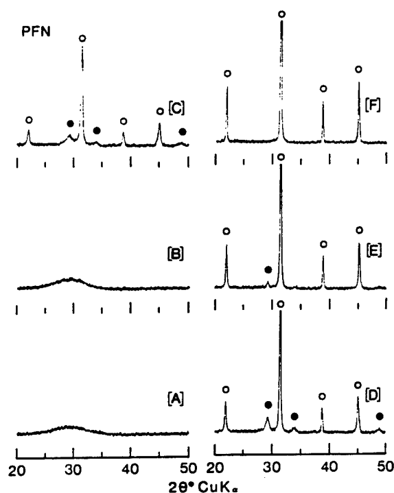
Fig. 6. XRD patterns of calcined PFN powder: (A) as-dried, (B) 400°, (C) 500°, (D) 600°, (E) 700°, and (F) 800°C ((○) perovskite and (●) pyrochlore).
