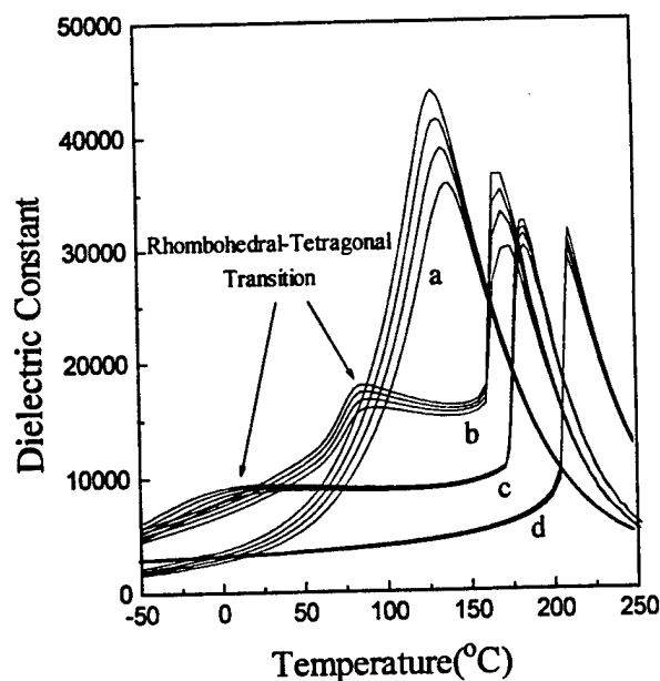
Figure 2 K vs. T curves for (001) oriented crystals for (a) PZN, (b) PZN-8%PT, (c) PZN-9.5%PT, and (d) PZN-15% PT
