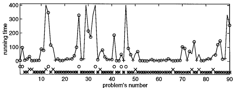
Figure 8: Selection of a method in the extended transportation domain: the running times (solid line), successes (o) and failures (+), and the selection made among APPLY (o), DELAY (x), and ALPINE (*).
