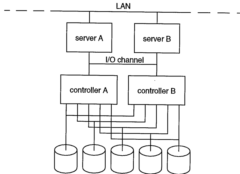
Figure 2-14 Disk array with redundant controllers
