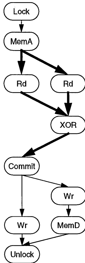
Figure 5-7(a): Step 4: eliminate a redundant arc
