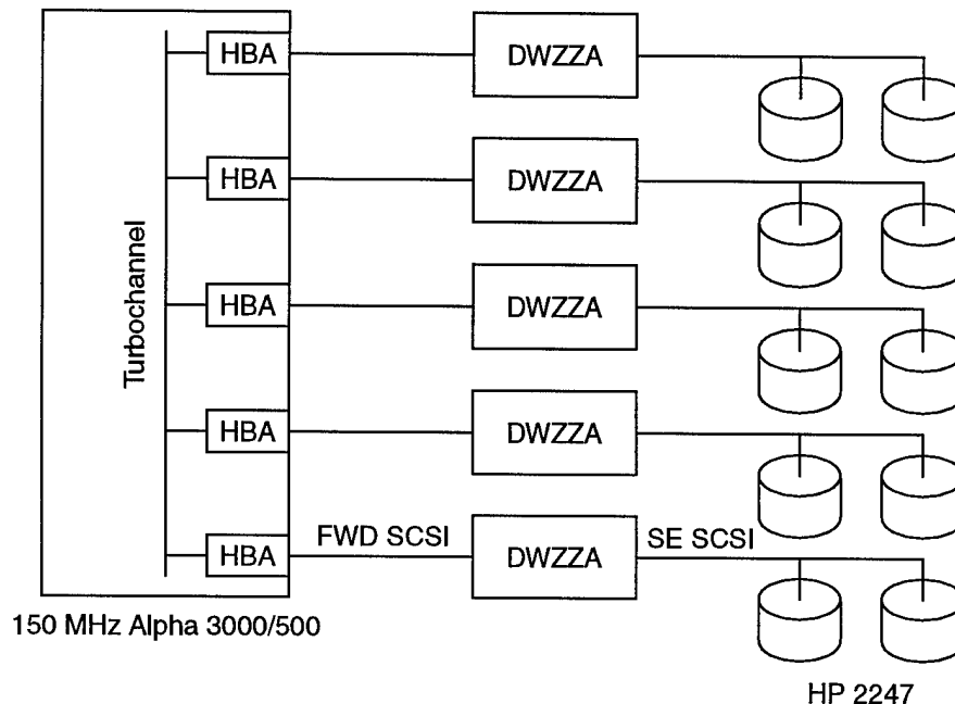
Figure 4-3 Setup used for collecting performance data
