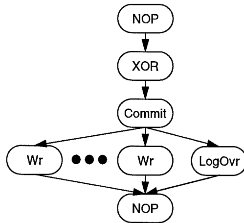
Figure B-9 Parity-logging large-write graph
