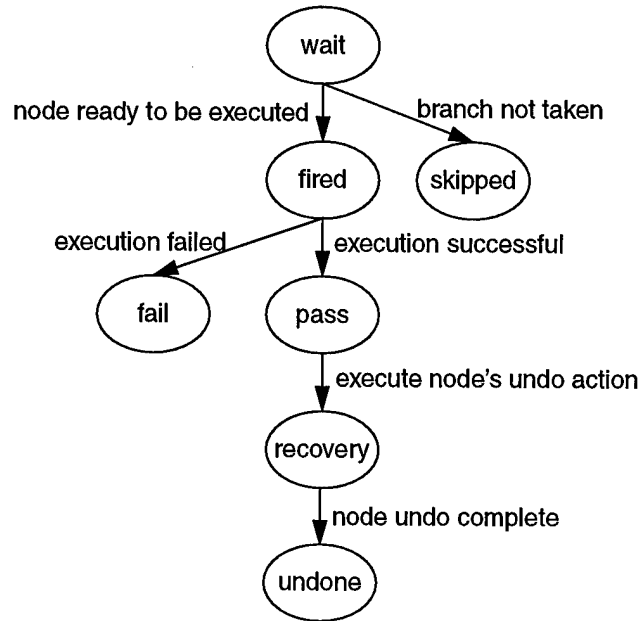
Figure 3-9 Node state transitions
