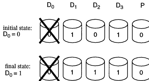
Figure 2-15 The write hole
