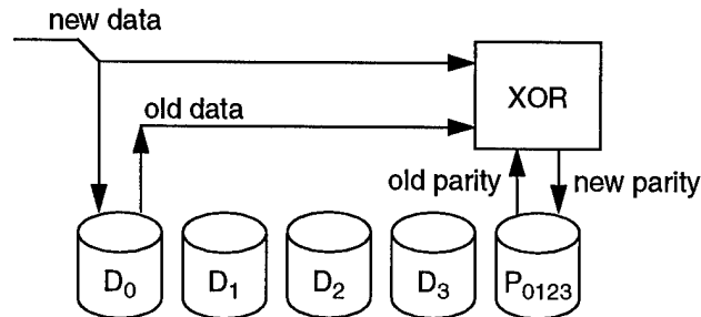
Figure 2-9 The small-write algorithm
