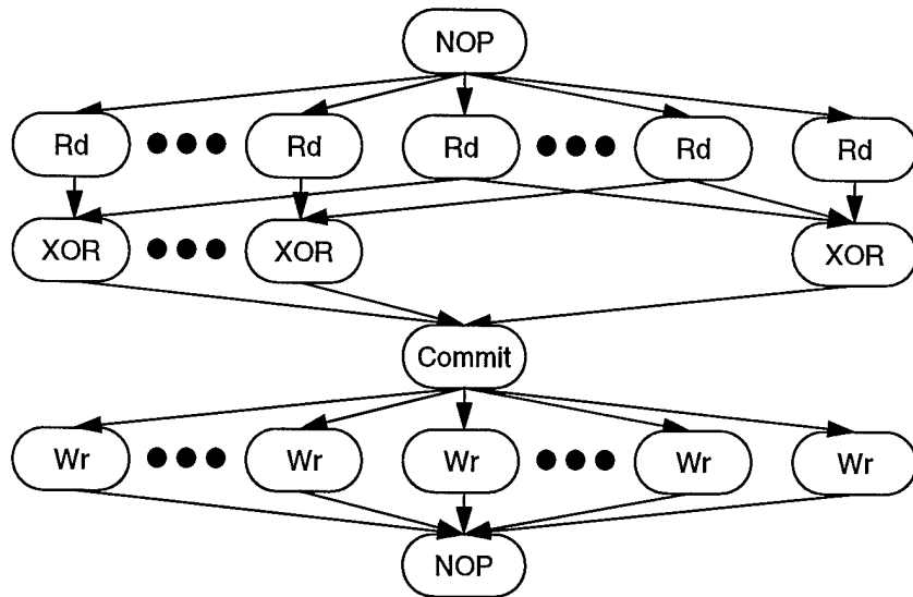
Figure B-21 2D degraded-DV write graph
