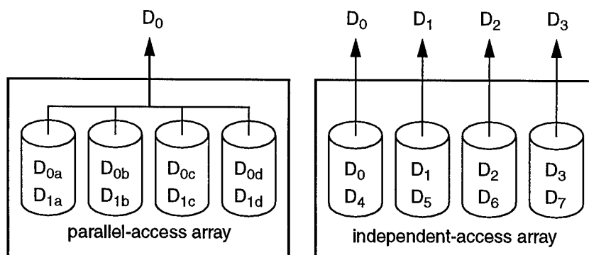
Figure 2-5 Data layouts which enable concurrency in disk storage
