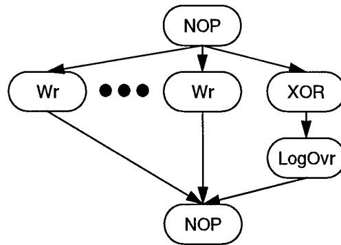
Figure A-9 Parity-logging large-write graph
