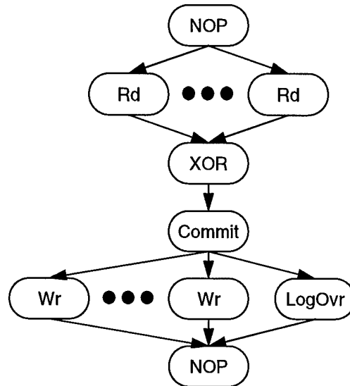
Figure B-8 Parity-logging reconstruct-write graph
