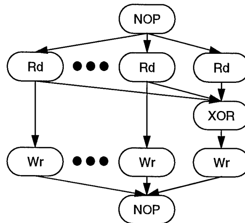
Figure A-5 Small-write graph
