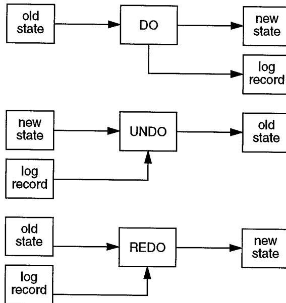
Figure 2-2 The DO-UNDO-REDO protocol
