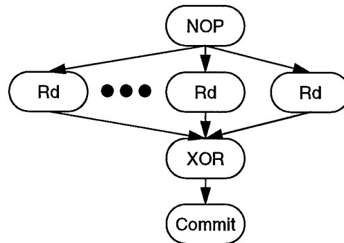
Figure B-4 Degraded-read graph
