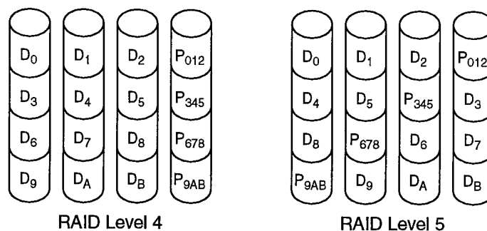
Figure 2-13 Parity placement in RAID levels 4 and 5
