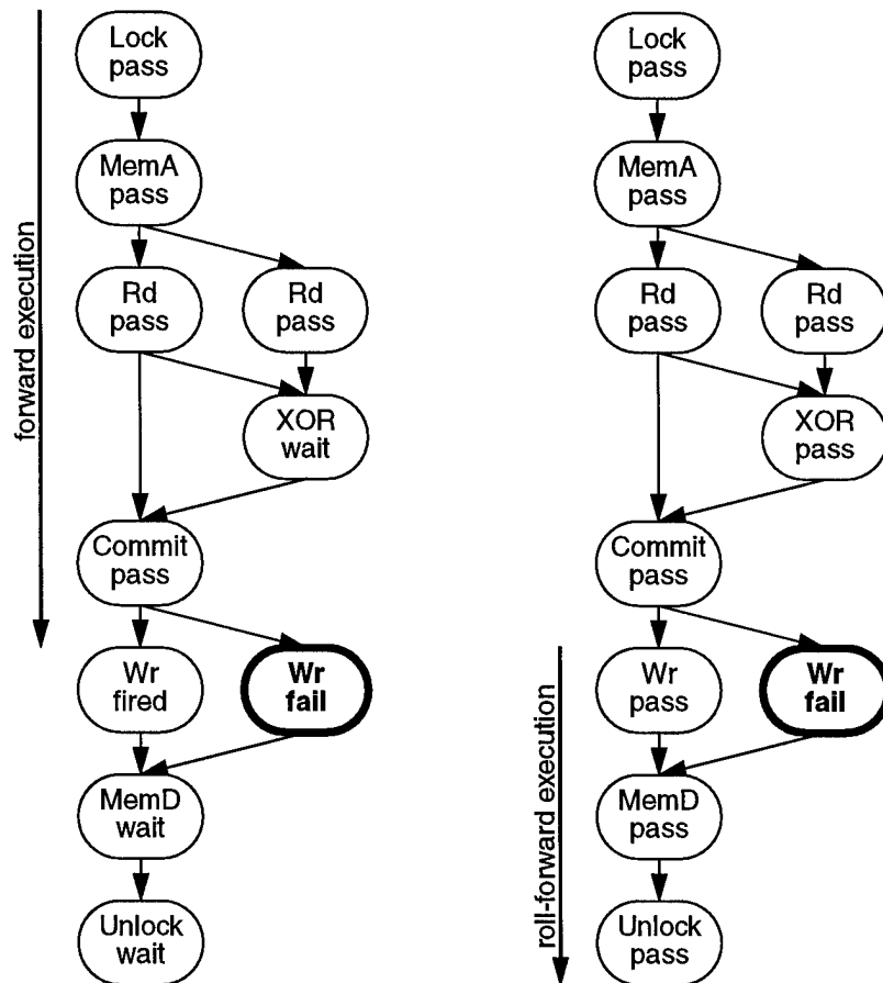
Figure 5-9 Recovering from errors following the commit point
