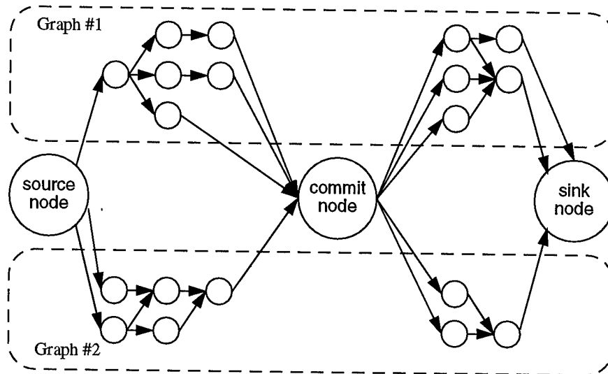
Figure 6-1 Synchronized commit coordinates recovery of multi-graph requests
