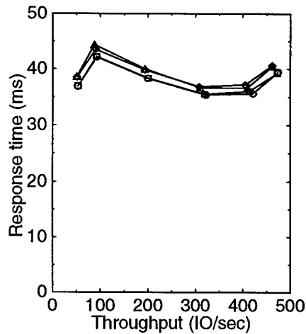
Figure 4-5(a): Constant workload/disk
