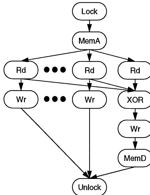
Figure 3-3 RAID level 4/5 small-write graph
