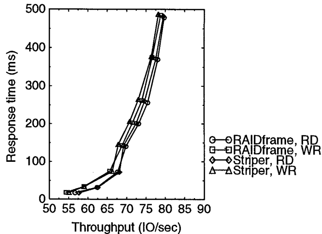
Figure 4-4 Single disk performance of striper and RAIDframe
