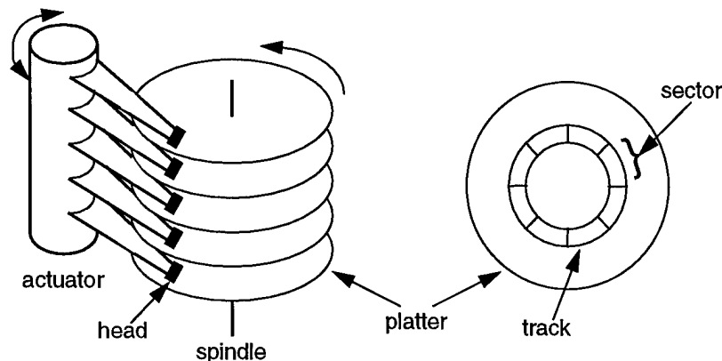
Figure 2-3 Accessing a sector
