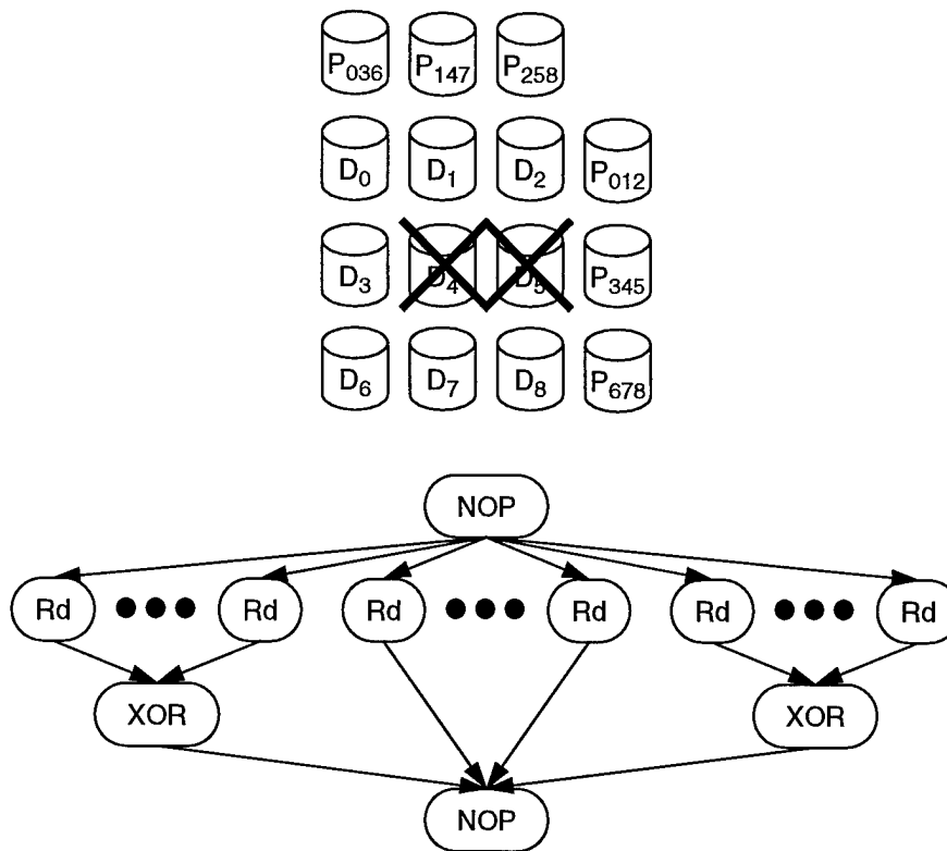
Figure A-16 2D double-degraded read graph
