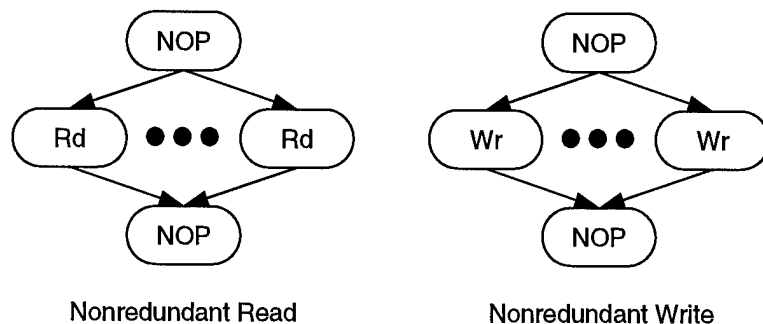
Figure A-1 Nonredundant graphs
