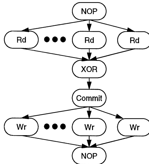
Figure B-5 Small-write graph
