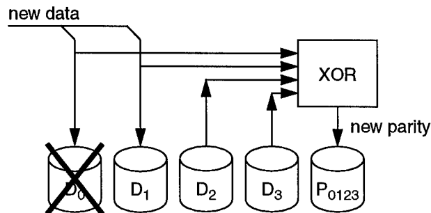
Figure 2-11 The degraded-write algorithm
