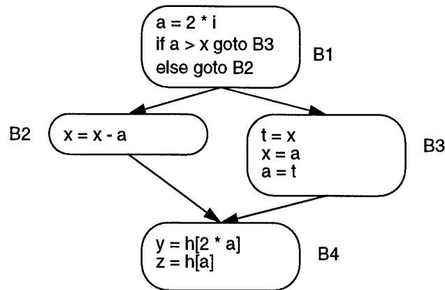
Figure 3-2 Flow graphs model program control flow
