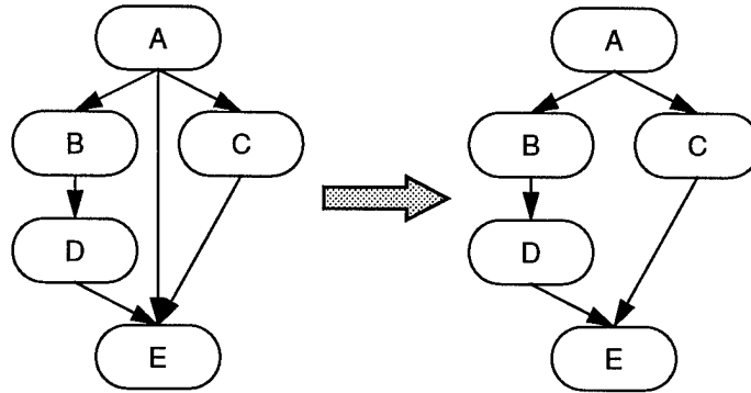
Figure 3-4 Eliminating redundant arcs
