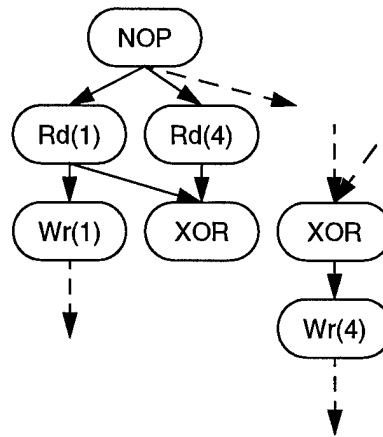
Figure 3-5(b): Common Subexpression Removed
