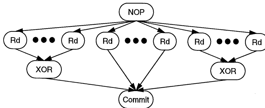
Figure B-16 2D double-degraded read graph
