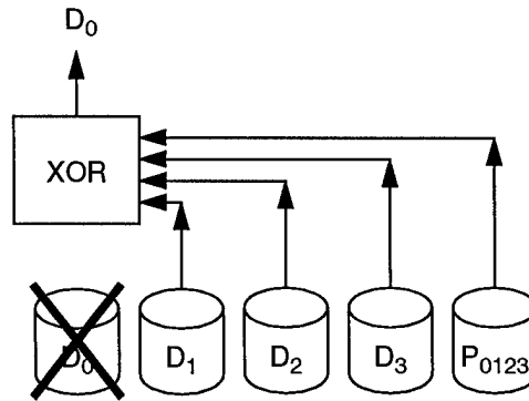
Figure 2-12 The degraded-read algorithm
