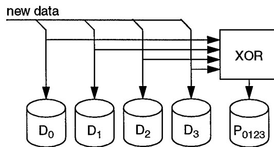
Figure 2-8 The large-write algorithm
