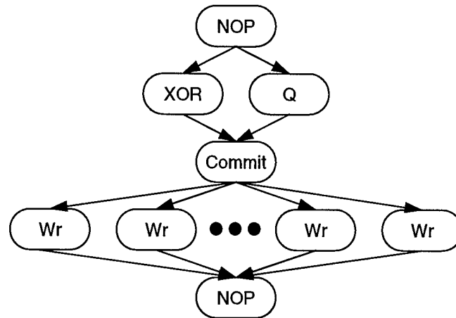
Figure B-15 PQ large-write graph
