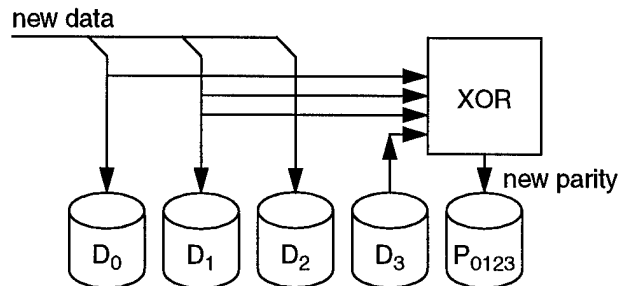
Figure 2-10 The reconstruct-write algorithm
