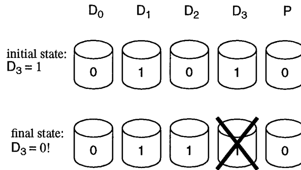
Figure 3-7 Constraining execution to ensure forward recovery
