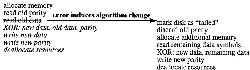
Figure 3-6 Forward error recovery
