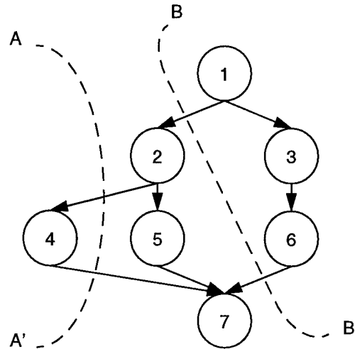
Figure 3-13 Pruning a graph for distributed execution
