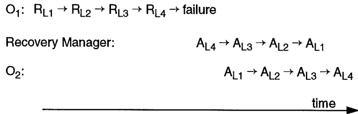
Figure 3-8 Deadlock resulting from out-of-order allocation during recovery
