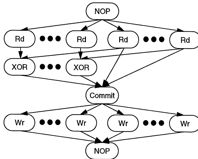
Figure B-19 2D degraded-H write graph
