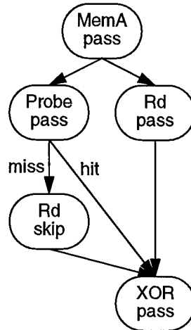
Figure 3-10 Sequencing a graph which contains a predicate
