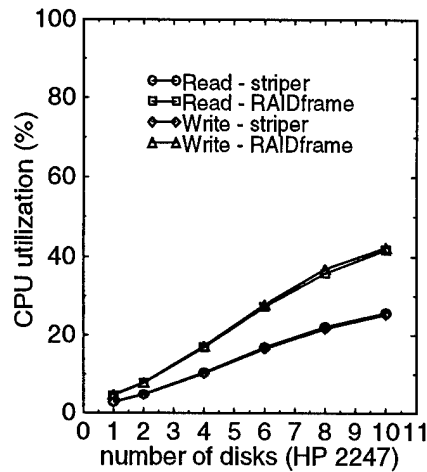
Figure 4-5(b): CPU consumption
