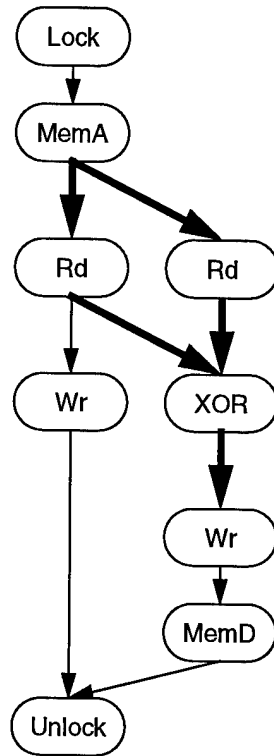
Figure 5-5(a): Initial graph
