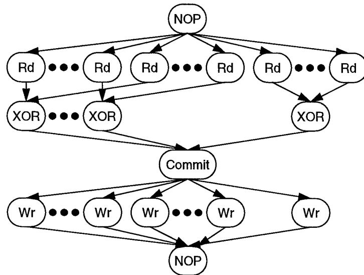
Figure B-20 2D degraded-DH write graph
