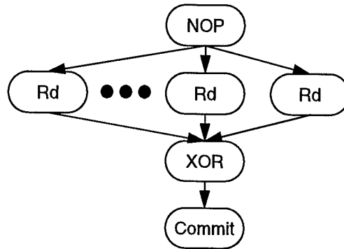
Figure 5-3 Degraded-read graph
