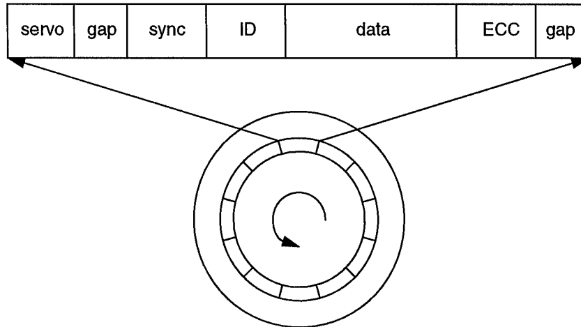
Figure 2-4 Typical sector formatting
