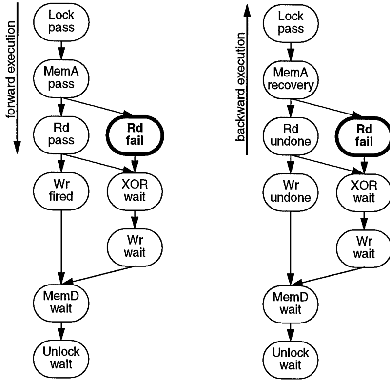
Figure 3-11 Error recovery from backward execution
