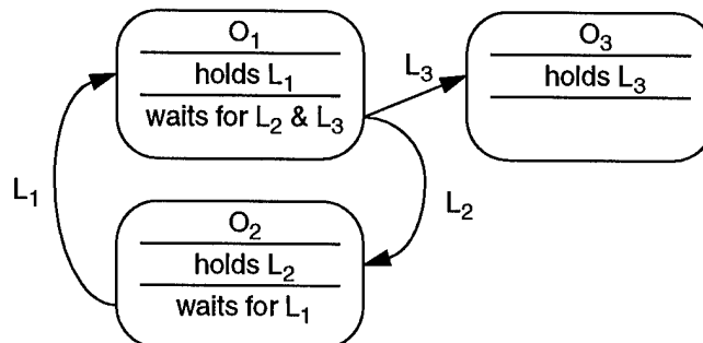
Figure 3-12 Detecting deadlock with a waits-for graph
