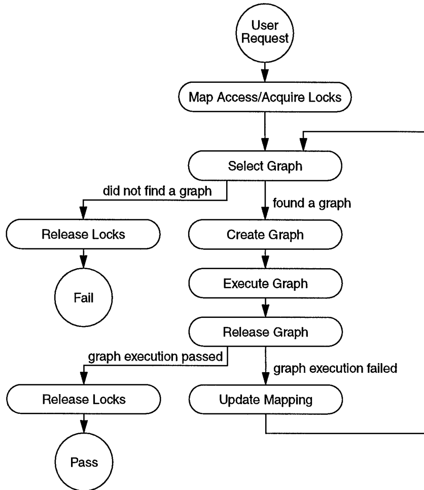
Figure 4-2 Mechanism for processing user requests
