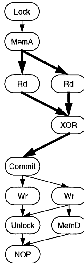
Figure 5-7(b): Step 5: eliminate an unnecessary control dependence
