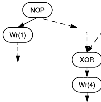
Figure 3-5(c): Dead Code Eliminated
