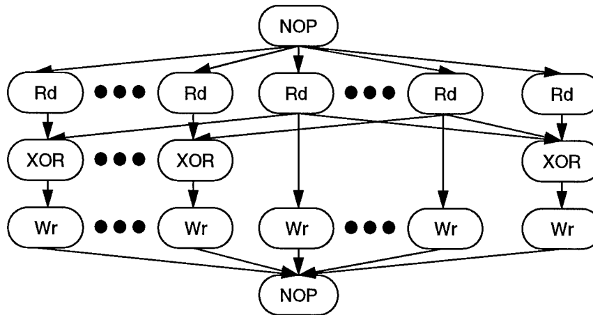
Figure A-17 2D small-write graph
