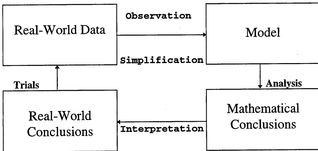
Figure 2: Modeling Process
