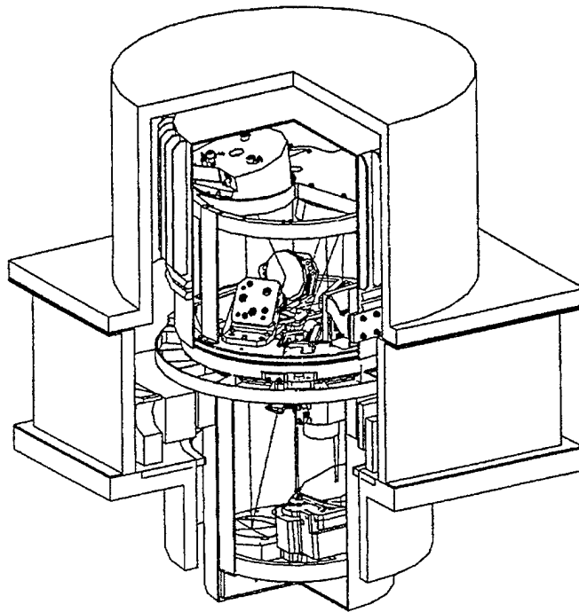
Figure 4.6. HYDICE Instrument (From Anderson, 1995)
