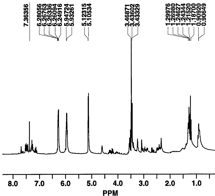
Figure 1. ^1\text{H} NMR spectrum of benzene oxide (singlets at 5.1, 5.9, and 6.2 ppm).
