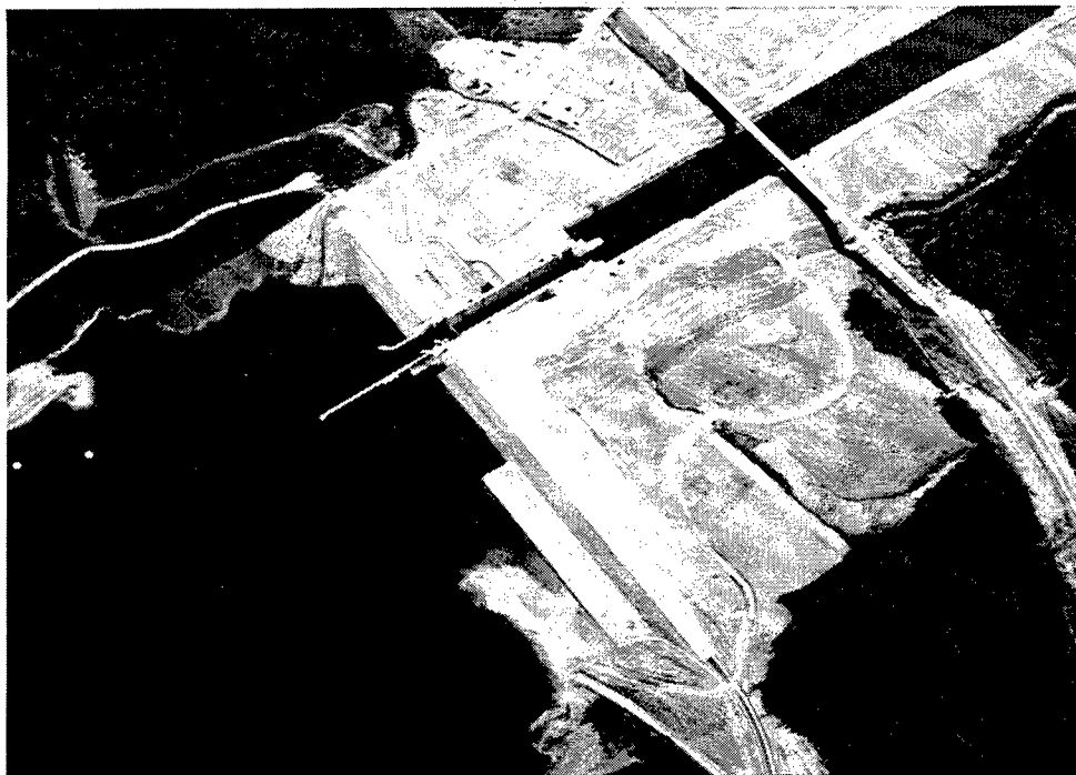
Figure 12. Bay Springs Lock, Tennessee-Tombigbee Waterway, illustrates a high-lift lock that bypasses the river regulation and flood control facilities
