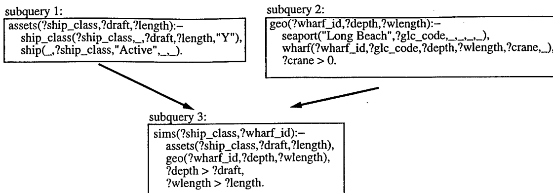
Figure 4.1: Example query plan that retrieves heterogeneous multidatabases
