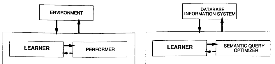
Figure 6.1: Learning for SQO as an instance of general autonomous learning
