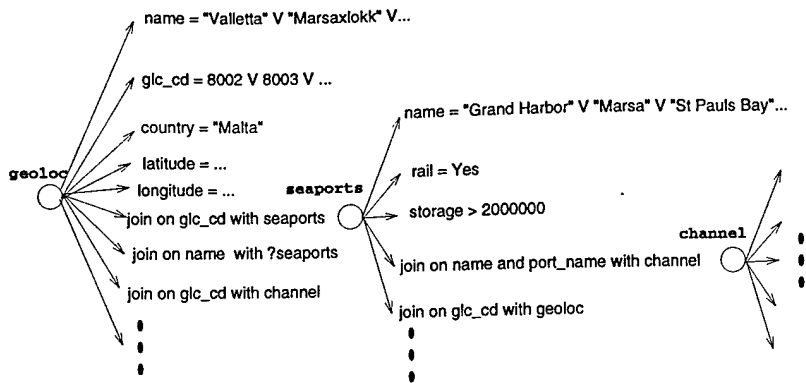
Figure 3.3: Candidate constraints to be selected
