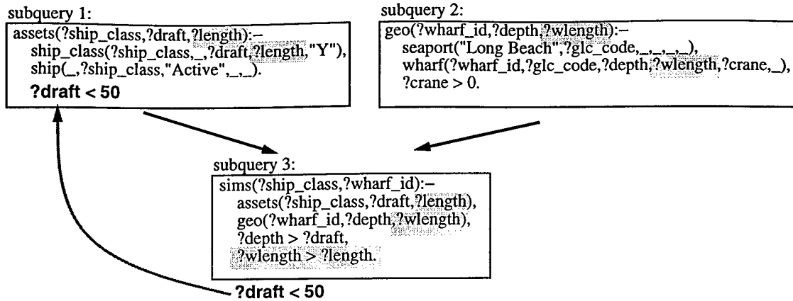
Figure 4.3: Propagating newly derived literals backward to optimize query plan
