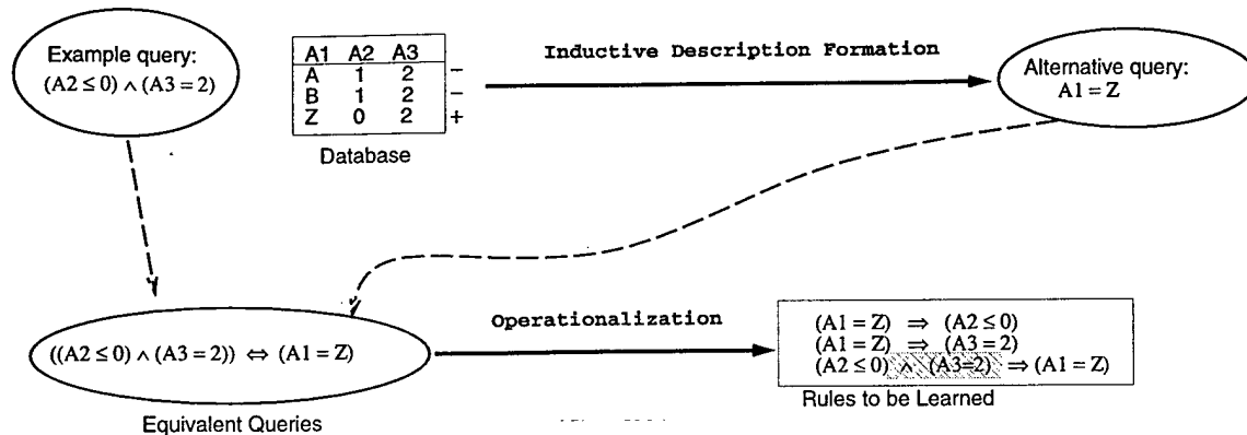
Figure 3.2: A simplified learning scenario
