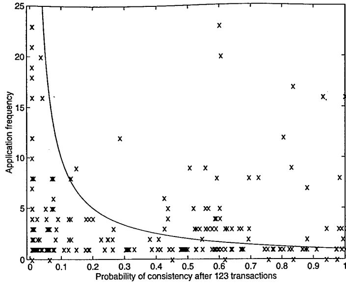
Figure 5.5: Relation between application frequency and estimated robustness
