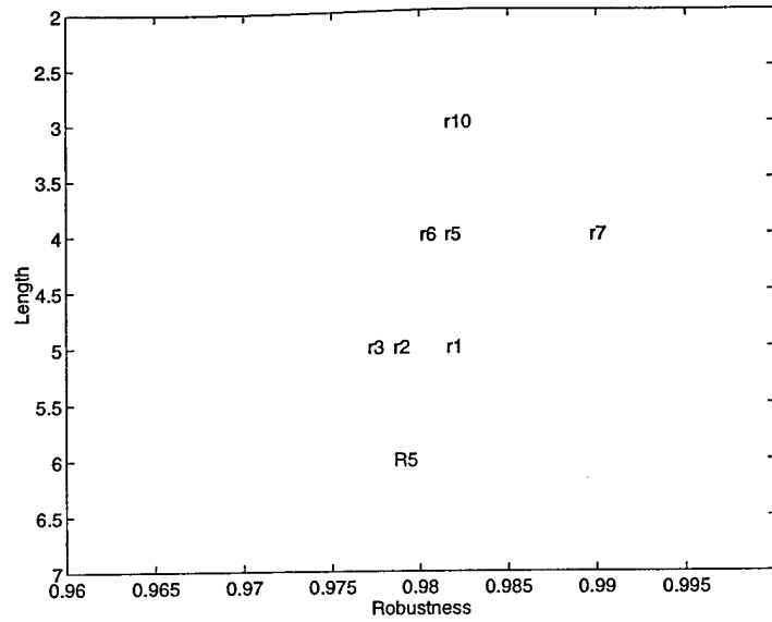
Figure 3.4: Pruned rules and their estimated robustness
