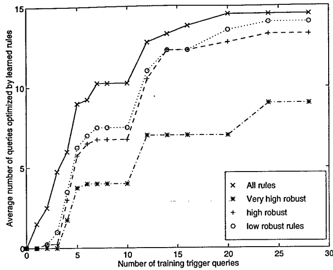
Figure 5.4: Rule coverage rates for rules of different robustness levels
