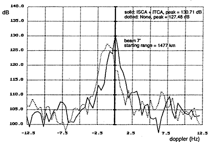
Figure 5.20. OTH Doppler Maps. The Abscissa Represents Doppler Frequency in Hz, and the Ordinate is Doppler Response in dB. The Dotted Curves are the Doppler Responses Without Self-Cohering. The Solid Curves are the Doppler Responses After Self-Cohering Using the ISCA + ITCA.
