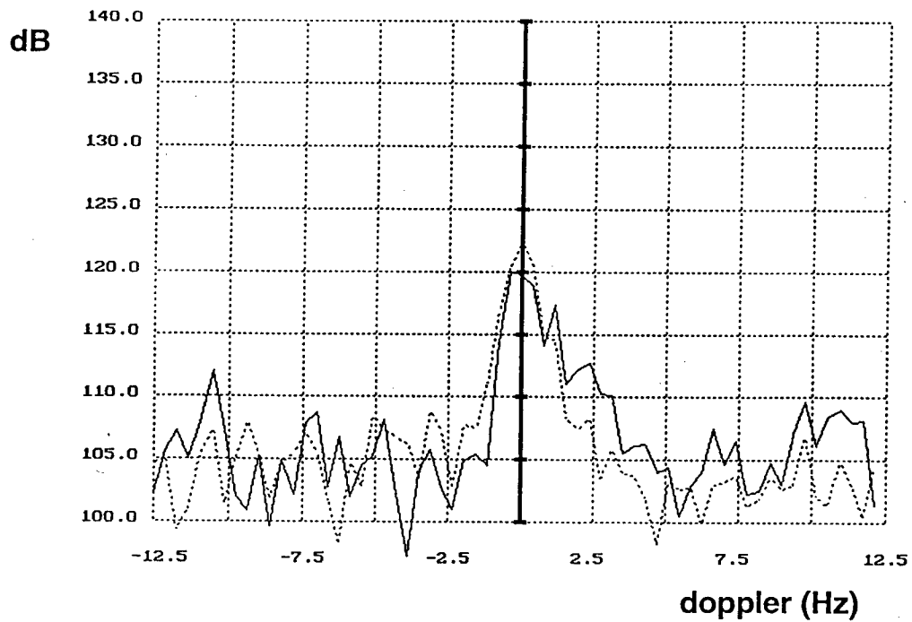
Figure 5.7. Averaged Doppler Cuts (2461-2520 km).
