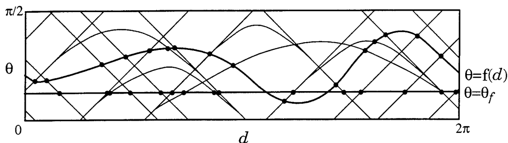
Figure 7.8: Modeling anisotropic directional uncertainty
