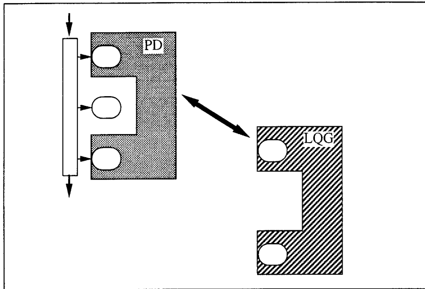
Figure 2.5: Configuration Manager
