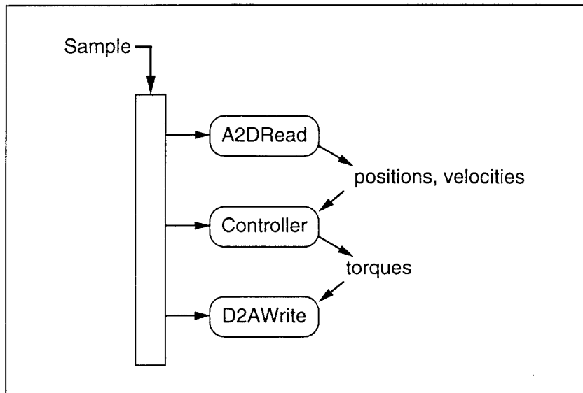
Figure 2.3: Dependency-Sorted List
