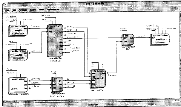
Figure 2.4: Data-Flow Editor
