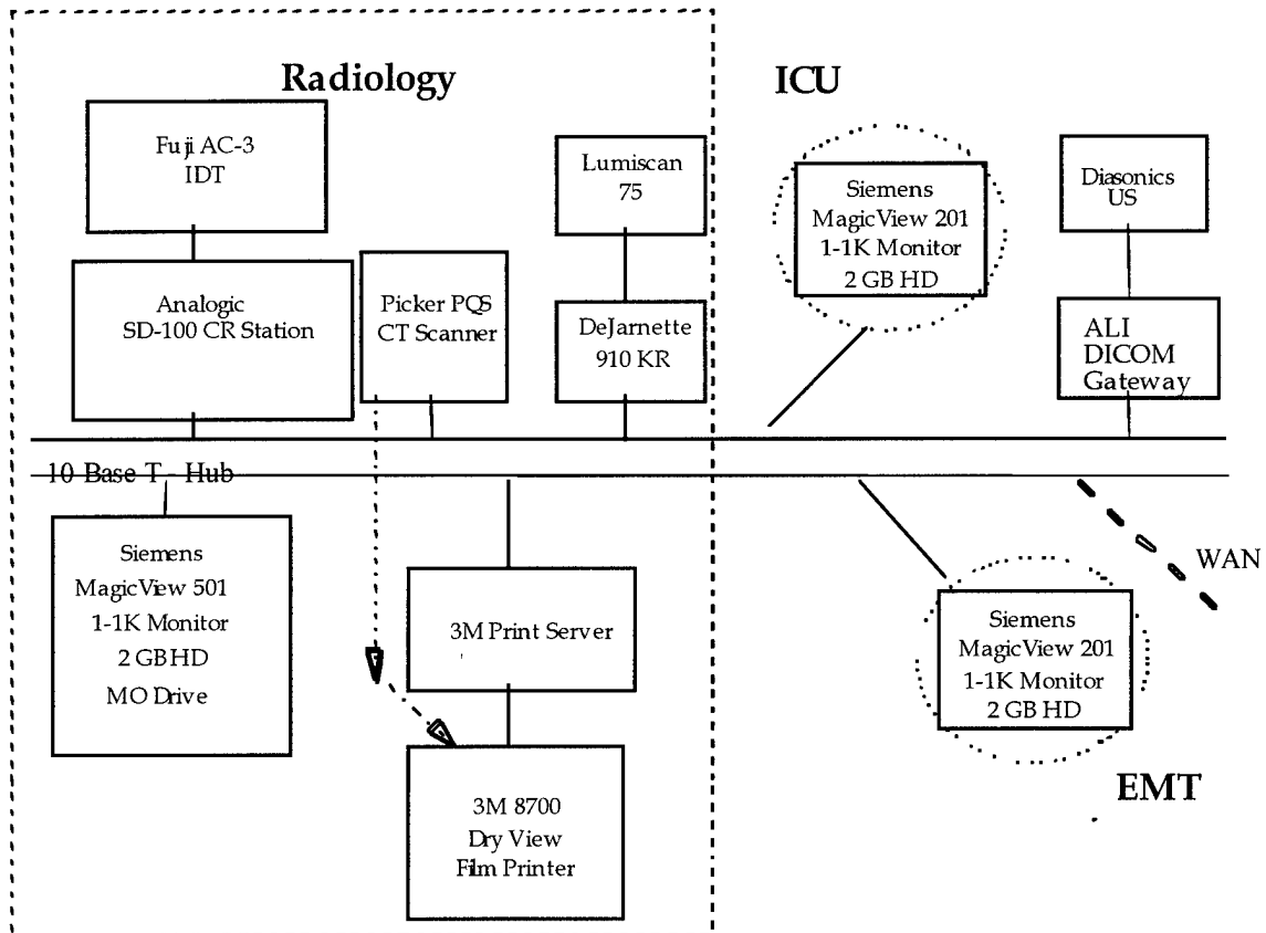
Figure 2.0 MASH Configuration
