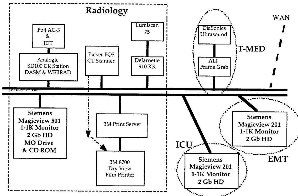
Figure 4.1 MASH network configuration
