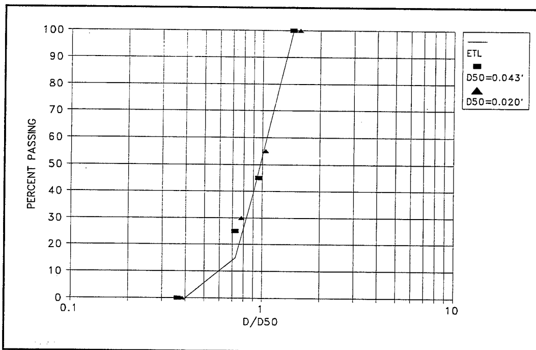
Figure 16. Model stone gradations used in Gallipolis lock approach study
