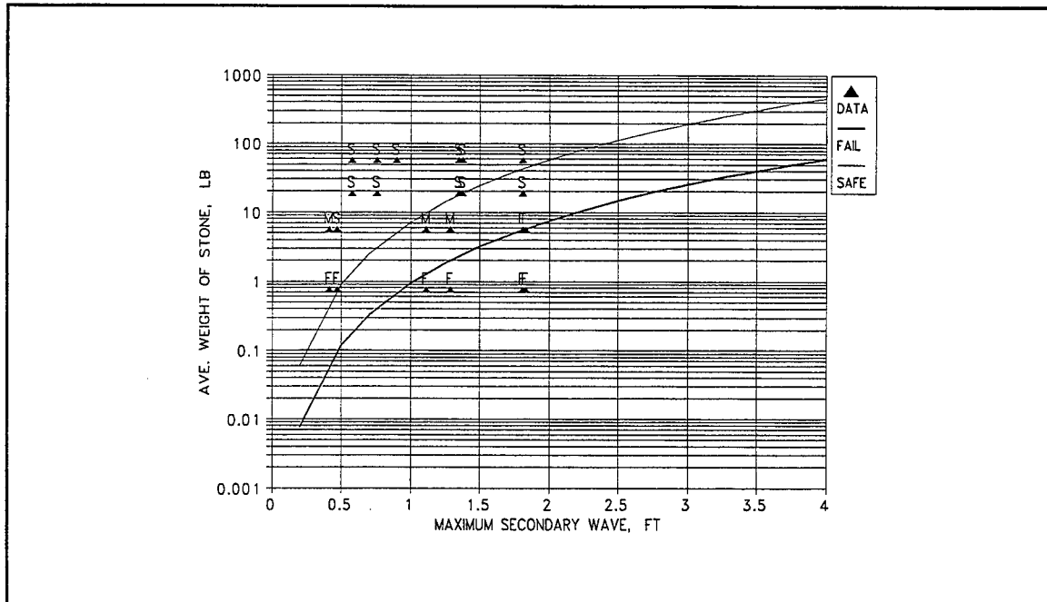
Figure 49. Determination of N_s for H_i , 2H:1V
