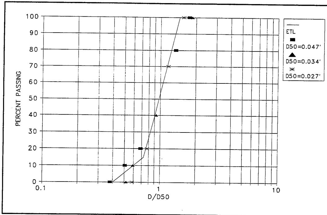
Figure 15. Model stone gradations used in Tennessee-Tombigbee study
