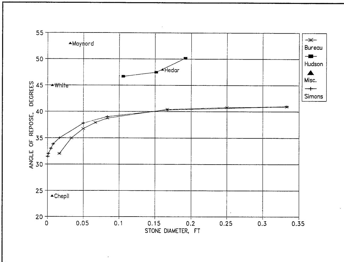
Figure 10. Comparison of angle of repose from various sources
