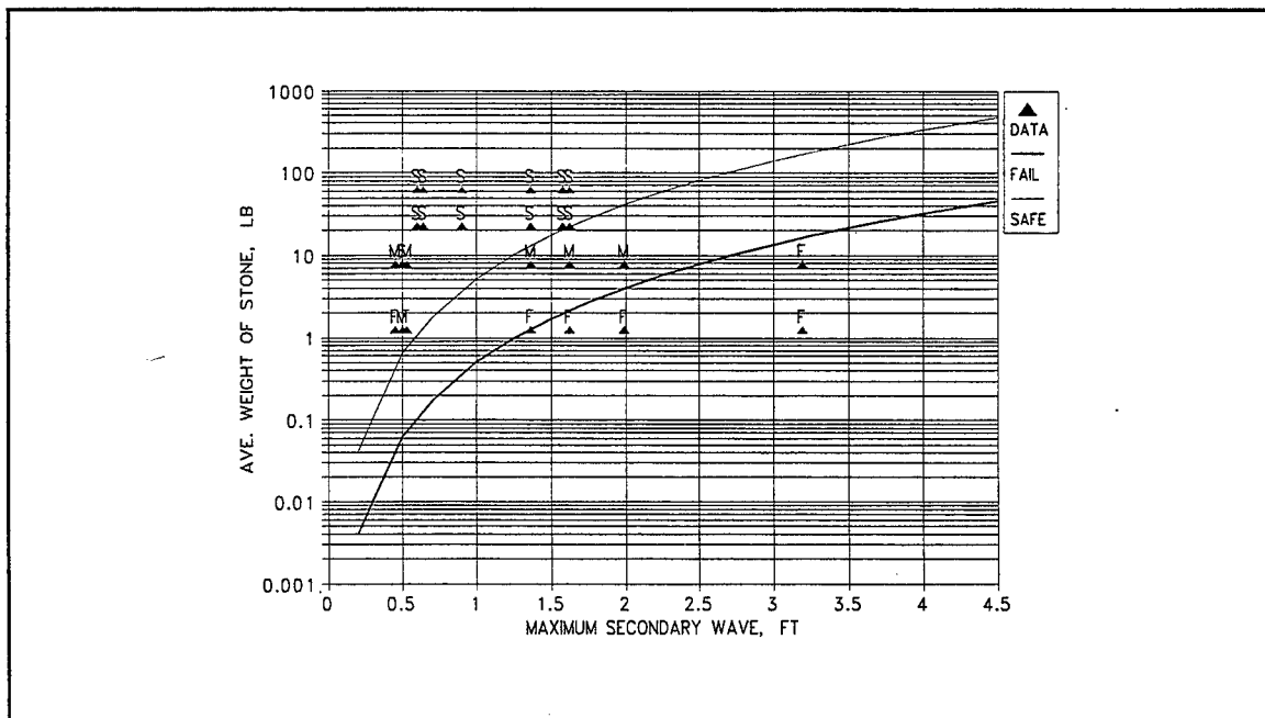
Figure 50. Determination of N_s for H_i , 3H:1V
