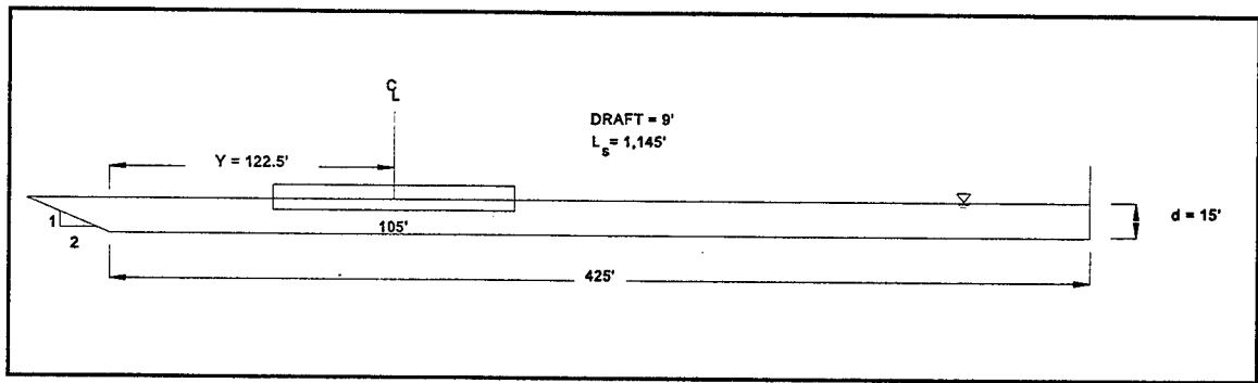
Figure 12. Pertinent cross-section and test data, Gallipolis study
