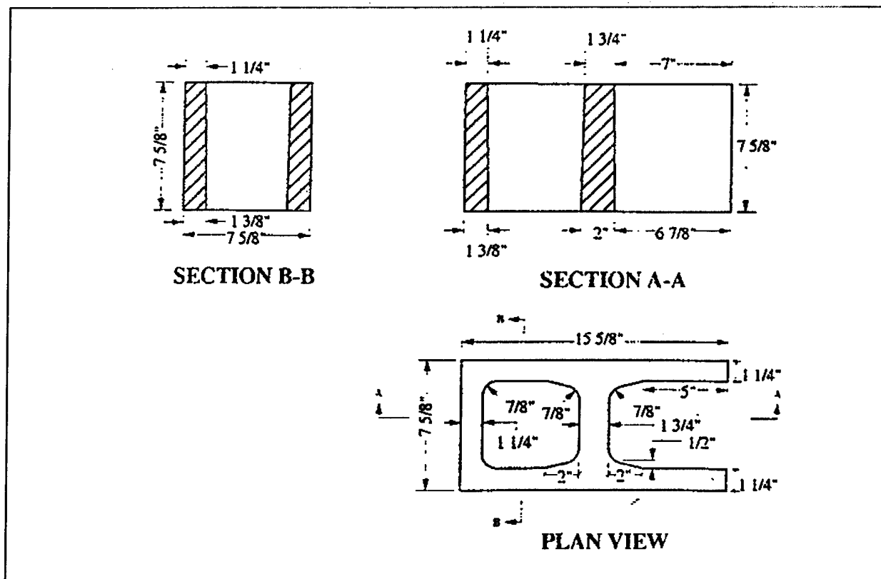
Figure 2.2. Standard 8 x 8 x 16-in. open-end CMU (A-block).
