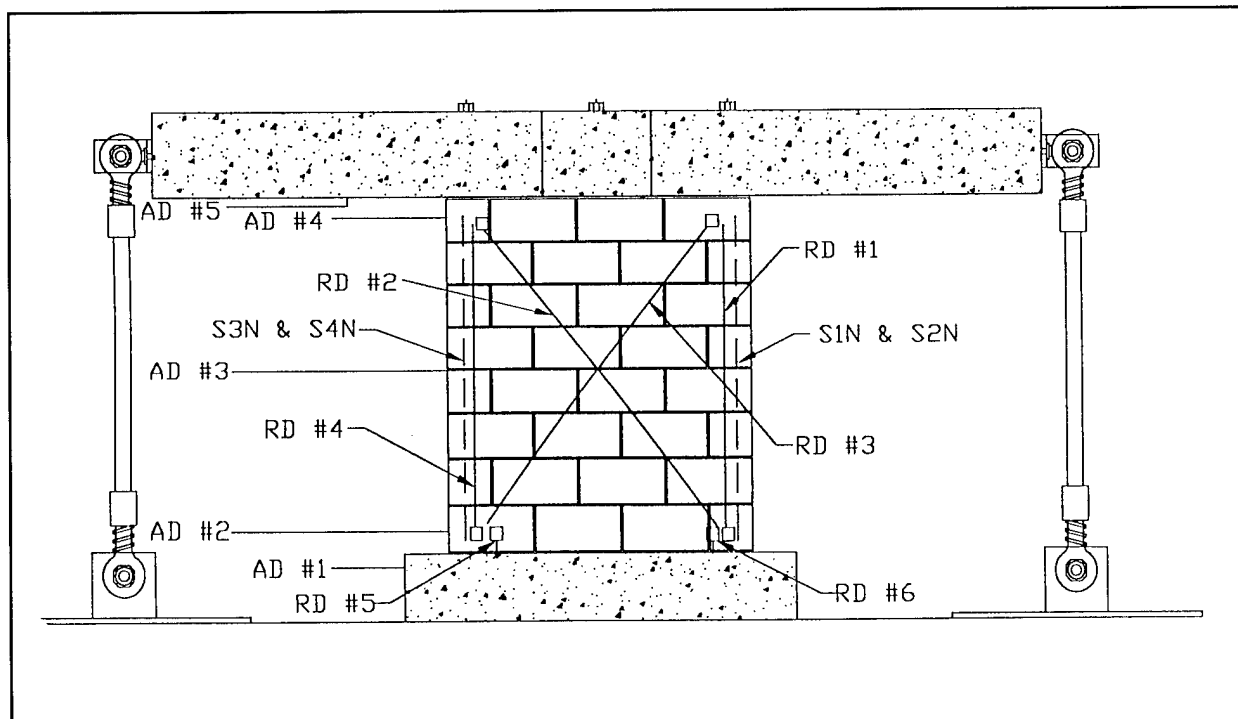
Figure 5.5. Instrumentation diagram for test setup.
