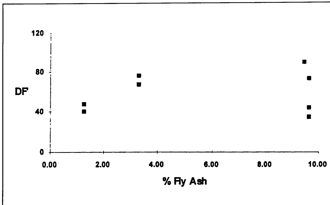
Figure 6.9. Durability factors vs percent fly ash lightweight mixes.
