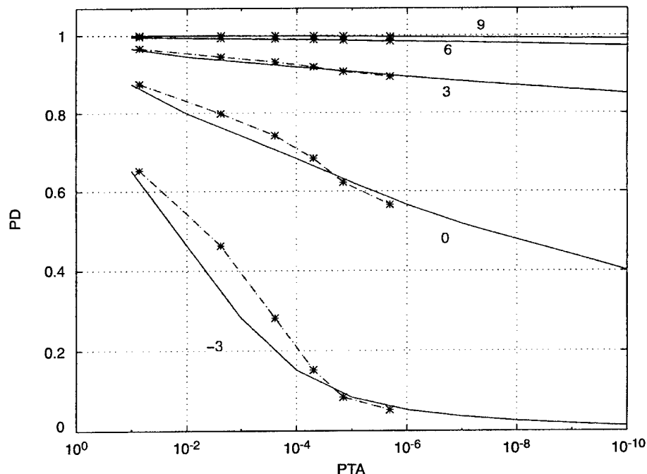
Figure 11. Empirical ROC curves for the OSMD, applied to the high-resolution radar data modeled in figure 2, using signal levels so that the average SNR over 4-second blocks of data were -3 , 0 , 3 , 6 , and 9 dB. The false alarm probability as a function of the threshold was calculated empirically and theoretically to produce the curves (***) and (—), respectively.
