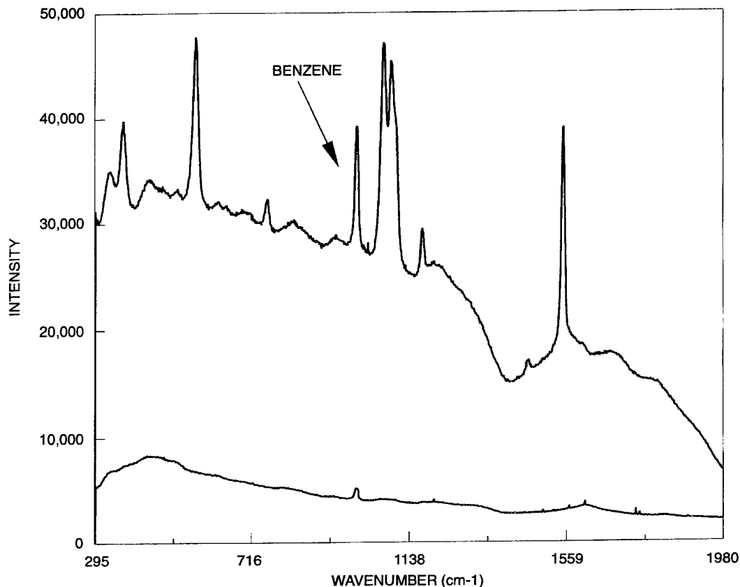
Figure 2. The bottom spectrum is of 661-ppm benzene in water. The top spectrum shows the SERS response of 4-chlorothiophenol on a roughened Ag substrate. The substrate is immersed in an aqueous 661-ppm benzene solution. The spectrum clearly shows the partitioning of benzene into the 4-chlorothiophenol coating.
