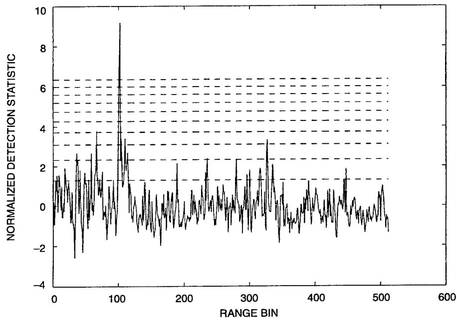
Figure 9. The HMM detector applied to the data in figure 5.
