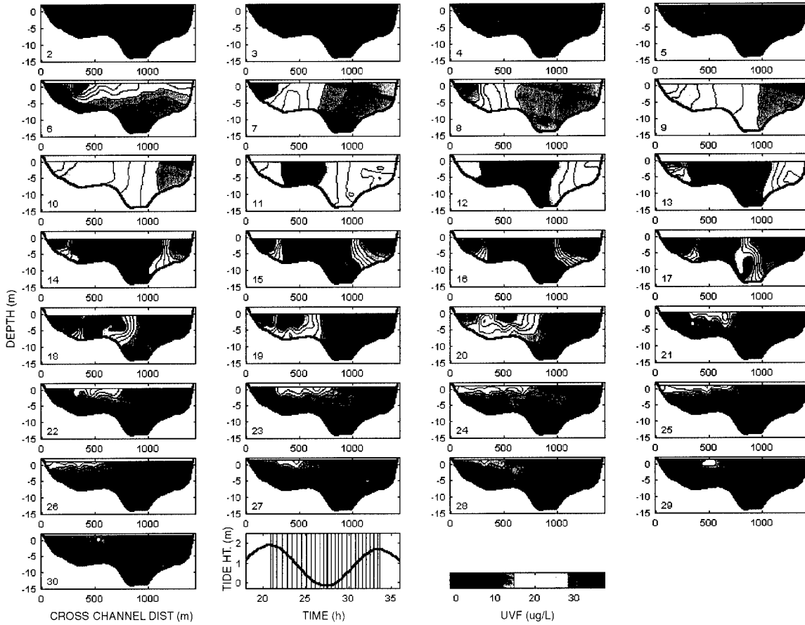
Figure 10. Cross-sectional time series of UVF at the mouth section during 95MOUTH-2.
