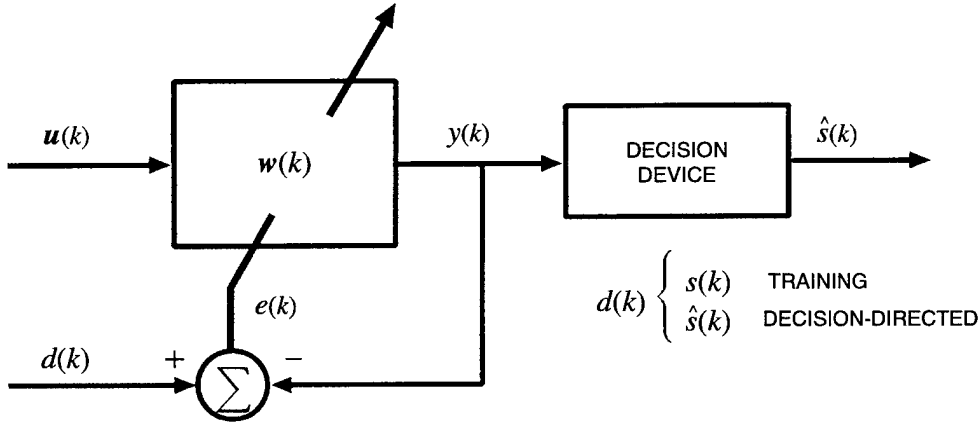
Figure 1. Adaptive equalizer structure.
