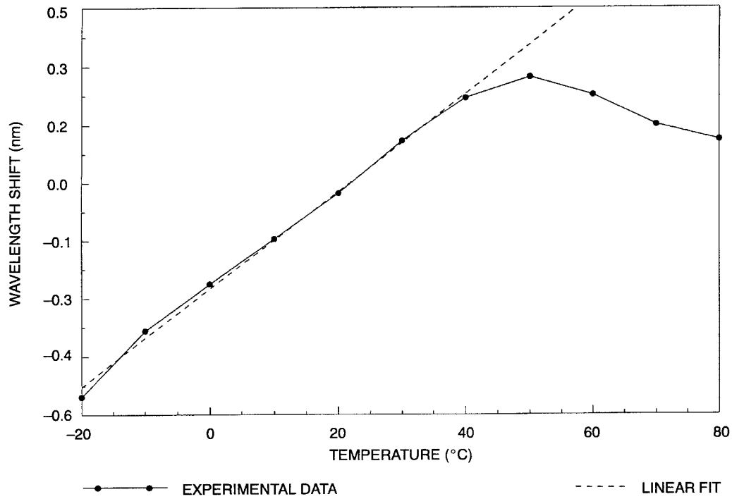
Figure 2. Temperature dependence of the peak channel wavelength of an 8.5-nm PINC WDM.
