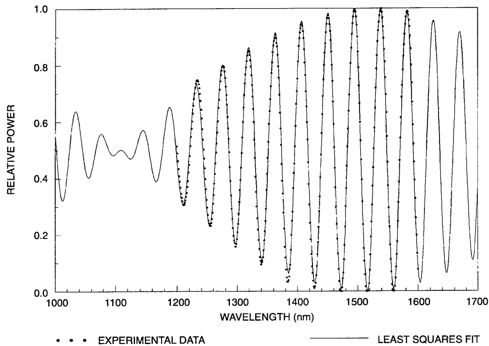
Figure 3. Wavelength response curves for PINC WDM coupler: 22-nm channel spacing.
