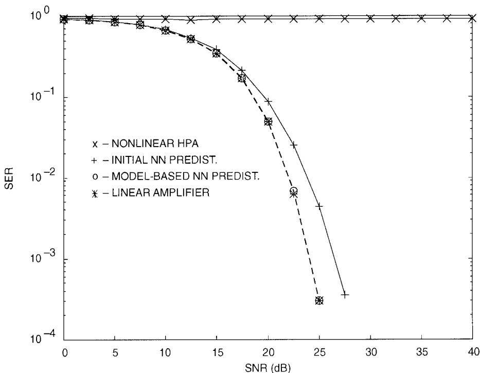
Figure 2. SER performance for 64 QAM.
