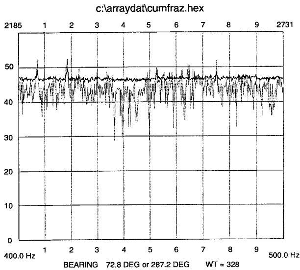
Figure 7. Spectrum and fourth cumulant for 400- to 500-Hz band in noisy beam.
