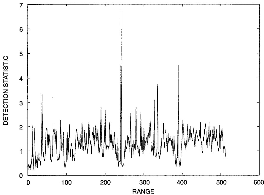
Figure 7. A CFAR processor applied to the data in figure 5.
