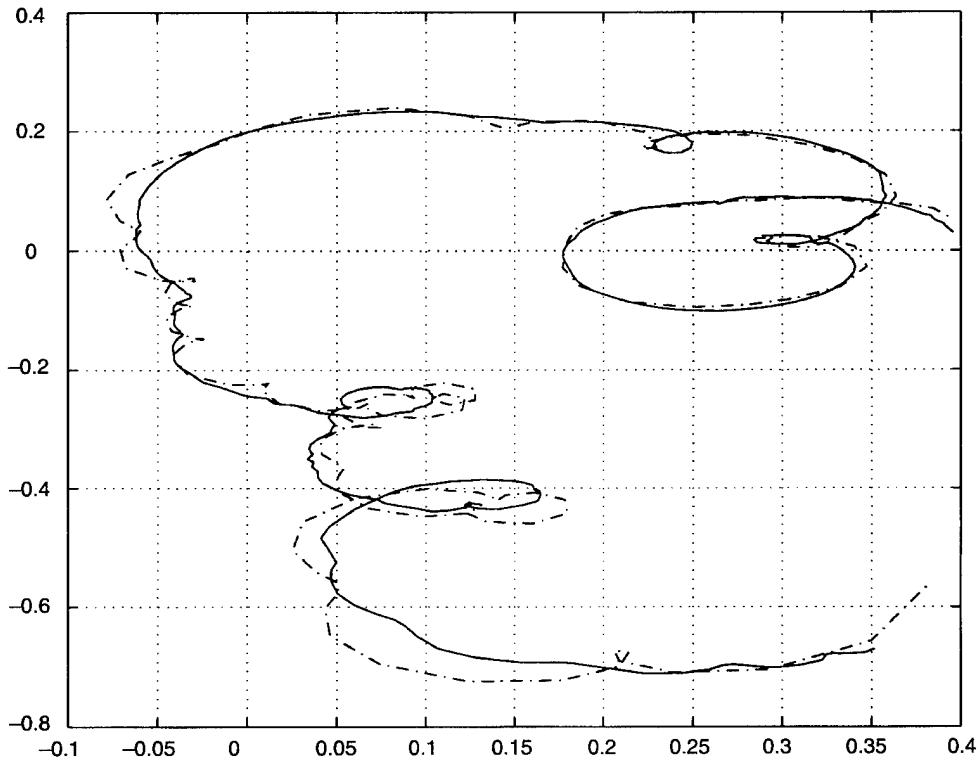
Figure 1. Estimate resulting from the constrained Nehari method.
