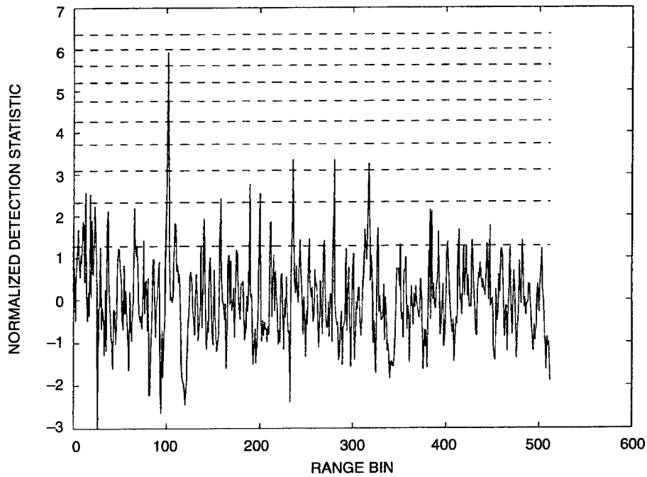
Figure 8. The OSMD applied to the data in figure 5.
