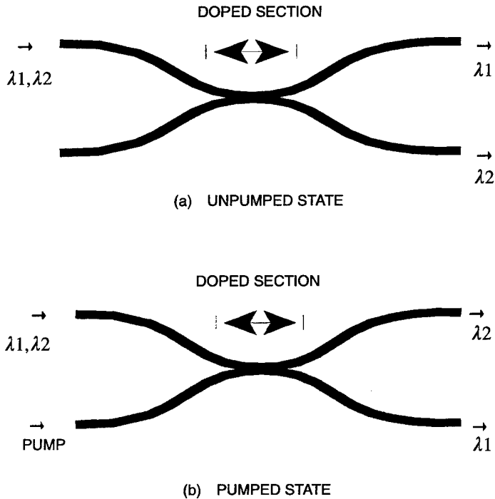
Figure 7. All-optical wavelength router/switch ( \Delta\lambda = \Delta\lambda_{WDM} ).
