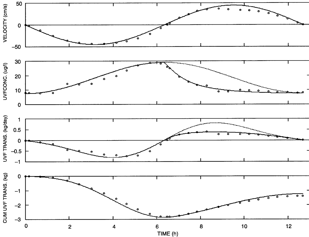
Figure 11. Time series of cross-sectional averages of (a) velocity, (b) UVF, (c) UVF transport, and (d) cumulative UVF transport. Open circles are measured data; solid lines are modeled results from equation 14 for the ebb tide and equation 15 for the flood tide. The dashed line represents the expected concentration and transport in the absence of tidal pumping.
