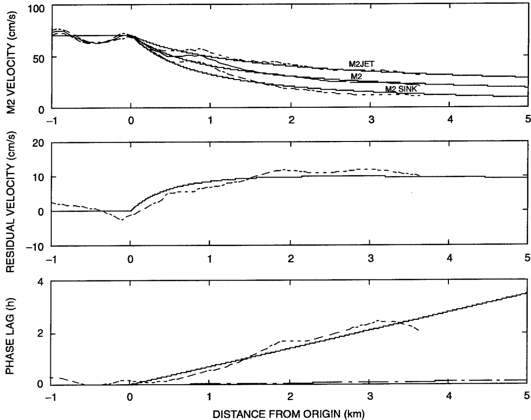
Figure 7. Fitted and measured centerline characteristics of the flow including (a) jet, sink, and M2 velocities; (b) residual velocity; and (c) phase lag.
