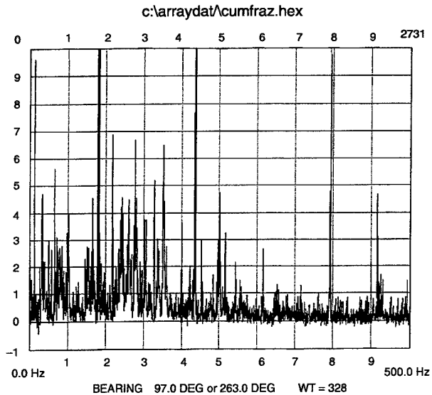
Figure 2. Normalized and fourth cumulant for quiet beam.
