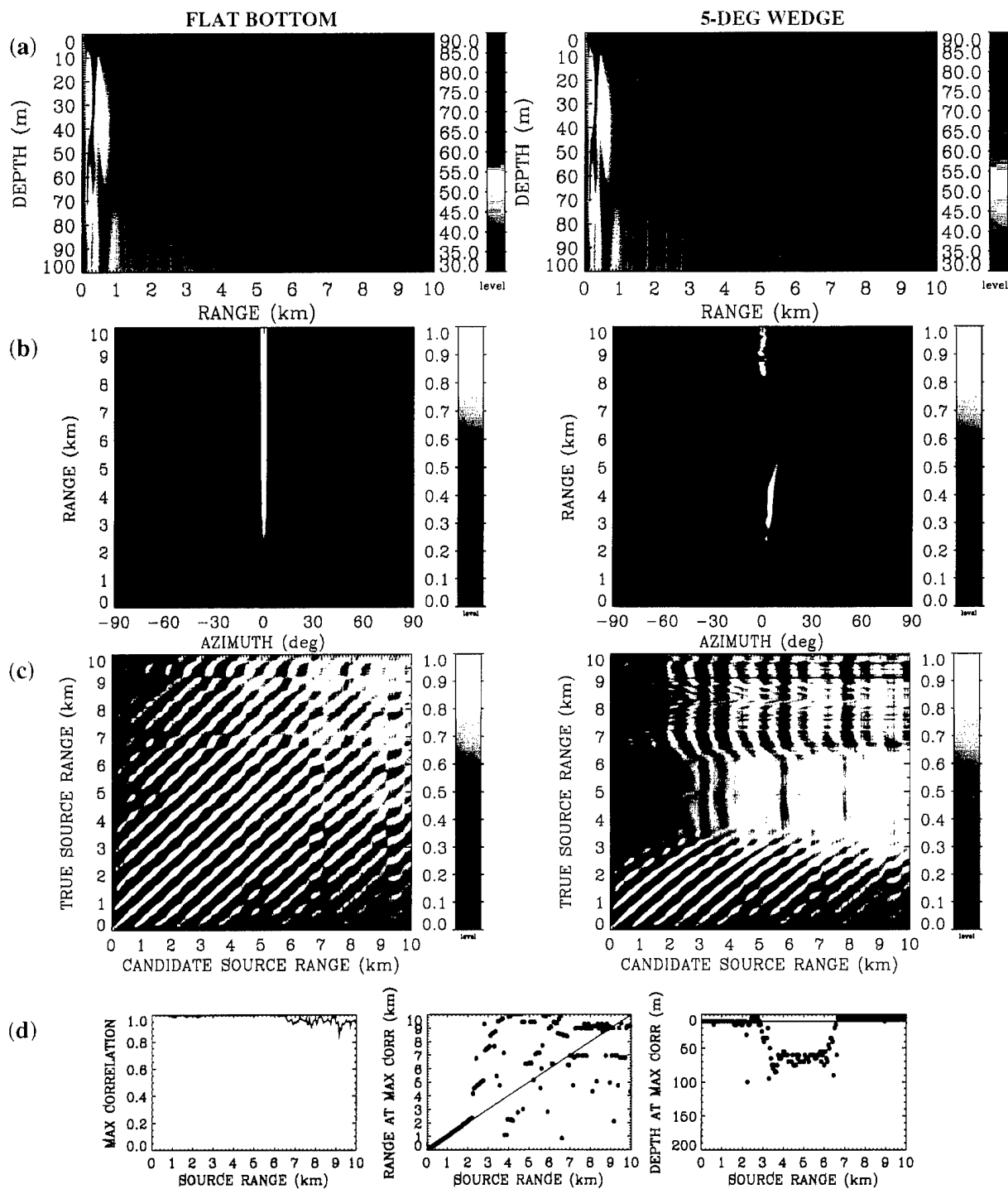
Figure 1. Typical 3-D bathymetric effects on (a) signal field, (b) HLA beam response, and (c and d) VLA matched-field response. Frequency = 25 Hz. Source depth = 10 m. Water depth along track = 100 m. In (a) through (c), the left column is for a flat bottom while the right column is for a 5-degree wedge. In (b), source track is in broadside direction to HLA aperture. All matched-field results use replicas obtained for flat bottom. In (c), candidate source depth = 10 m, and main peak track begins near zero candidate source range (near diagonal in left column). Large sidelobes occur in (c) because only a few modes propagate at this frequency and water depth. In (d), the maximum correlation, and the candidate range and depth of that maximum, for the full range-depth ambiguity surfaces, are plotted over the direction of the track. In (d), the light solid line represents results for flat bottom, for which the maximum correlation is always unity (no mismatch).
