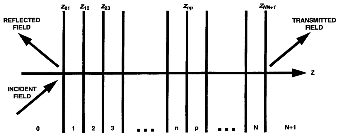
Figure 1. Multilayer thin-film geometry.
