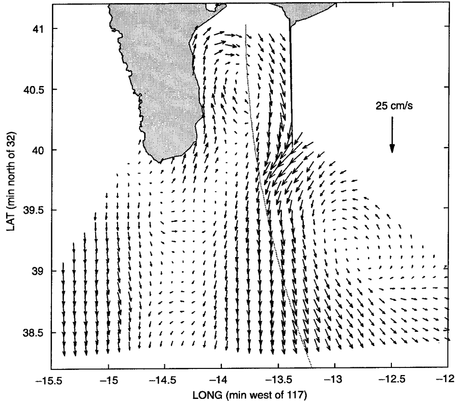
Figure 6. Horizontal structure of the tidally averaged residual flow.
