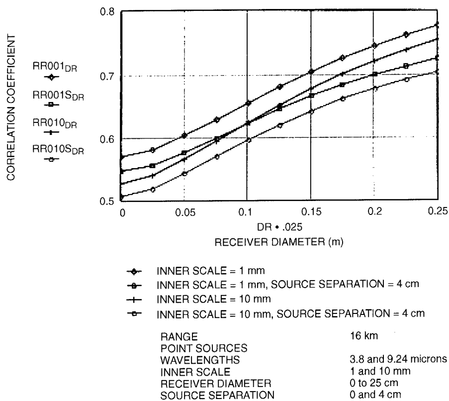
Figure 2. Bichromatic correlation as a function of receiver diameter.
