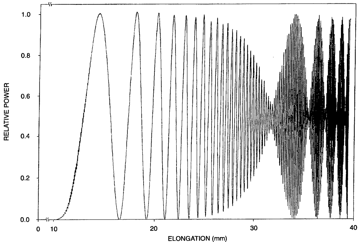
Figure 1. Coupled power as a function of pulled length in a fused-fiber coupler.
