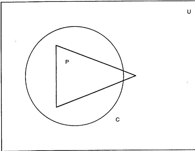
Figure 1. A Venn diagram illustrating what it means for a set of premises to imply a conclusion. The rectangle, U , is the set of all models. The triangle, P , is the set of models in which the premises are true. The circle, C , is the set of models in which the conclusion is true. The conclusion is implied by the premises because nearly every model of the premises is a model of the conclusion. Thus, in a valid implication, the conclusion has a high probability of being correct but is typically not certain to be correct.
