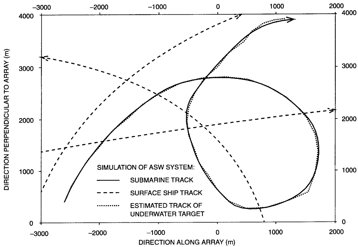
Figure 1. Submarine and three surface ships in shallow channel with sloping bottom.
