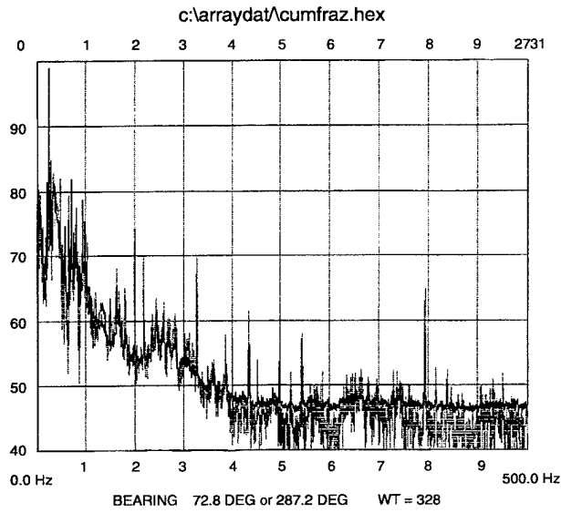
Figure 5. Spectrum and fourth cumulant for noisy beam.
