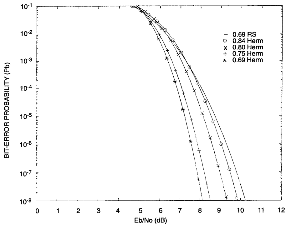
Figure 1. Bit-error probability versus SNR for low-rate RS code and selected Hermitian codes over F_{16} .
