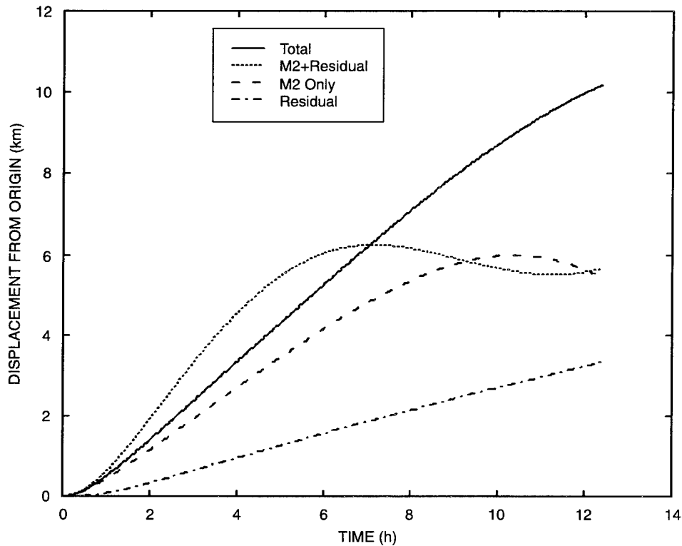
Figure 8. Predicted one-dimensional trajectories of particles released at the mouth of the bay at slack high water.
