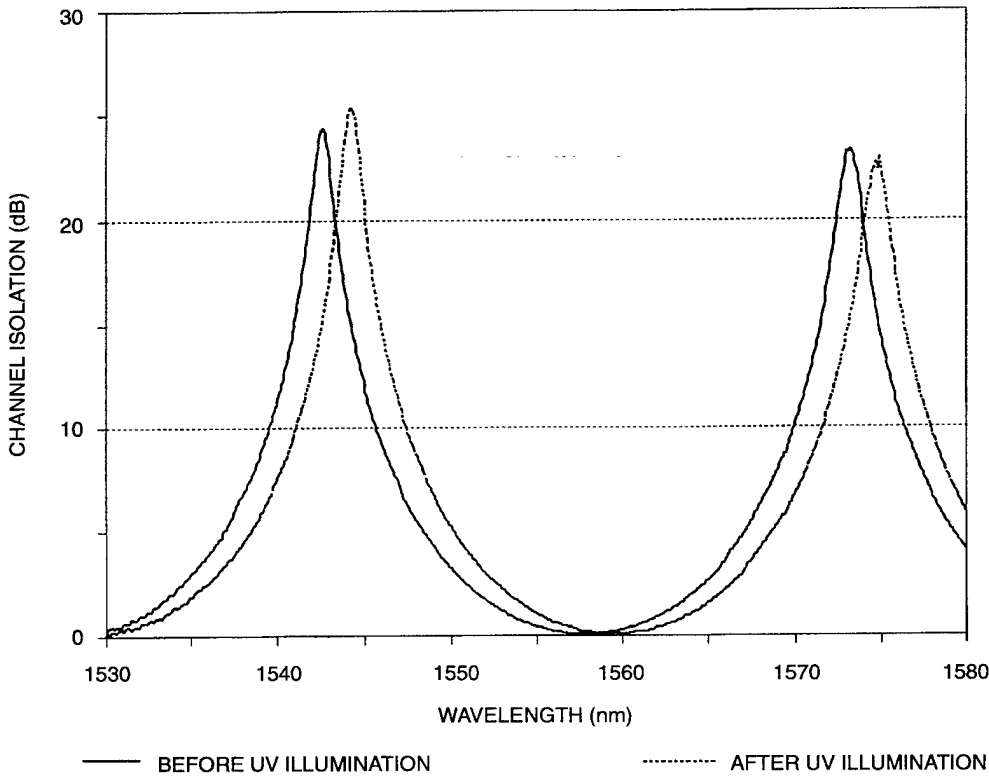
Figure 4. Wavelength response of one arm of a PINC WDM with 15-nm channel separation.
