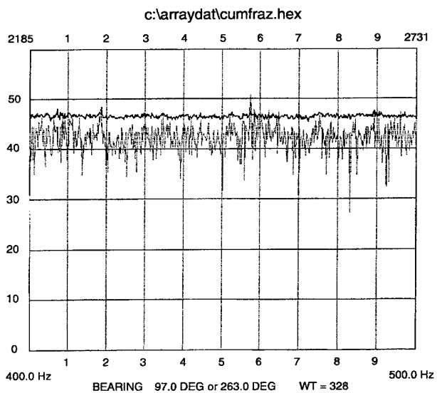
Figure 3. Spectrum and fourth cumulant for 457-Hz signal in quiet beam.
