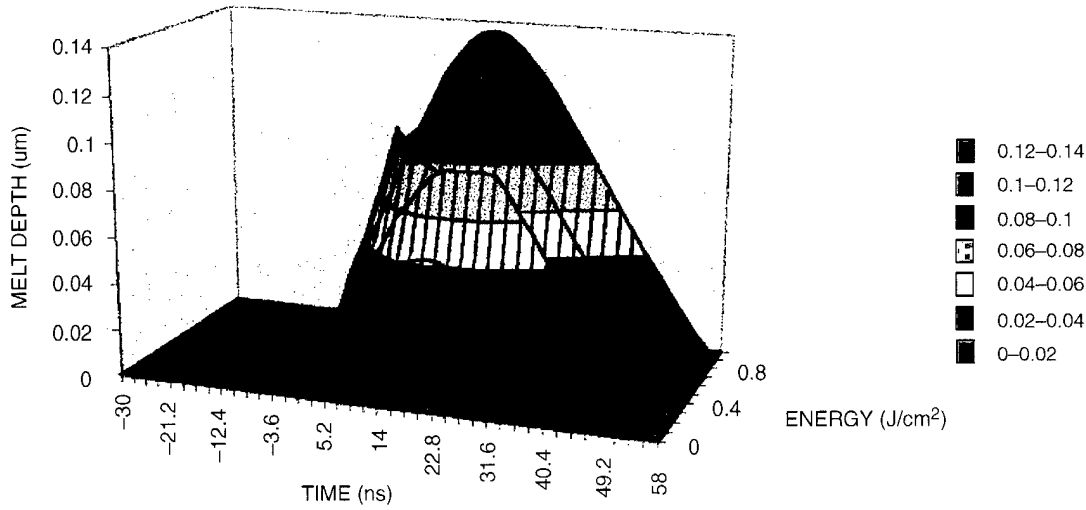
Figure 2. Modeled 3-D plot of thin silicon film melting on a sapphire substrate with a linear graded intensity beam.
