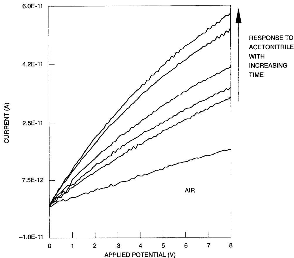
Figure 1. Voltammetric response of acetonitrile in the gas phase at room temperature. A 25- \mu l aliquot of acetonitrile was injected into a 5-ml glass flask. The evaporation of acetonitrile was monitored electrochemically using a UME array in which the inner working electrode was a 7- \mu m C disk, and the outer auxiliary electrode was an Au ring. Sweep rate was 100 \text{mv s}^{-1} .
