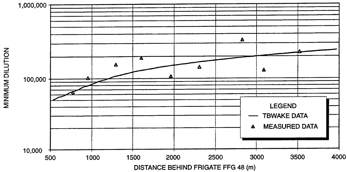
Figure 1. Comparison of TBWAKE solution with measured dye dilution.
