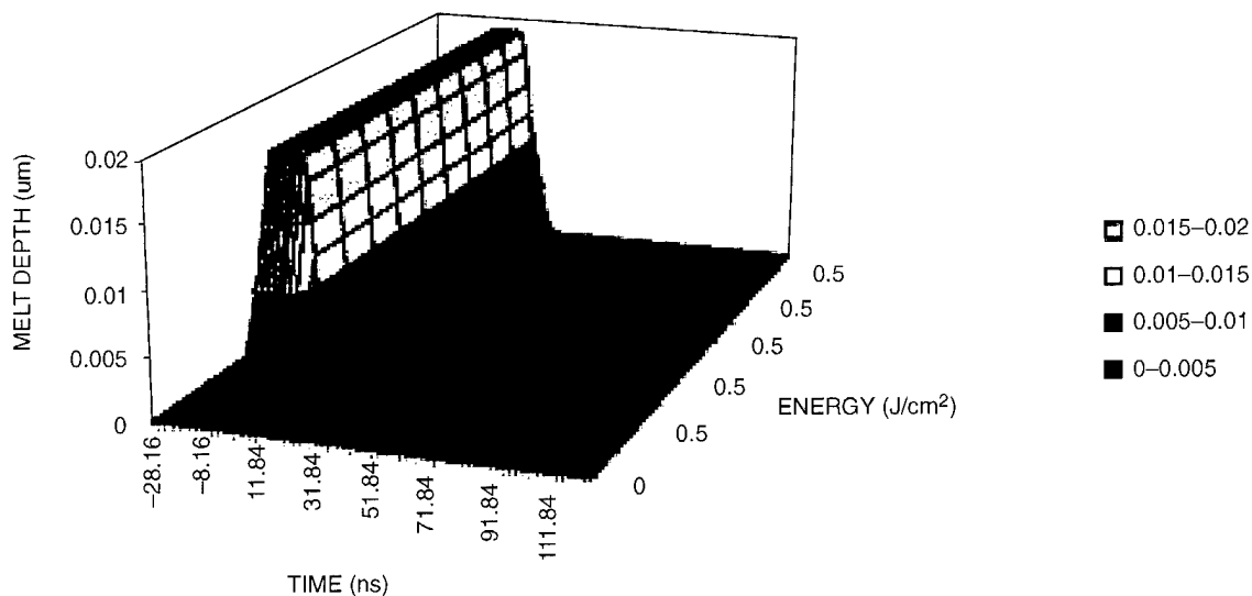
Figure 1. Modeled 3-D plot of thin silicon film melting on a sapphire substrate with a uniform intensity beam.
