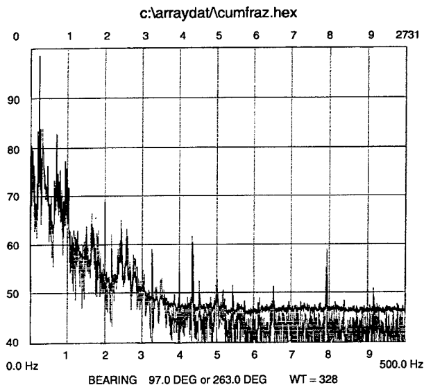
Figure 1. Spectrum and fourth cumulant for quiet beam.
