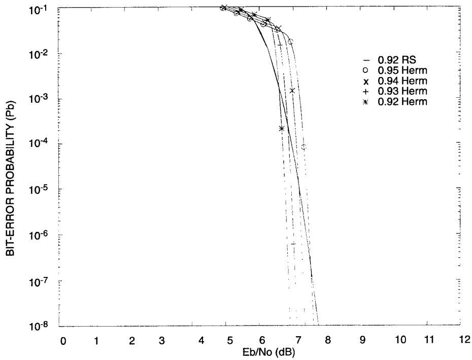
Figure 3. Bit-error probability versus SNR for low-rate RS code and selected Hermitian codes over F_{256} .
