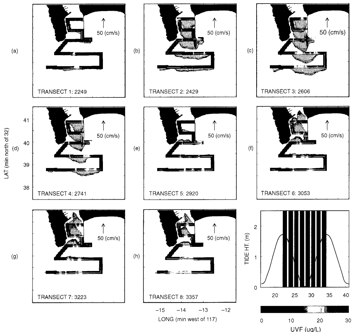
Figure 4. Horizontal structure of the tidal flow field and UVF concentrations from the mapping survey 95MAP.
