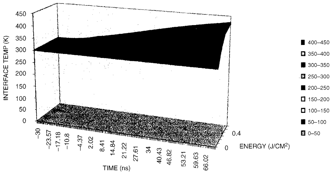
Figure 3. Modeled 3-D plot of the interface temperature between a fused silica thermal barrier and the silicon substrate as a result of linear-graded intensity beam heating of a thin silicon film.
