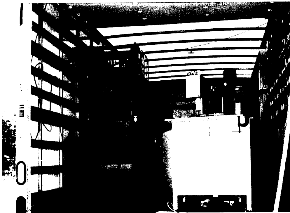
Figure 1. 20-cm aperture telescope and sandwich detector.
