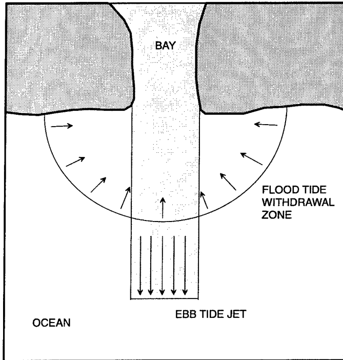
Figure 1. The tidal pumping model of Stommel and Farmer (1952), with the ebb flow as a rectangular jet, the flood flow as a semi-circular sink, and the exchange determined by the overlap of the jet and sink.
