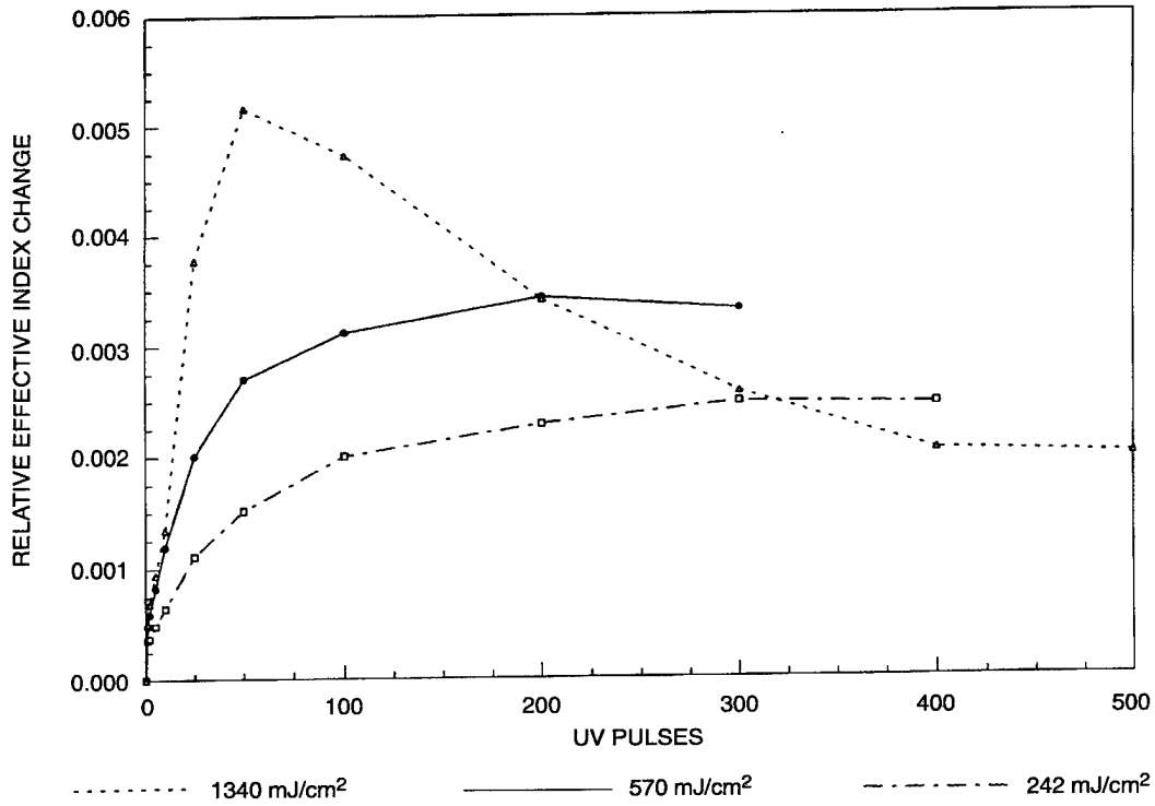
Figure 5. Effective index change vs. UV pulses for various pulse energies: 55-cycle couplers.
