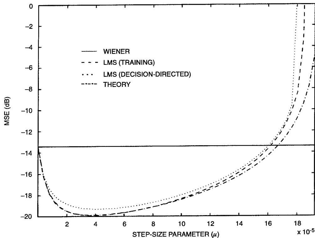
Figure 2. LMS MSE as a function of \mu for a sinusoidal interference, with L = 51 , SNR = 25 dB, and SIR = -20 dB.
