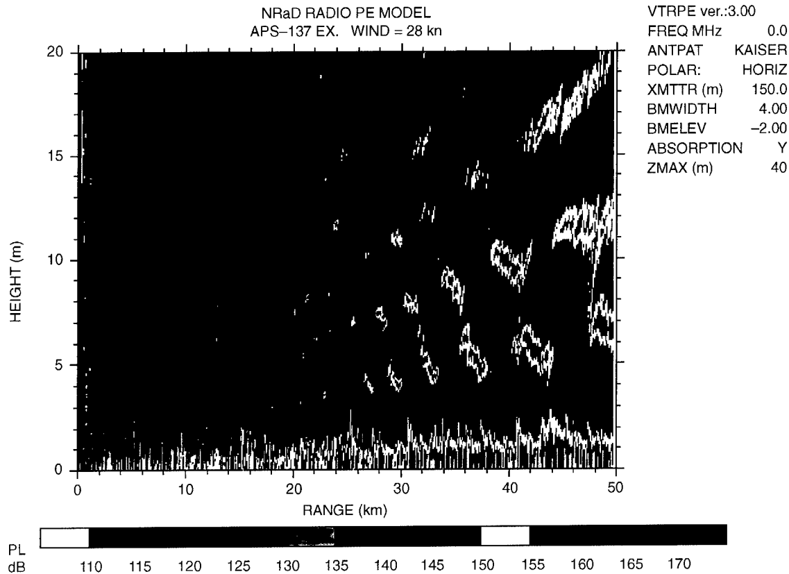
Figure 1. APS-137 sea clutter.
