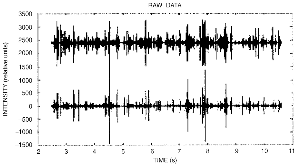
Figure 3. Raw data: red/bottom curve ( CO_2 ), blue/top curve (DF). The separation between the curves is for viewing purposes only.
