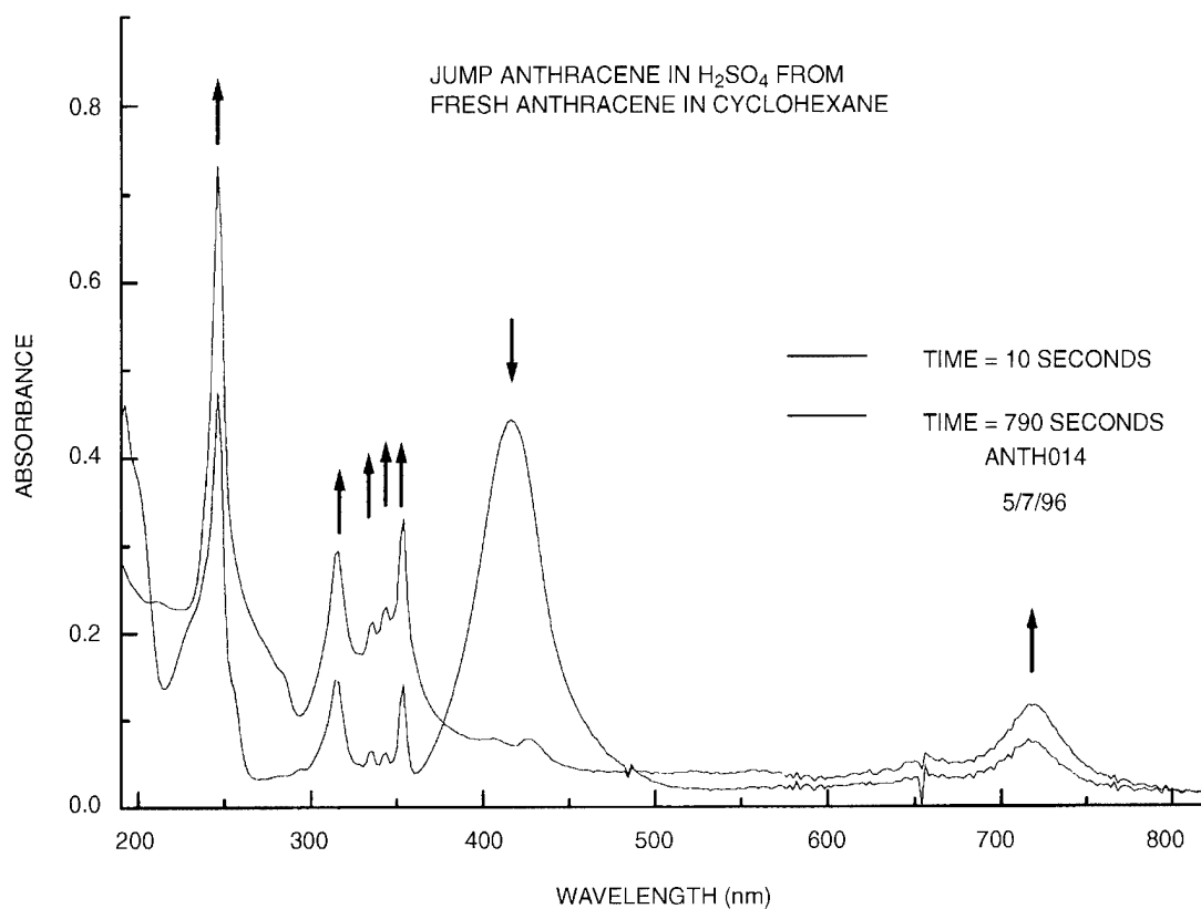
Figure 1. Absorption spectra at t = 10\text{ s} and t = 790\text{ s} of candidate jump molecule anthracene in sulphuric acid. Note that impurity peaks (indicated by up arrows) increase with time; the peak at 424 nm due to protonated anthracene (indicated by a down arrow) decreases with time.
