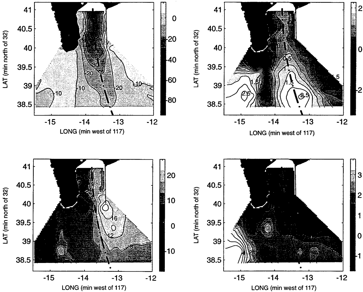
Figure 5. M2 tidal characteristics of the horizontal flow including (a) N-S amplitude, (b) N-S phase, (c) E-W amplitude, and (d) E-W phase. Velocities are in cm · s -1 and phase lag (+) is in hours from high water.
