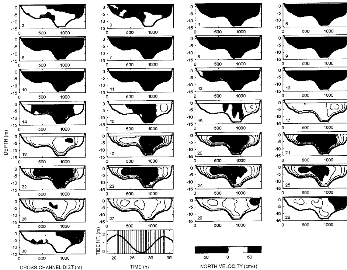
Figure 9. Cross-sectional time series of flow at the mouth section during 95MOUTH-2.
