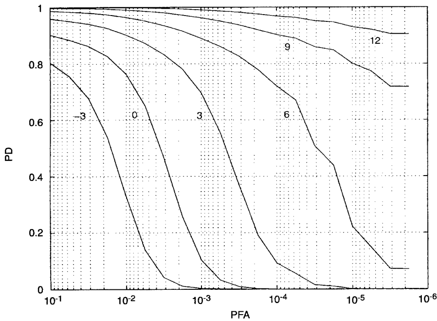
Figure 10. Empirical ROC curves for CFAR_1_2_100 using signal levels so that the average SNR over 4-second blocks of data were -3 , 0 , 3 , 6 , 9 , and 12 dB applied to the high-resolution radar data modeled in figure 2.
