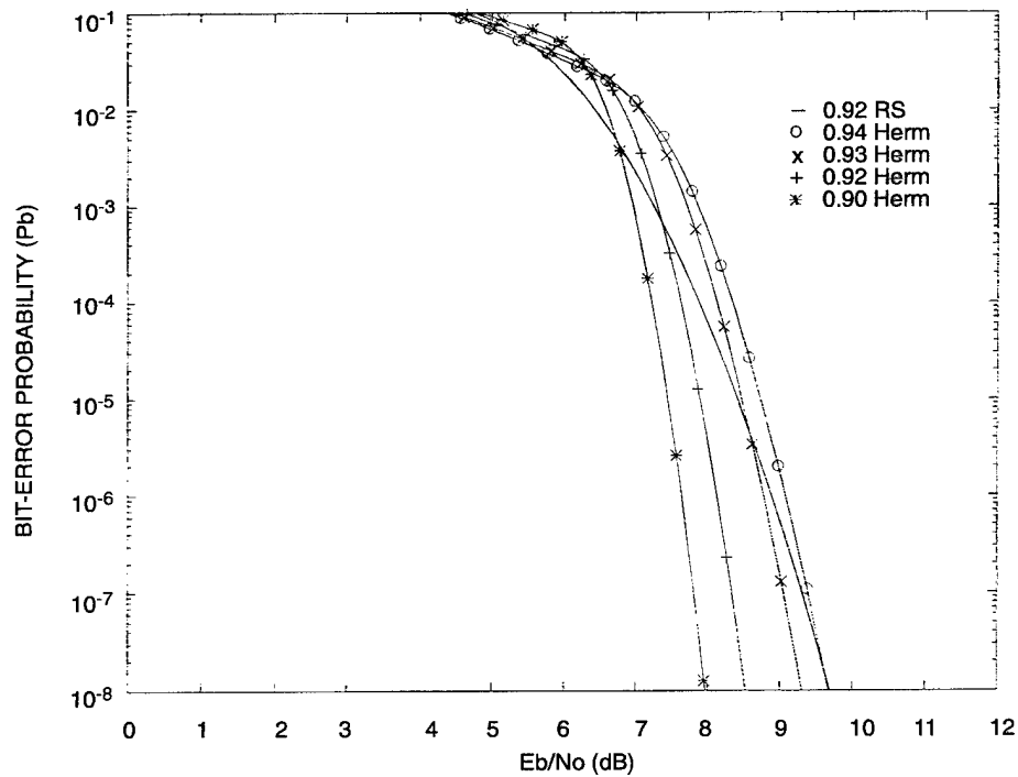
Figure 2. Bit-error probability versus SNR for low-rate RS code and selected Hermitian codes over F_{64} .
