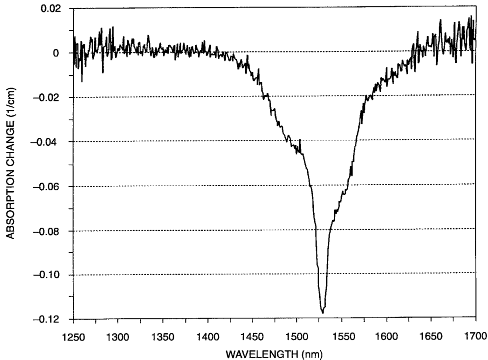
Figure 8. Absorption change vs. wavelength for a highly doped erbium filter.
