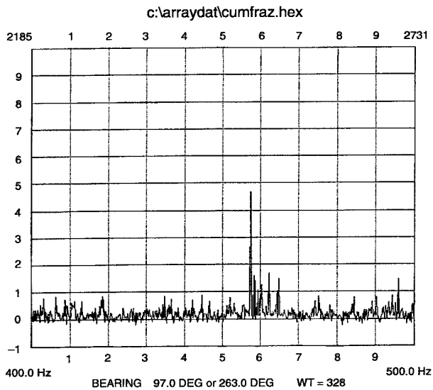
Figure 4. Normalized fourth cumulant for 457-Hz signal in quiet beam.
