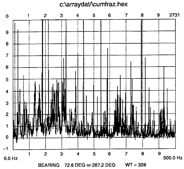
Figure 6. Normalized fourth cumulant for noisy beam.
