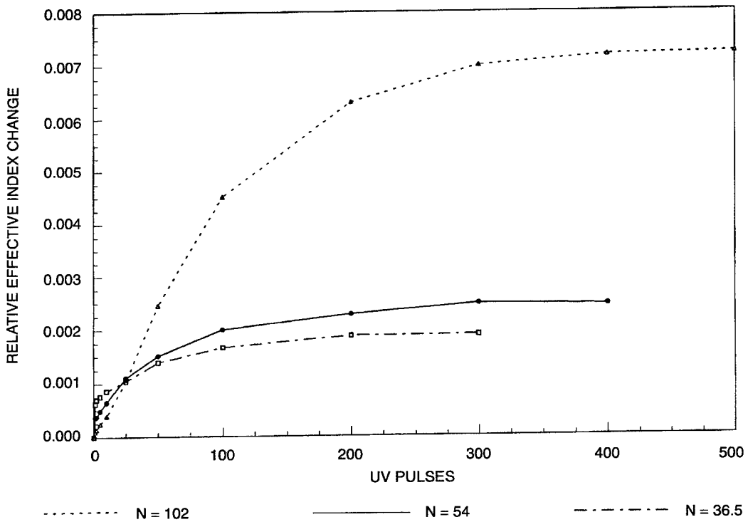
Figure 6. Effective index change vs. UV pulses for couplers with various coupled power cycles N: UV fluence of 242 mJ/cm².
