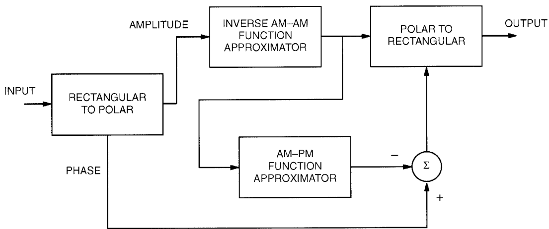
Figure 1. Model-based predistorter.
