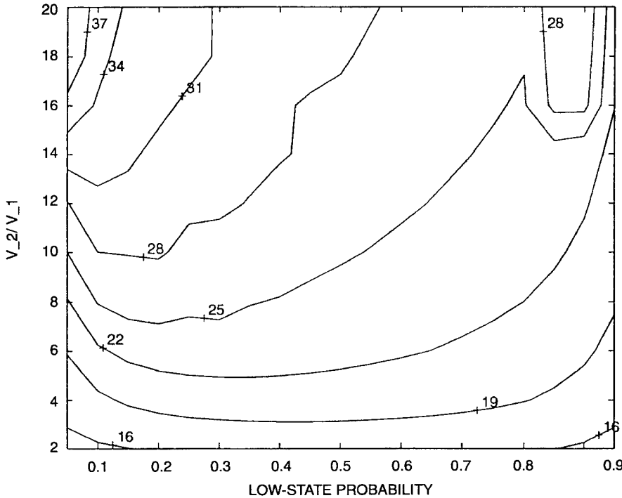
Figure 4. The signal gain (dB) of \mathcal{M}_{\mathcal{P}} over \mathcal{G}_{\mathcal{P}} .
