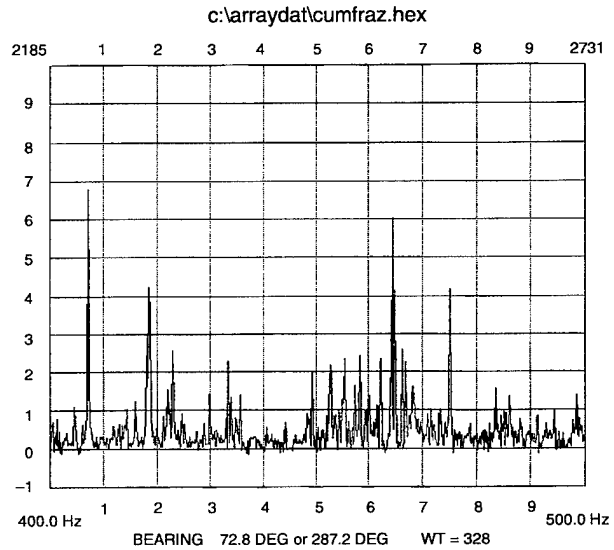
Figure 8. Normalized fourth cumulant for 400- to 500-Hz band in noisy beam.
