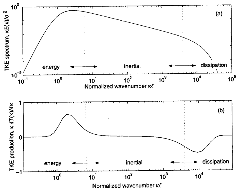
Figure 1: Three subranges of high-Reynolds-number turbulence. (a) Turbulent kinetic energy (TKE) spectrum, \kappa E(\kappa)/\sigma^2 . (b) TKE production spectrum, \kappa dT(\kappa)/d\kappa . (App A gives actual equations plotted here.)
