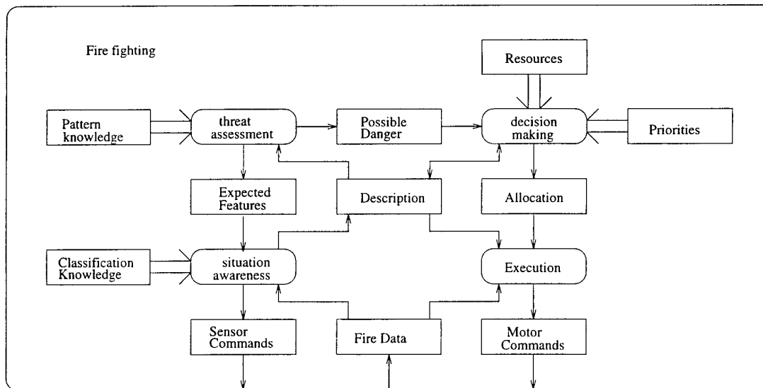
Fig. 4 Information and knowledge in the fire-fighting task. The rounded boxes denote (sub-)tasks; the square boxes information; the arrows data dependencies; and the double arrows knowledge dependencies.
