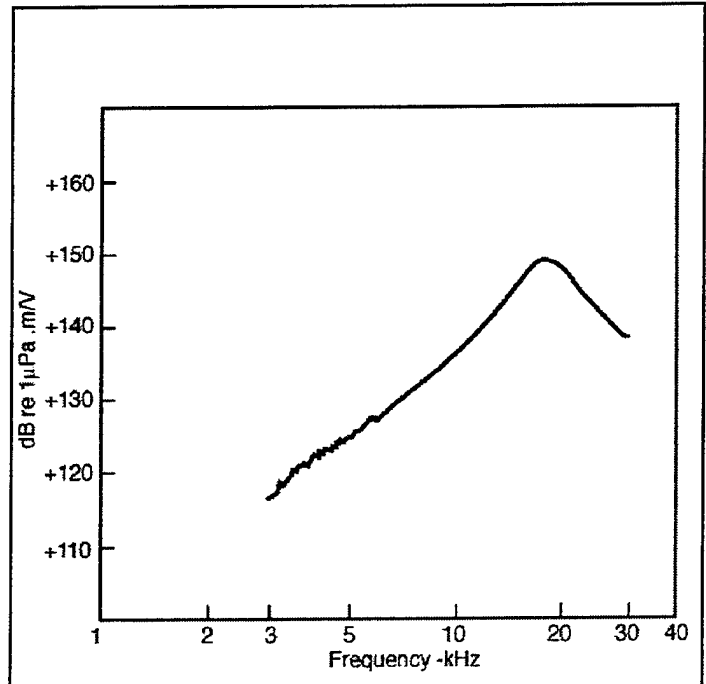
Figure A-2. ITC-1001 Projector voltage source level response.
