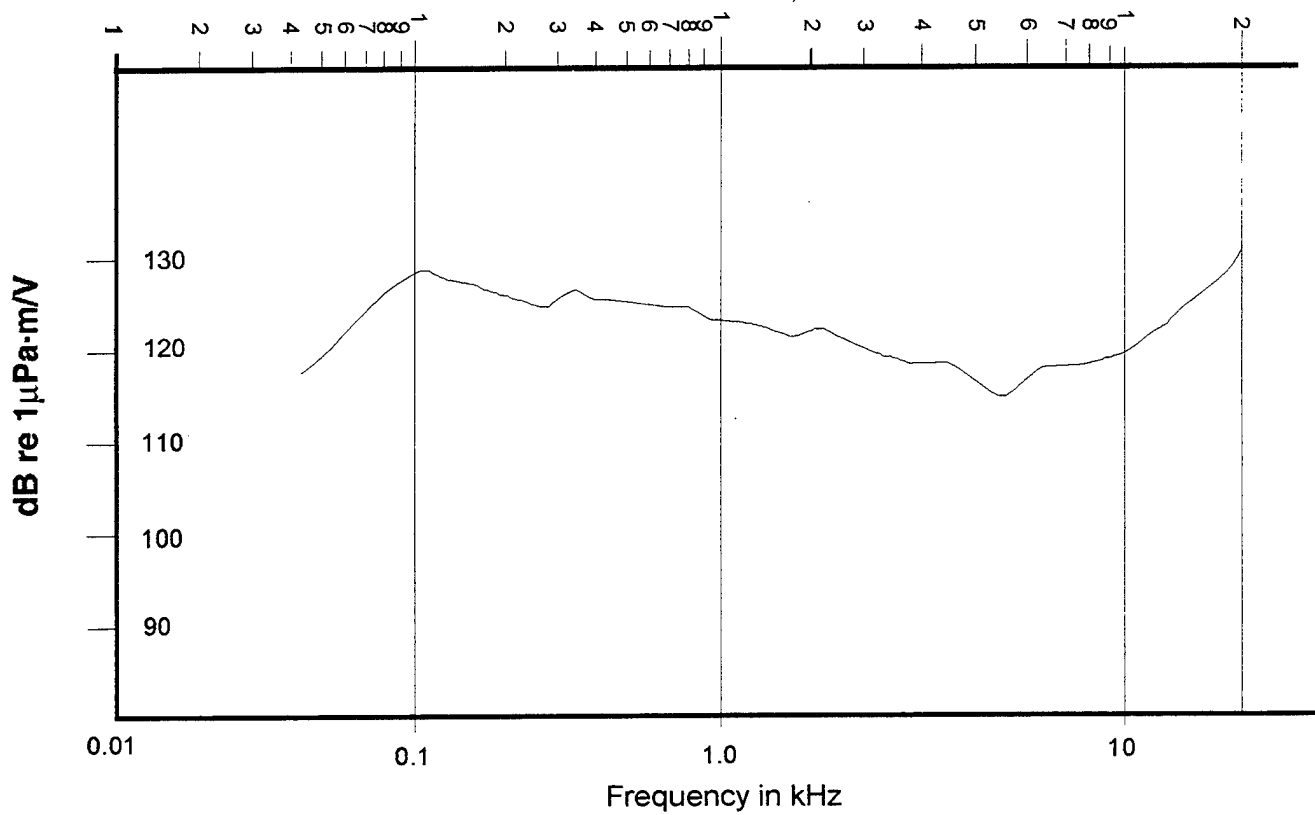
Figure A-6. J-9 Projector voltage source level response.
