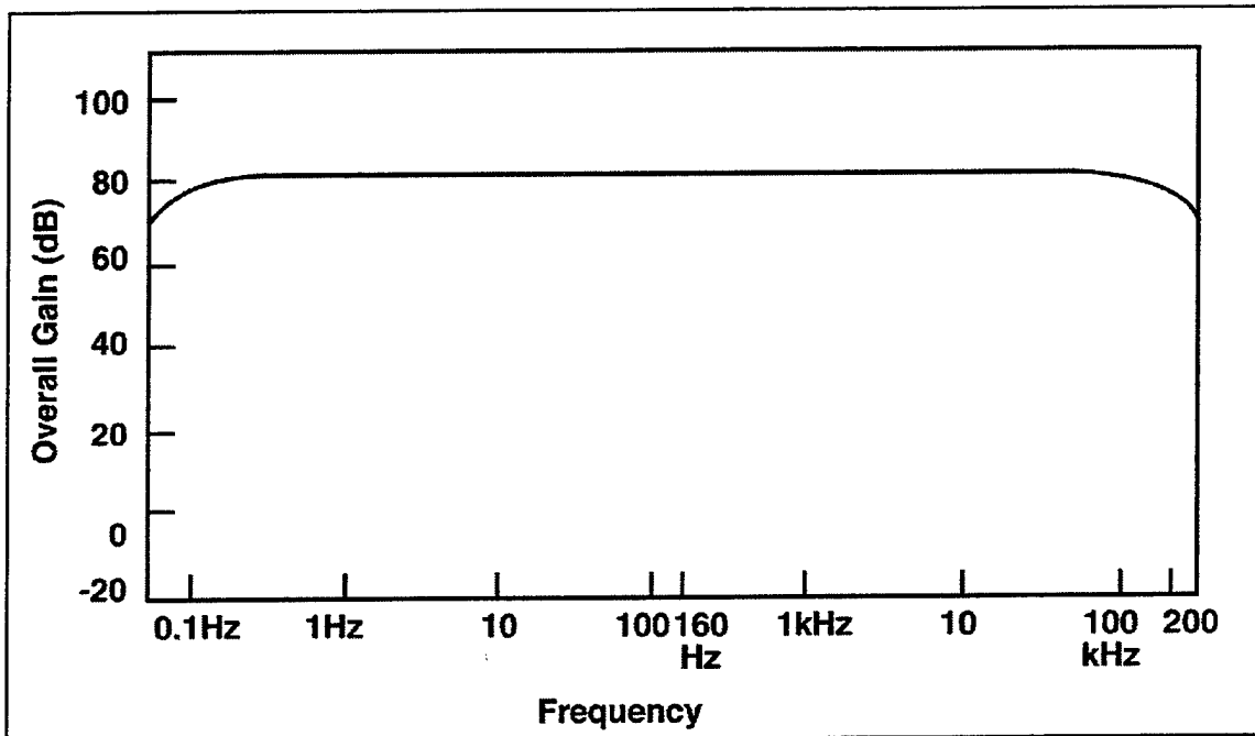
Figure A-8. Bruel & Kjaer 2635 Charge Amplifier frequency response.
