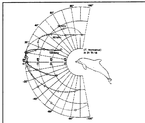
Figure 10b. Dolphin vertical received beam pattern. 9
