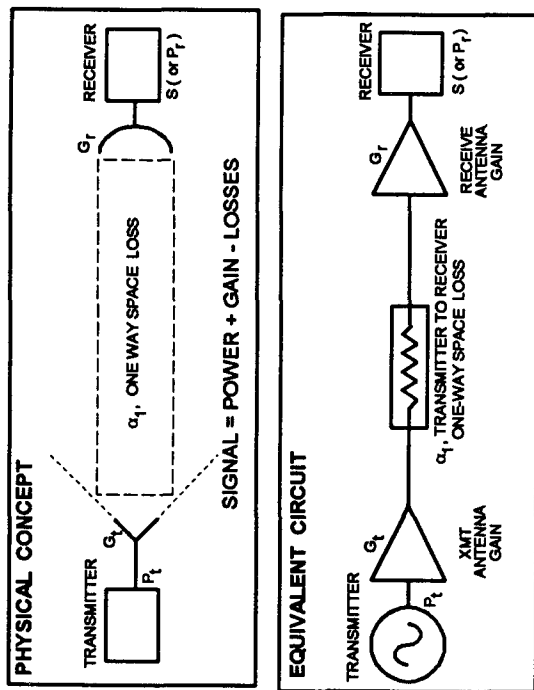
Figure 3. Concept of One-Way Space Loss
