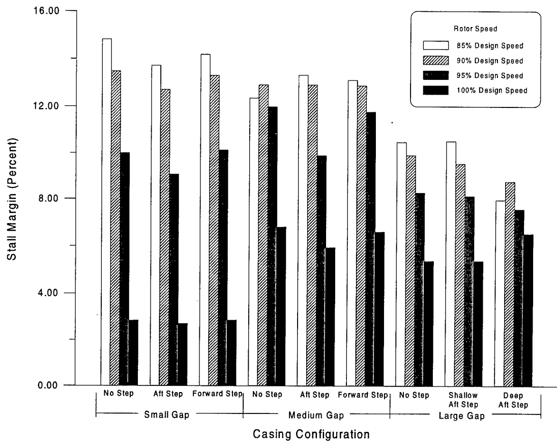
Figure 27. Stall Margin for Casing Configurations and Speeds
