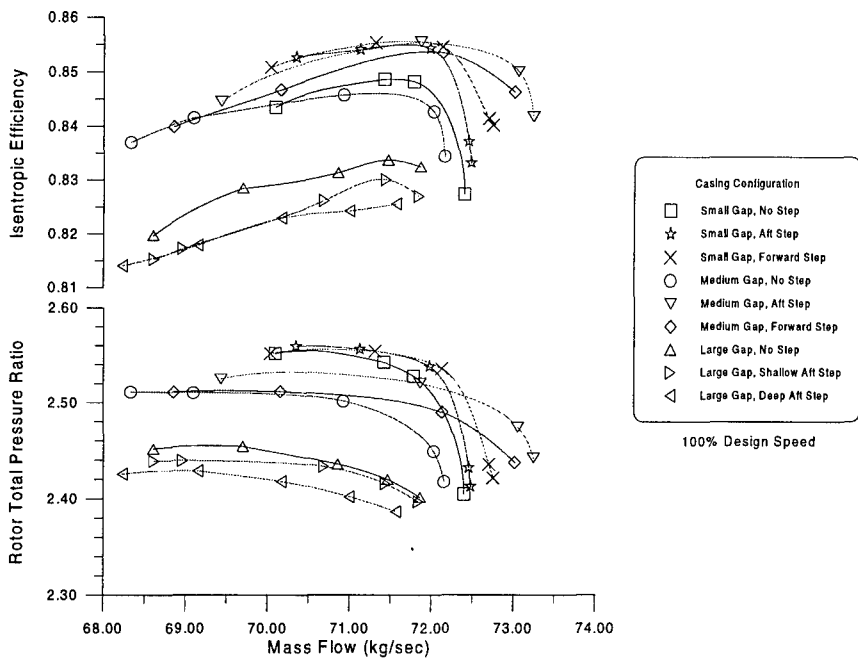
Figure 35. Rotor Map for 100% Design Speed
