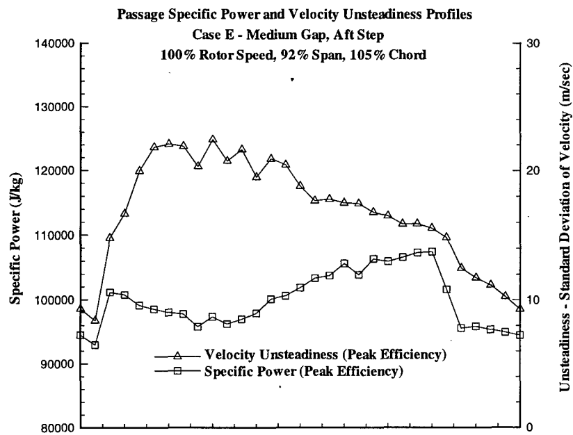
Figure 67. Power and Velocity Unsteadiness at Rotor Exit (Case E, 100% Design Rotor Speed)
