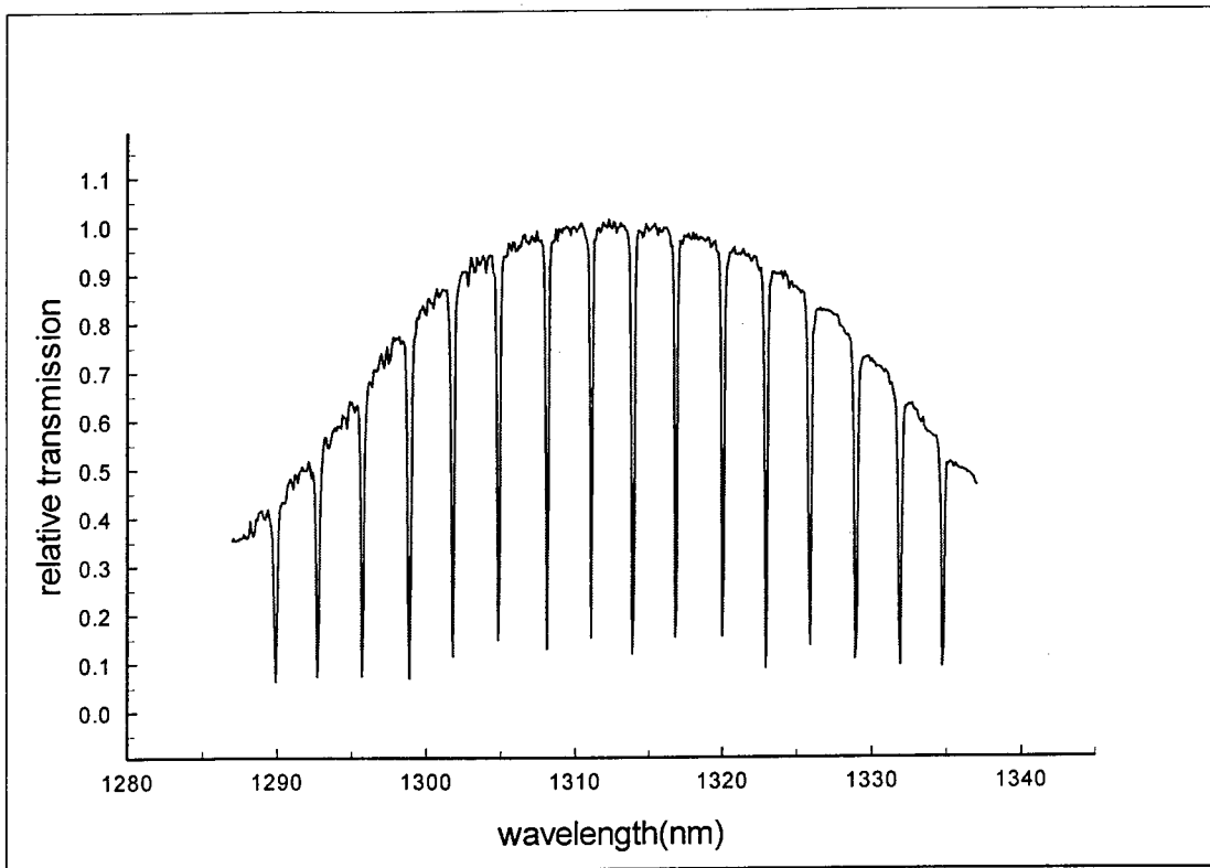
Figure 5-7. Transmission spectra of 16 grating fiber.
