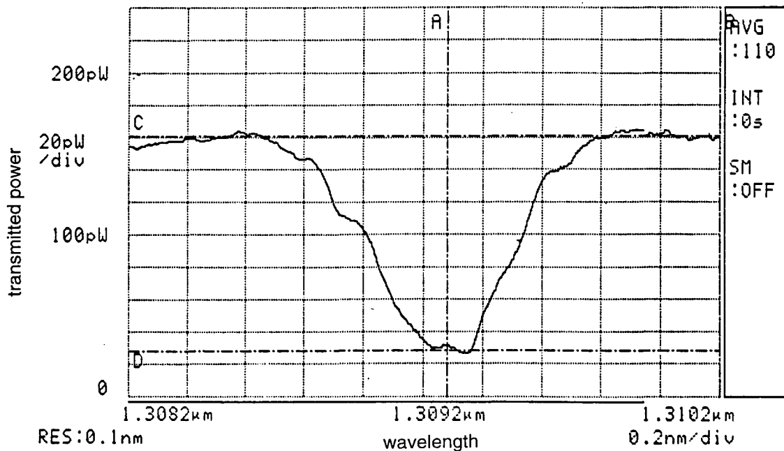
Figure 4-1. Bragg fiber grating transmission spectra of Andrews Series E polarization preserving fiber. R = 1 - (26 \text{ pW}) / (160 \text{ pW}) = 84\%
