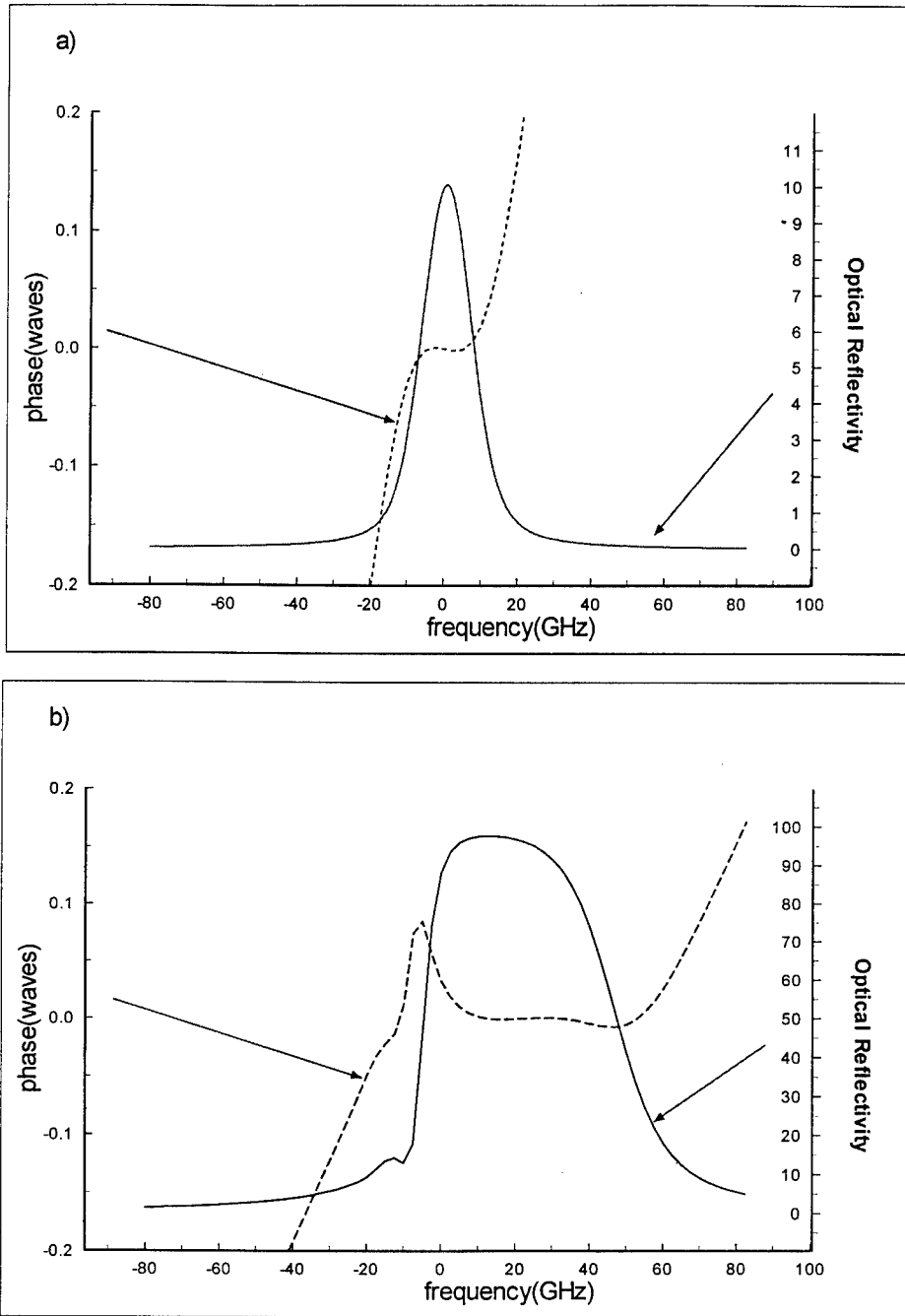
Figure 2-5. The optical response of weak a) and strong b) gratings shows a flat response over the useful portion of the gratings. The higher reflectivity of the strong gratings come at the expense of wide bandwidth and thus reduced channel isolation. The asymmetry of the strong grating is due to the grating chirp.
