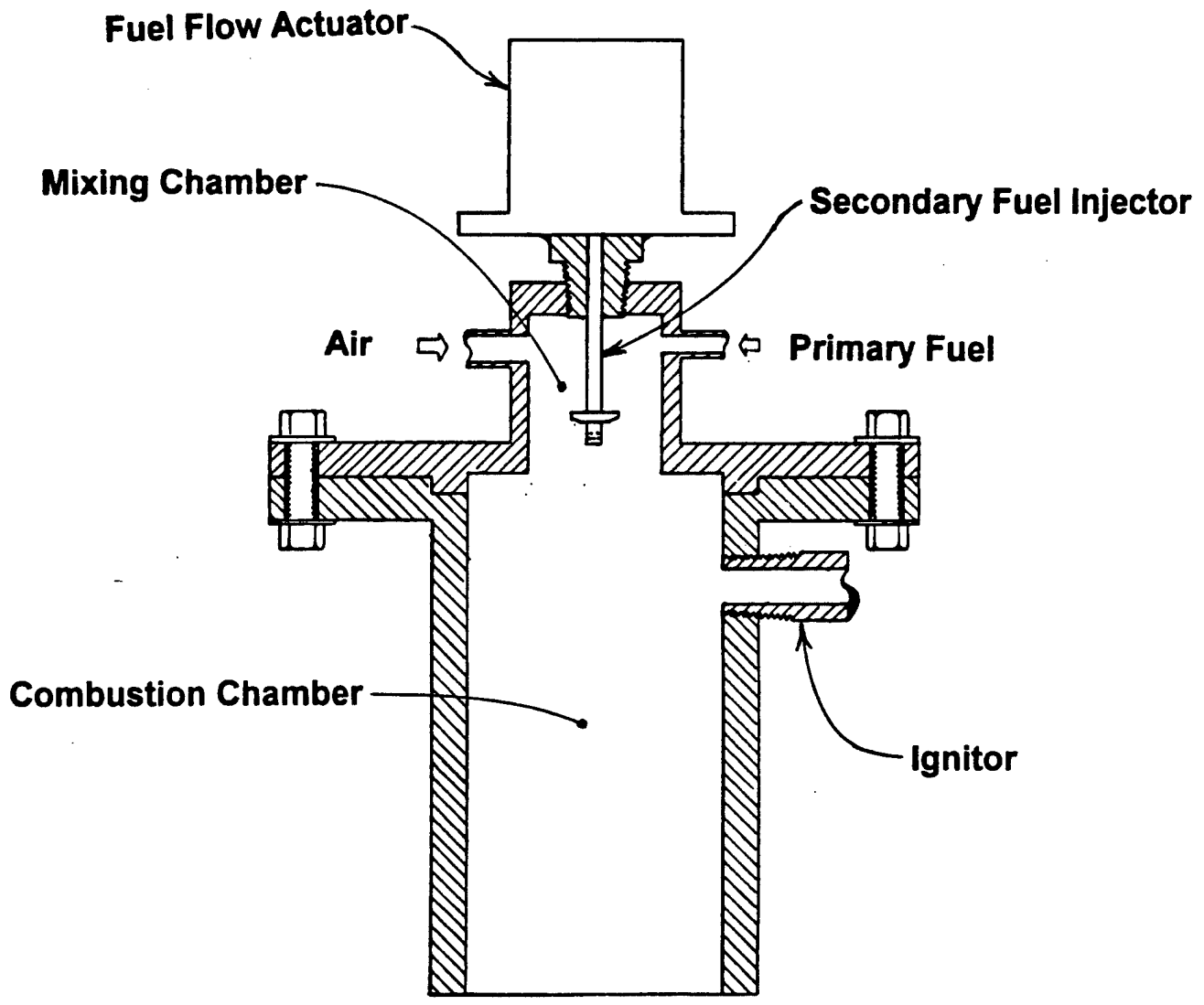
Figure 6. A schematic of the PFTD configured with the secondary fuel injector and actuator installed
