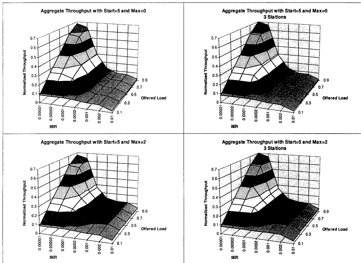
Figure H-5. Aggregate Throughput with Start=5 and Max=0 & 2
