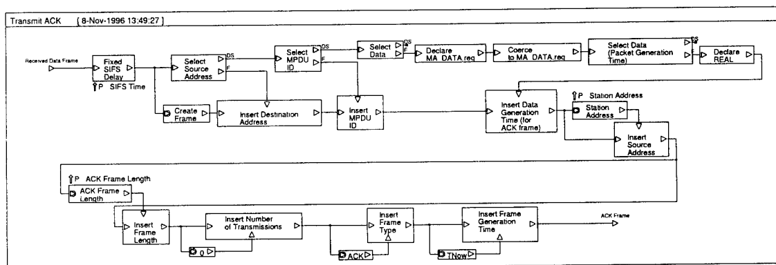
Figure A-25. Transmit ACK Simulation Module
