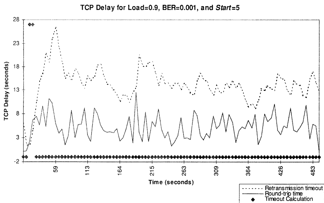
Figure G-10. TCP Delay for Load=0.9, BER=0.001, and Start=5
