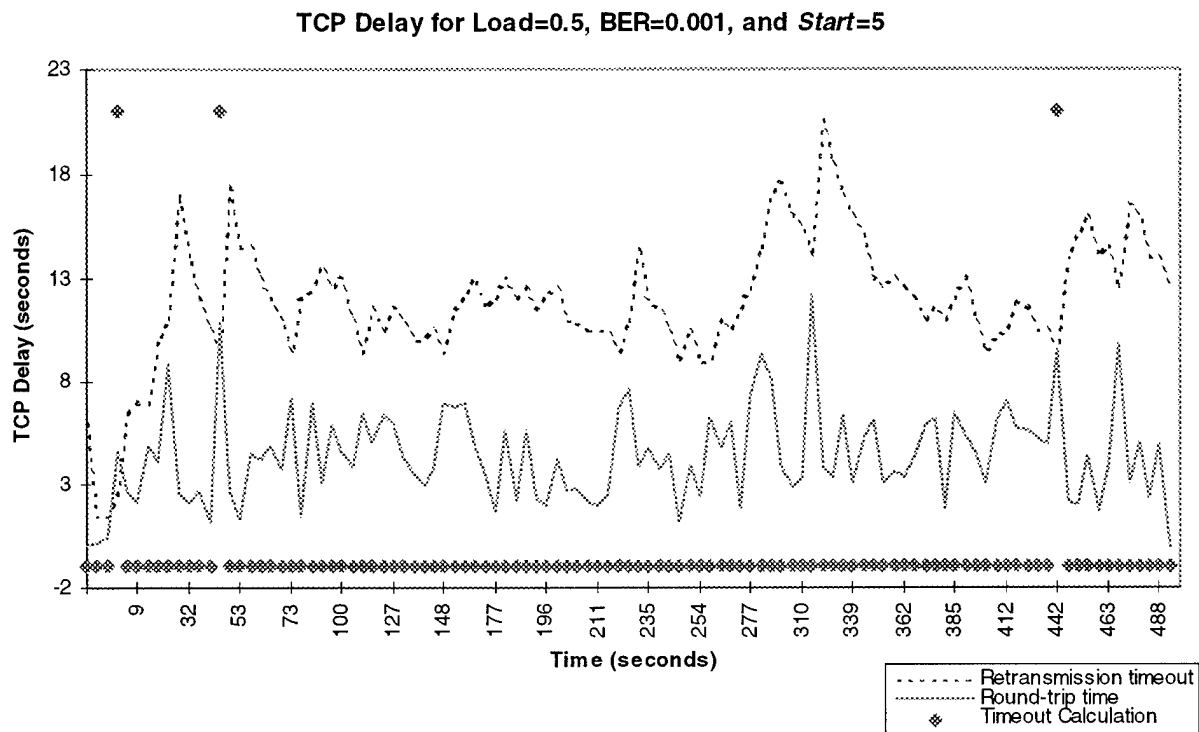
Figure 6-18. TCP Delay for Load=0.5, BER=0.001, and Start=5
