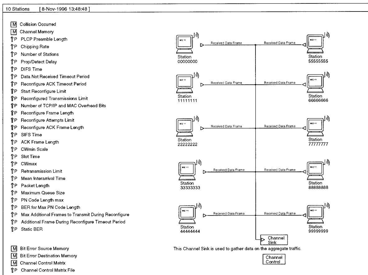
Figure 5-1. 10 Stations Simulation Module
