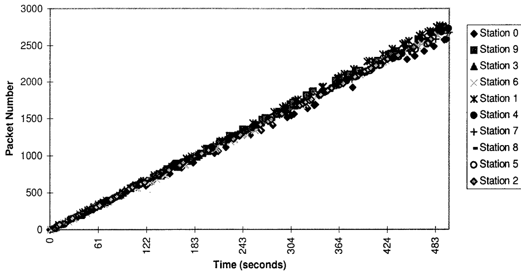
Figure F-11. System Fairness for Load=0.5, BER=0.00001, and Start =5
