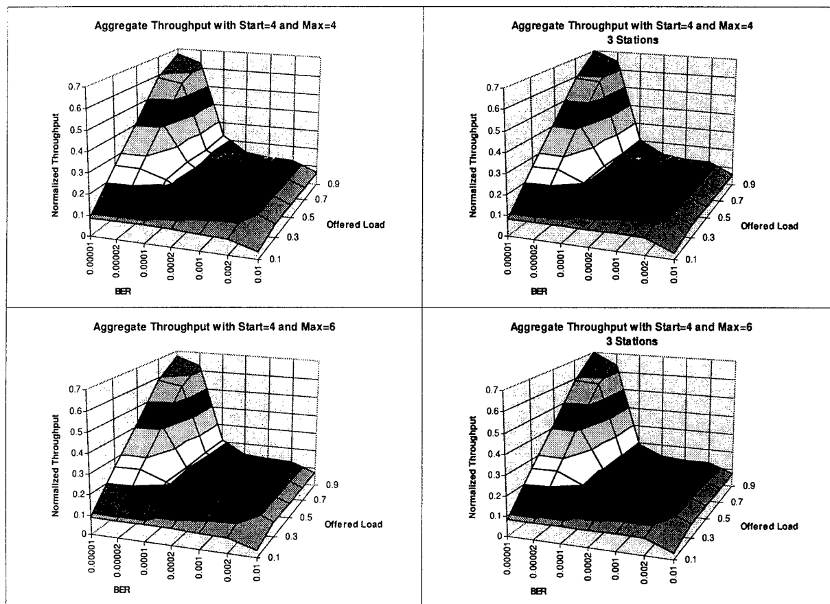
Figure H-4. Aggregate Throughput with Start=4 and Max=4 & 6
