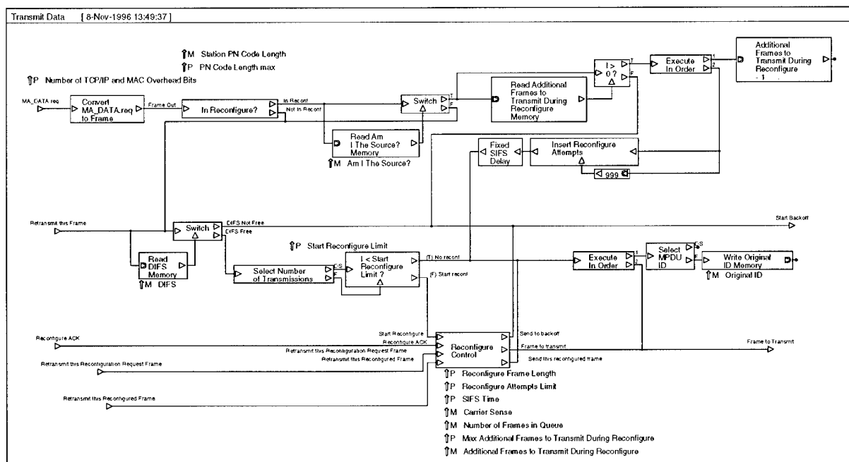
Figure 5-5. Transmit Data Simulation Module
