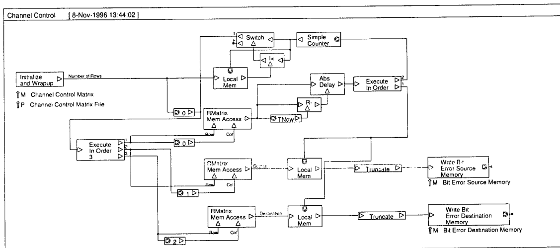
Figure A-8. Channel Control Simulation Module
