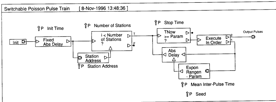
Figure A-23. Switchable Poisson Pulse Train Simulation Module
