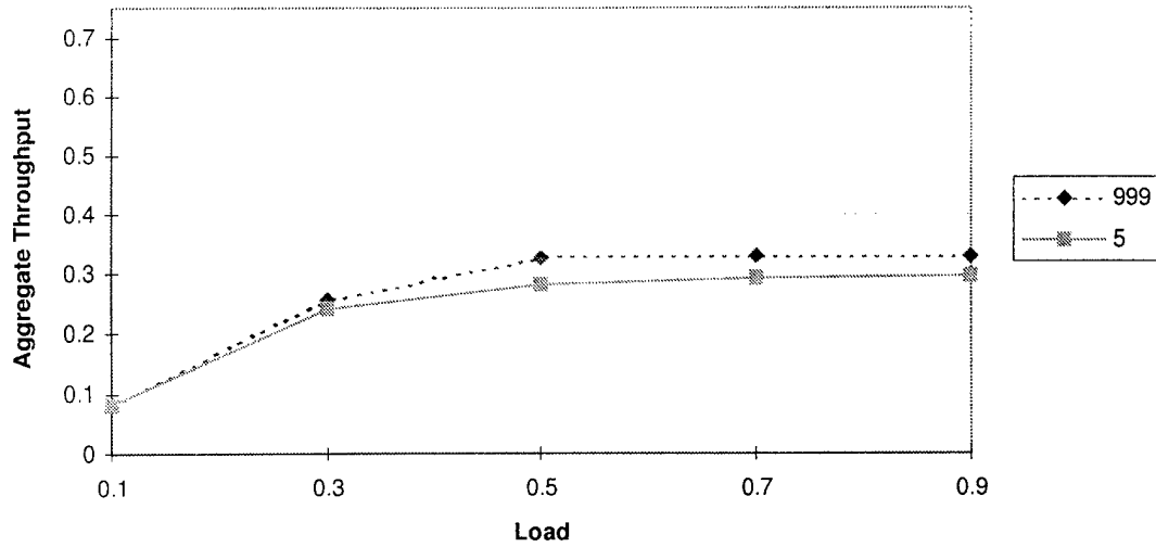
Figure E-5. Throughput for Gilbert Errors ( P=0.0001 , p=0.01 , and 1-h=0.2 )
