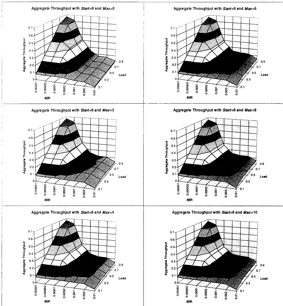
Figure B-6. Aggregate Throughput with Start=8 for 10 Station Simulation
