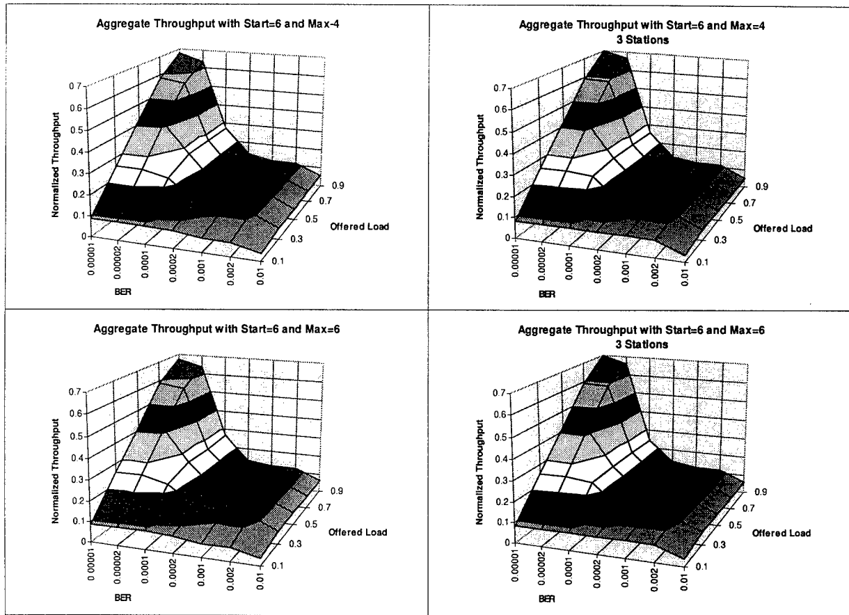
Figure H-8. Aggregate Throughput with Start=6 and Max=4 & 6
