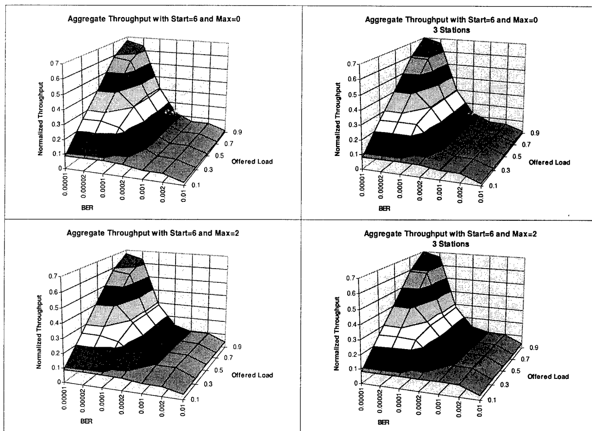
Figure H-7. Aggregate Throughput with Start=6 and Max=0 & 2
