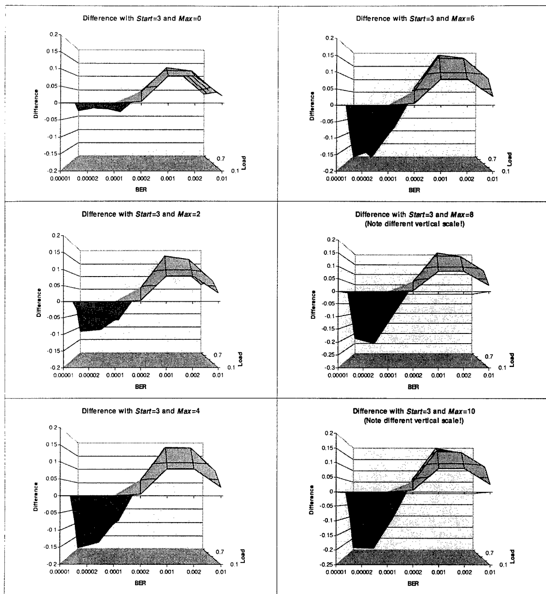
Figure D-1. Difference Plots with Start=3
