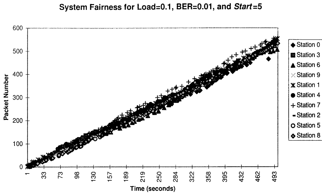
Figure F-1. System Fairness for Load=0.1, BER=0.01, and Start =5
