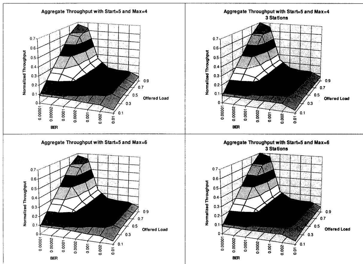
Figure H-6. Aggregate Throughput with Start=5 and Max=4 & 6
