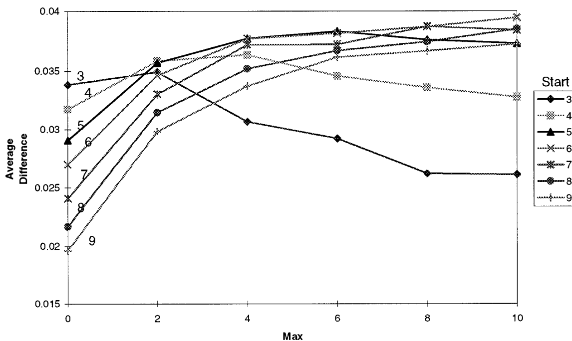
Figure 6-7. Average Difference for Values of Start and Max
