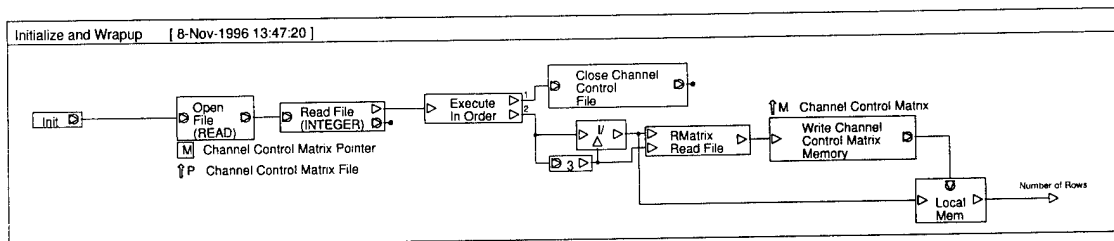
Figure A-18. Initialize and Wrapup Simulation Module
