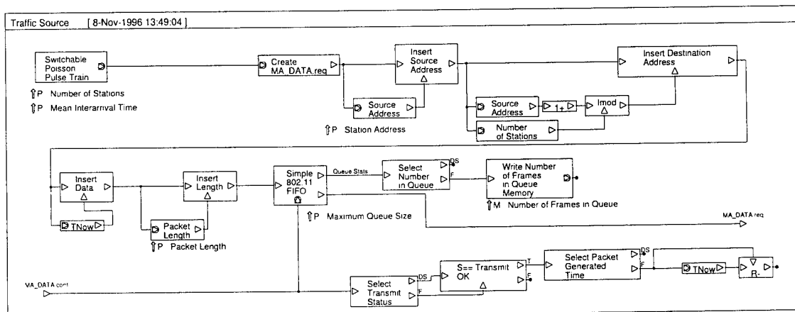
Figure A-24. Traffic Source Simulation Module
