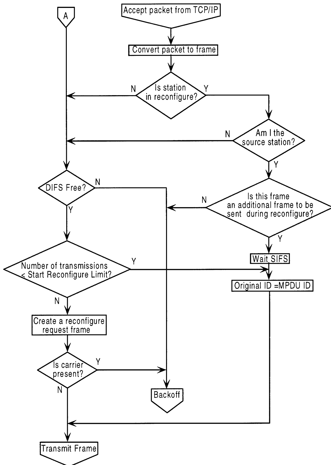
Figure 4-4. Process Packet Transmission Request from TCP/IP Flowchart
