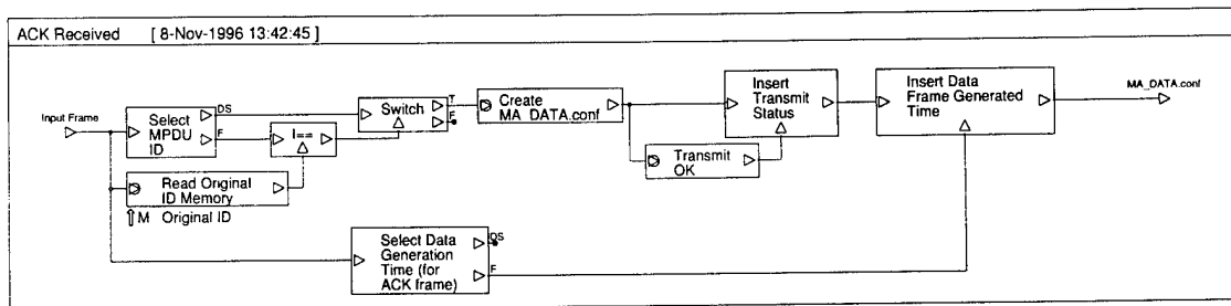
Figure A-2. ACK Received Simulation Module
