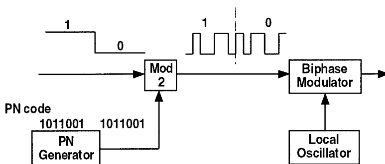
Figure 2-8. Direct Sequence Spread Spectrum Transmitter
