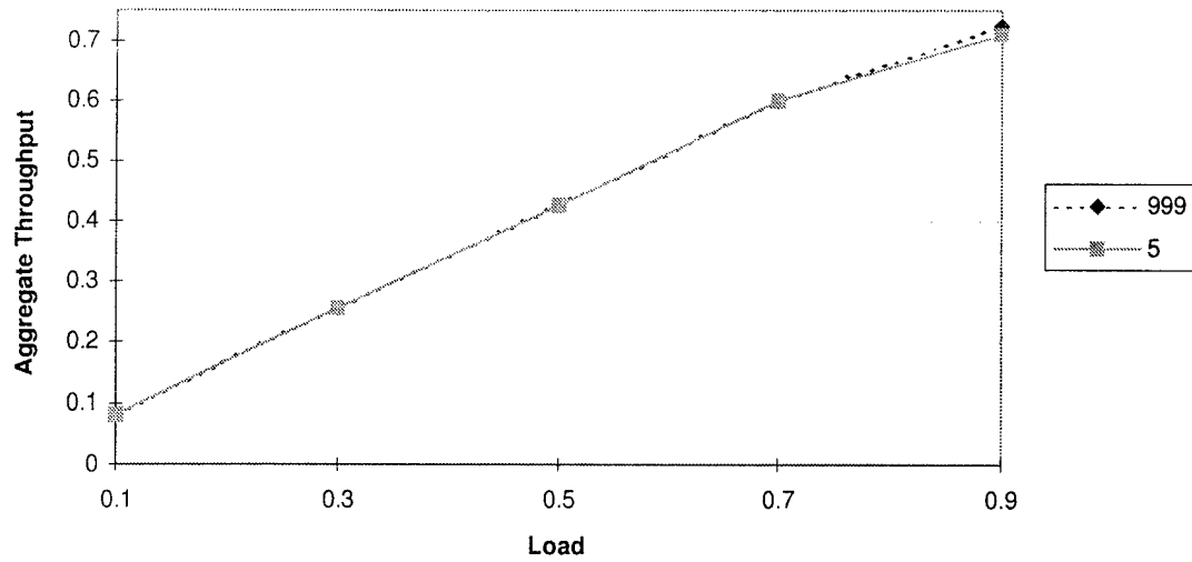
Figure E-9. Throughput for Gilbert Errors ( P=0.000001 , p=0.01 , and 1-h=0.2 )
