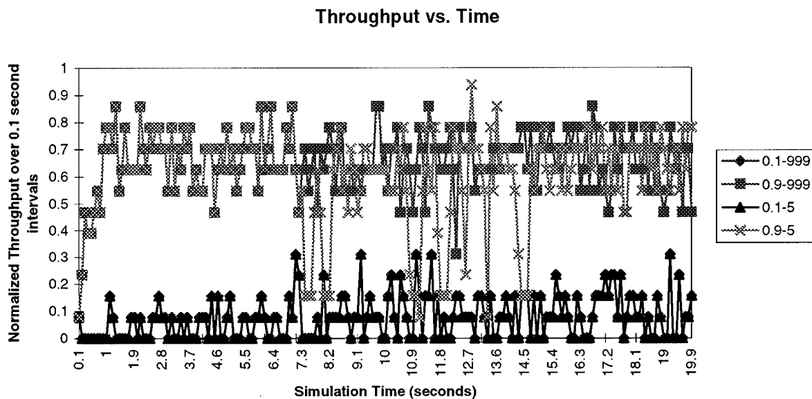
Figure 5-11. Normalized Throughput versus Time over 0.1 second intervals (Start=5 and 999 Load=0.1 and 0.9)
