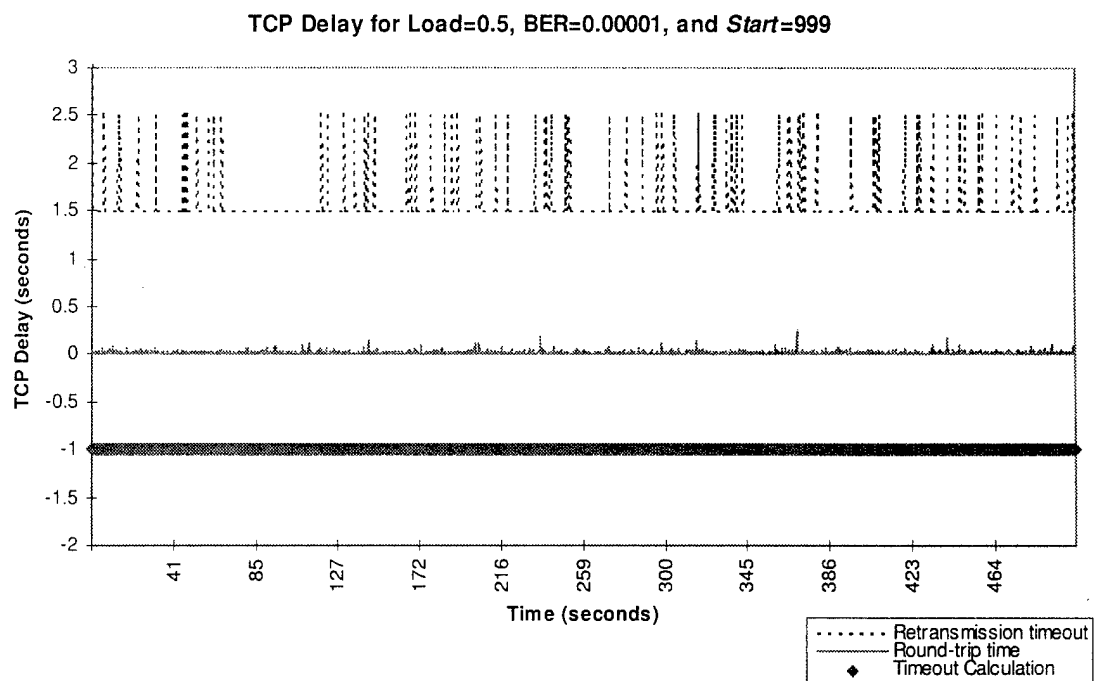
Figure G-16. TCP Delay for Load=0.5, BER=0.00001, and Start=999
