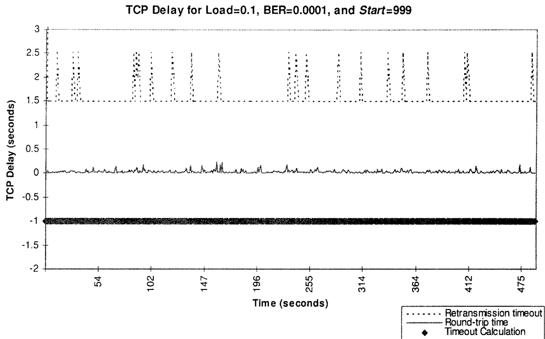
Figure G-13. TCP Delay for Load=0.1, BER=0.0001, and Start=999
