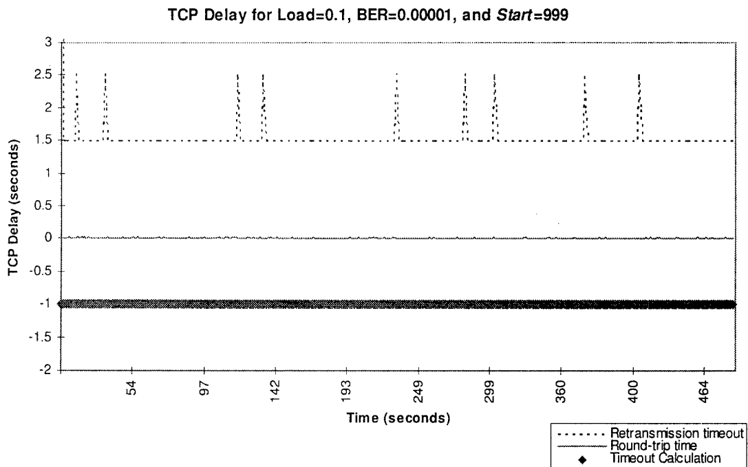
Figure G-14. TCP Delay for Load=0.1, BER=0.00001, and Start=999
