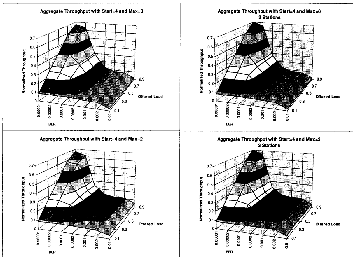
Figure H-3. Aggregate Throughput with Start=4 and Max=0 & 2
