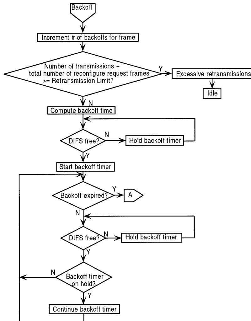
Figure 4-7. Backoff Flowchart
