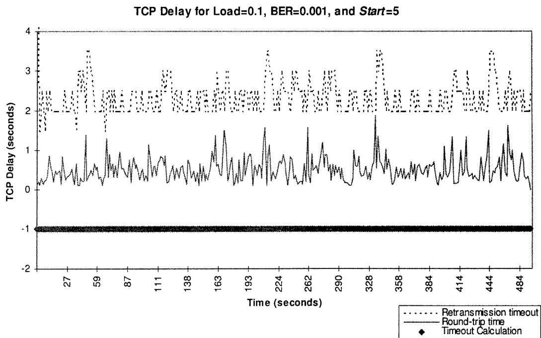
Figure G-2. TCP Delay for Load=0.1, BER=0.001, and Start =5
