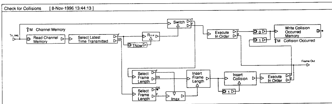
Figure A-9. Check for Collisions Simulation Module
