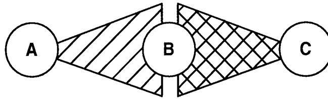
Figure 2-19. Hidden Terminal Situation
