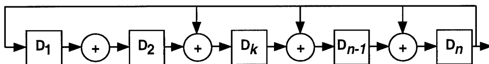
Figure 2-9. Modular Multiple-Tap Sequence Generator [Dix94]
