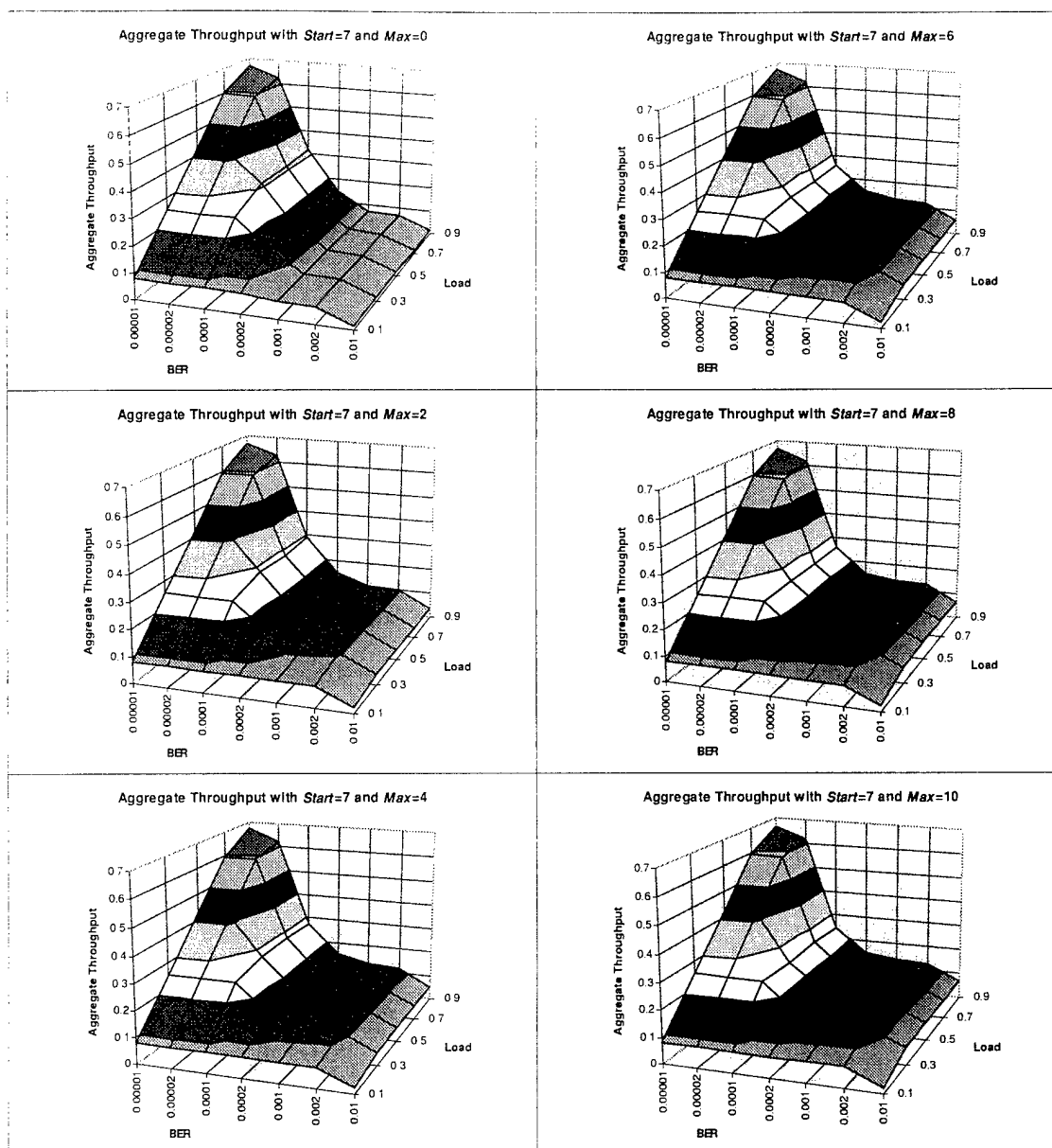
Figure B-5. Aggregate Throughput with Start=7 for 10 Station Simulation
