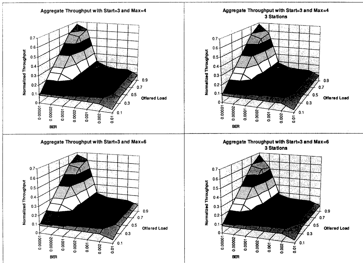
Figure H-2. Aggregate Throughput with Start=3 and Max=4 & 6
