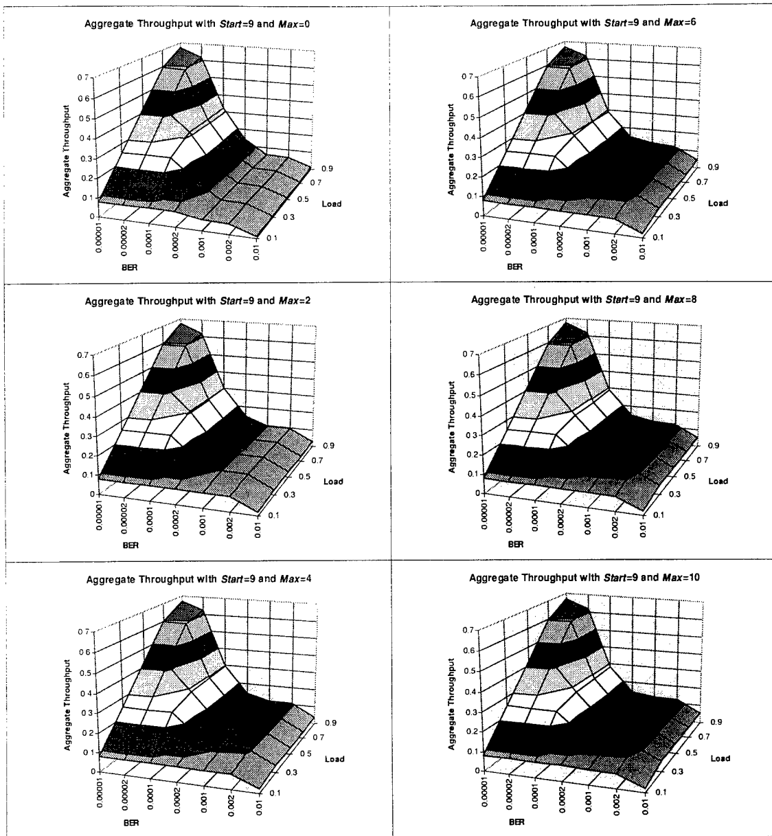
Figure B-7. Aggregate Throughput with Start=9 for 10 Station Simulation
