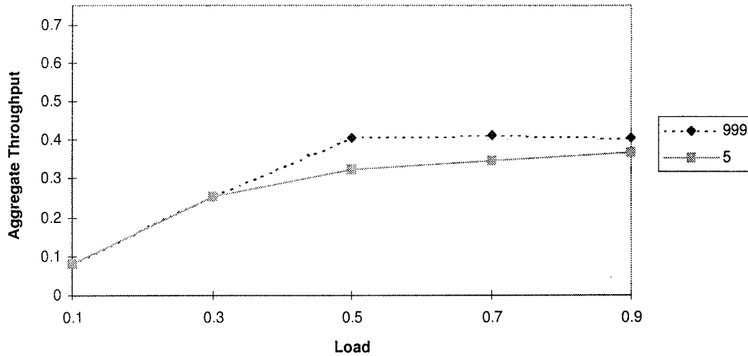
Figure E-3. Throughput for Gilbert Errors ( P=0.0001 , p=0.1 , and 1-h=0.2 )
