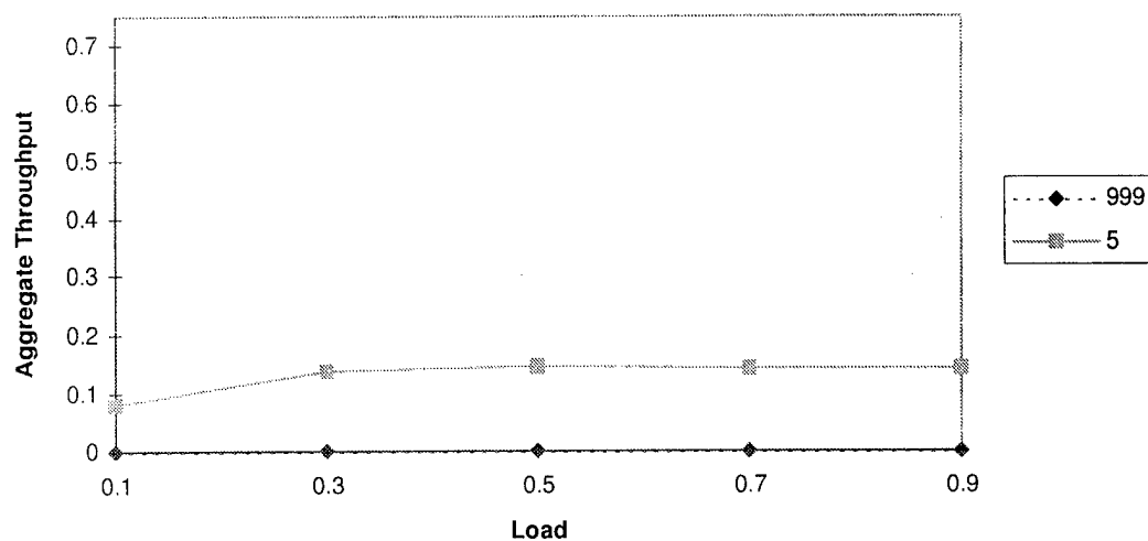
Figure E-1. Throughput for Gilbert Errors ( P=0.001 , p=0.1 , and 1-h=0.2 )
