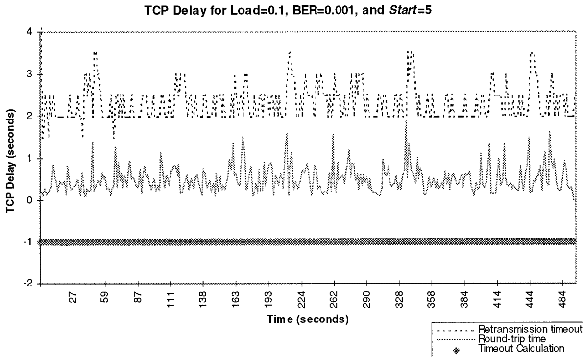
Figure 6-17. TCP Delay for Load=0.1, BER=0.001, and Start =5
