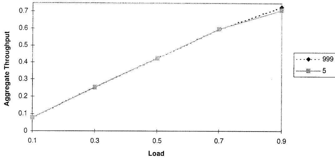
Figure E-7. Throughput for Gilbert Errors ( P=0.000001 , p=0.1 , and 1-h=0.2 )
