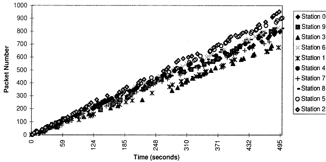
Figure F-13. System Fairness for Load=0.9, BER=0.01, and Start =5
