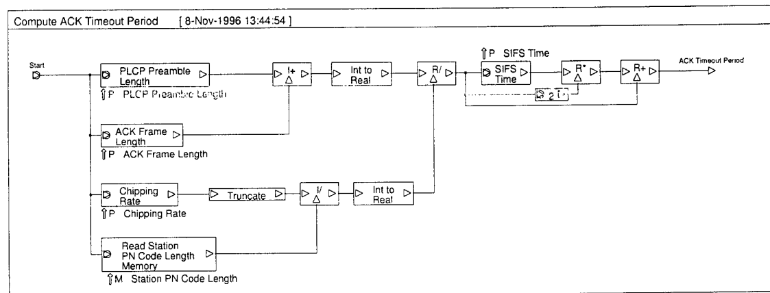
Figure A-11. Compute ACK Timeout Period Simulation Module
