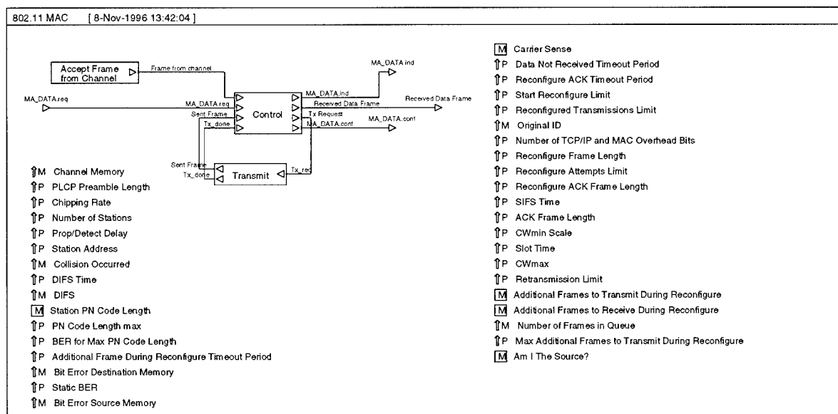
Figure 5-3. 802.11 MAC Simulation Module
