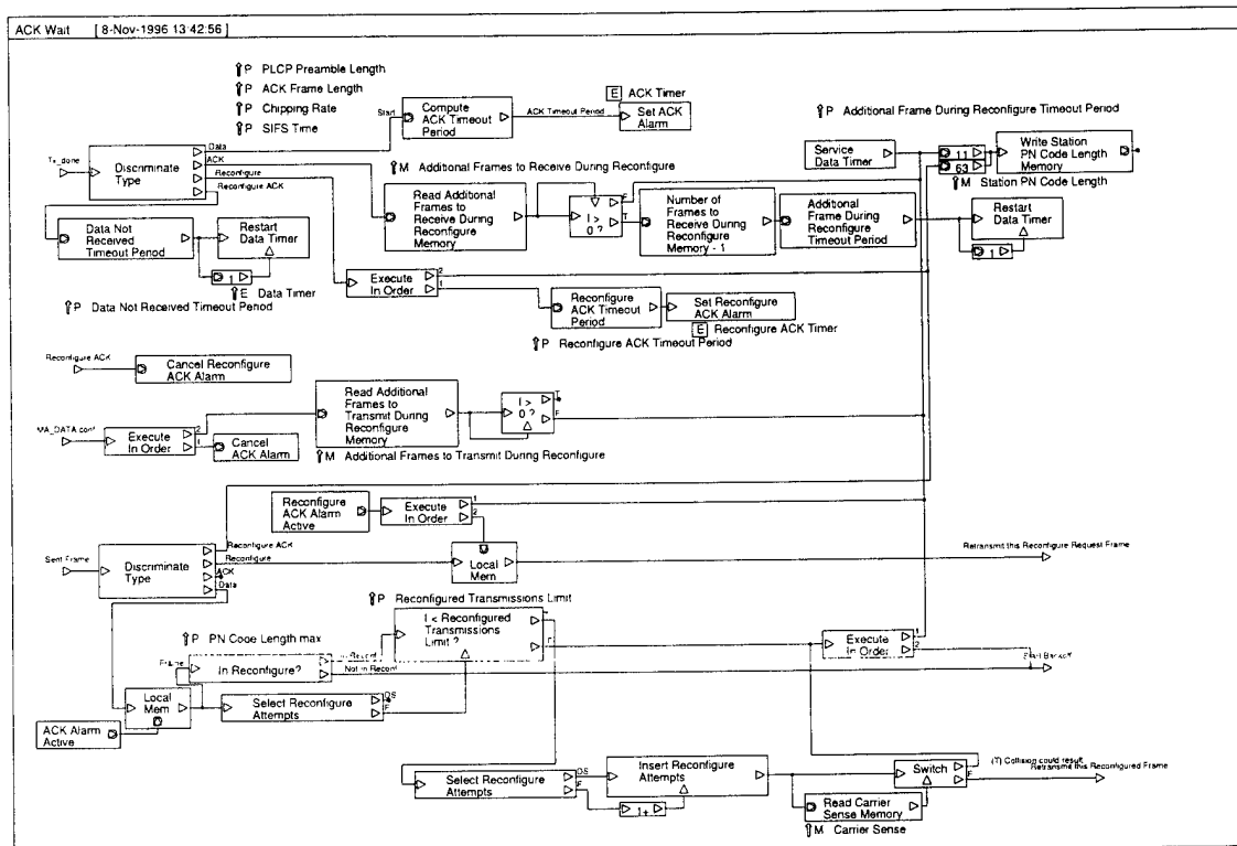
Figure A-3. ACK Wait Simulation Module
