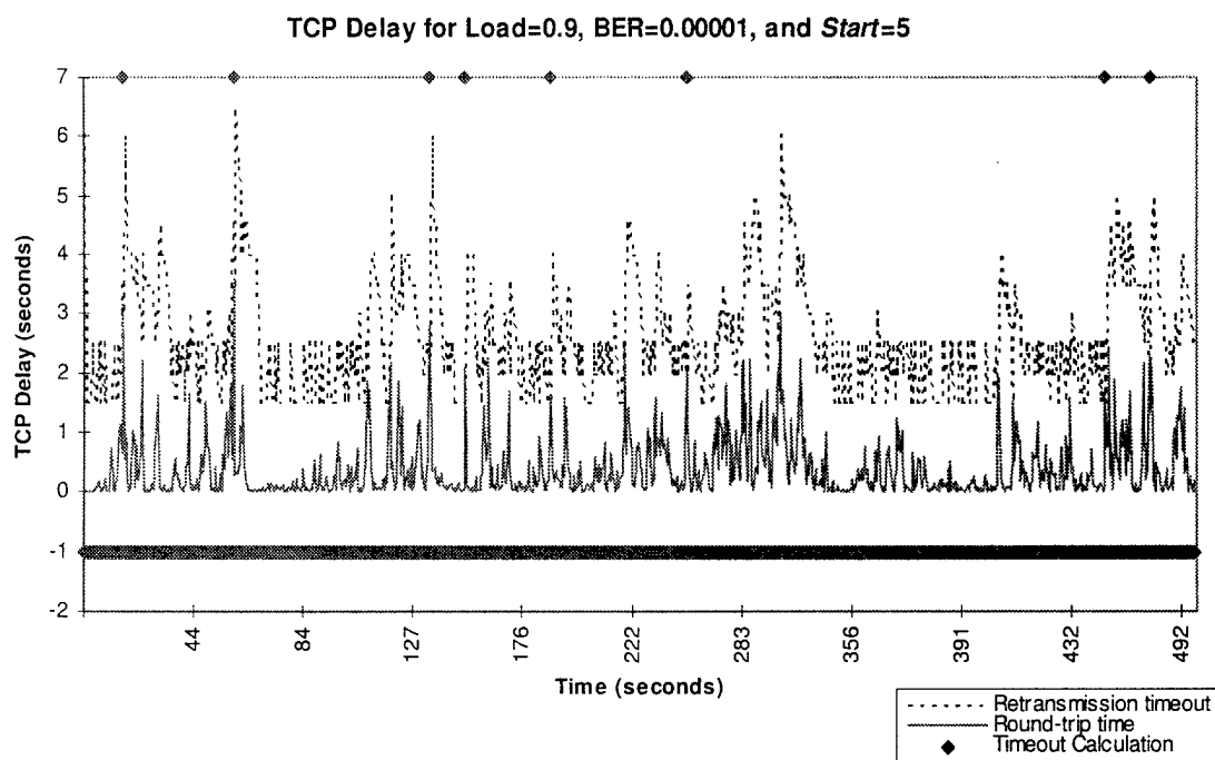
Figure G-12. TCP Delay for Load=0.9, BER=0.00001, and Start=5
