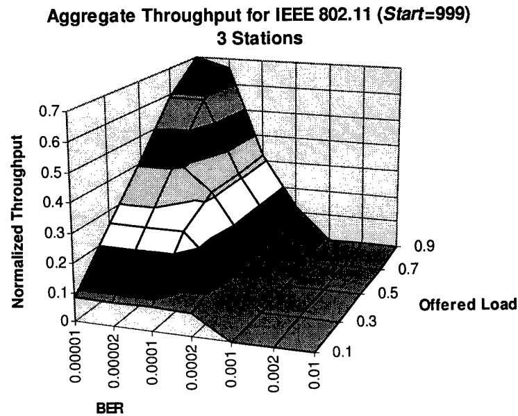
Figure 7-5. Three Station Simulation Results for IEEE 802.11
