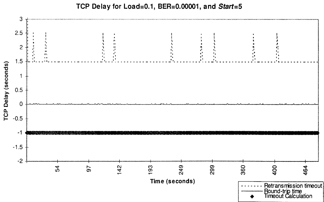
Figure G-4. TCP Delay for Load=0.1, BER=0.00001, and Start =5
