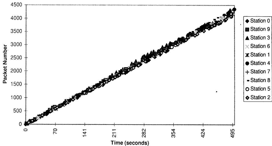
Figure F-18. System Fairness for Load=0.9, BER=0.00001, and Start =999
