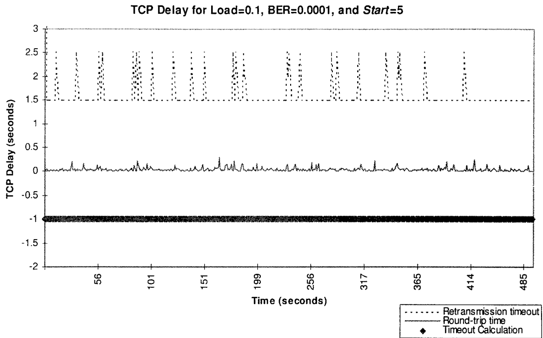
Figure G-3. TCP Delay for Load=0.1, BER=0.0001, and Start =5
