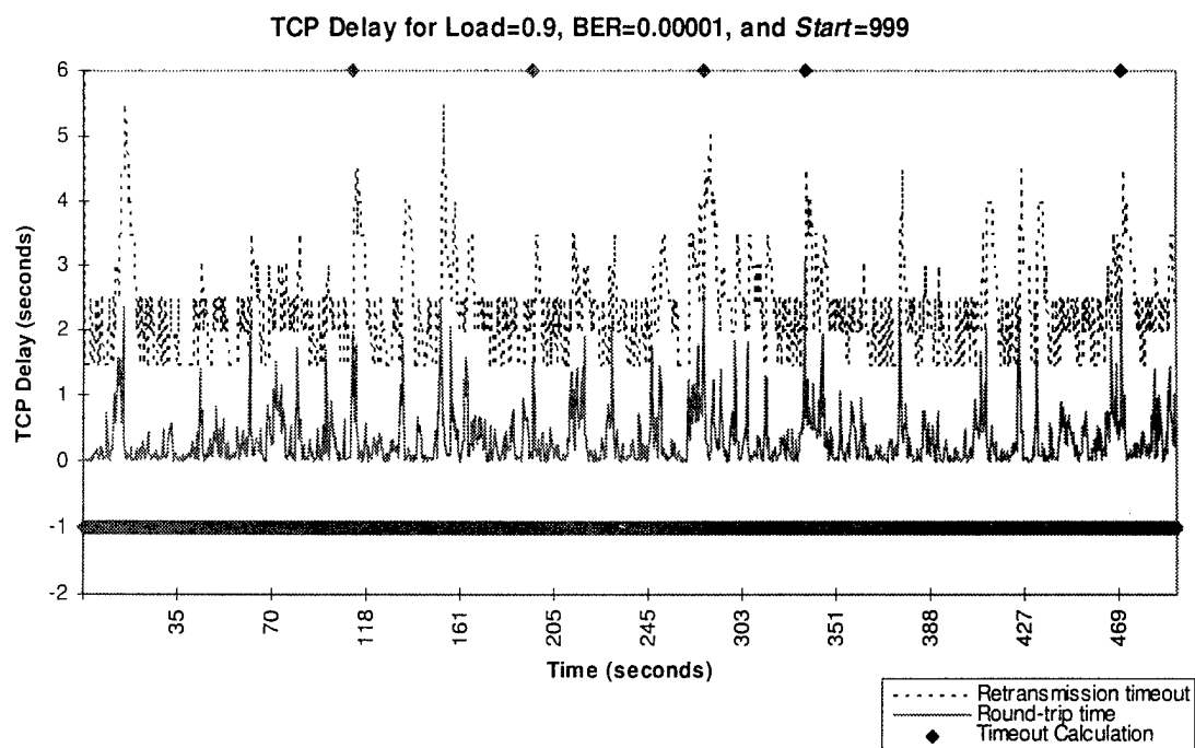
Figure G-18. TCP Delay for Load=0.9, BER=0.00001, and Start=999
