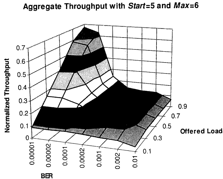
Figure 7-8. CATER Emulation Results when Start =5 and Max =6
