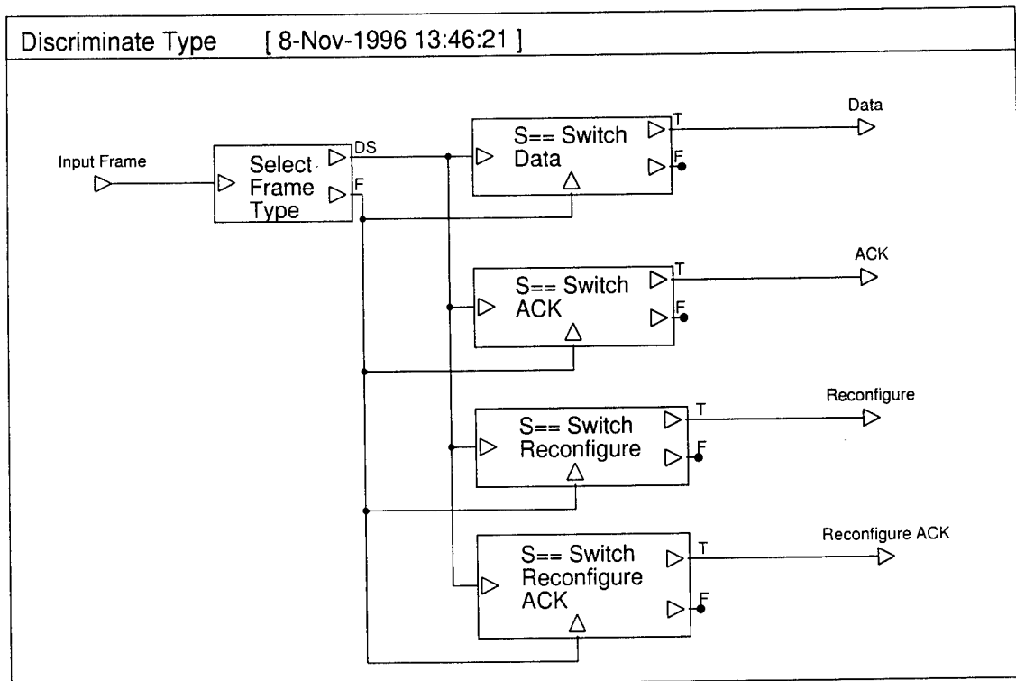
Figure A-16. Discriminate Type Simulation Module
