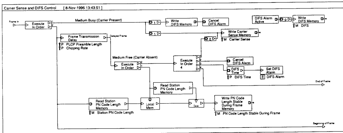
Figure A-7. Carrier Sense and DIFS Control Simulation Module
