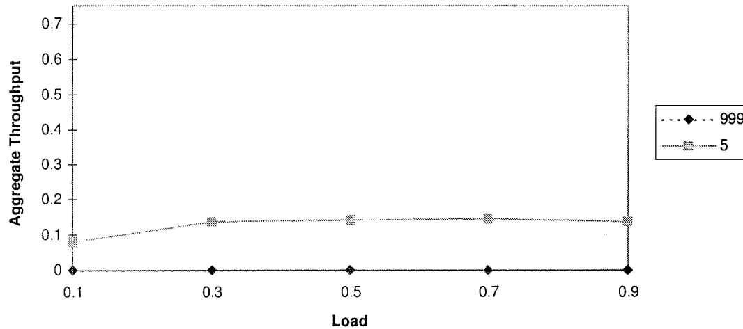
Figure E-2. Throughput for Gilbert Errors ( P=0.001 , p=0.1 , and 1-h=0.8 )
