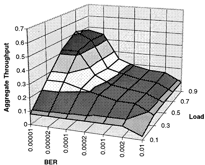
Figure 7-2. Ten Station Simulation Results
