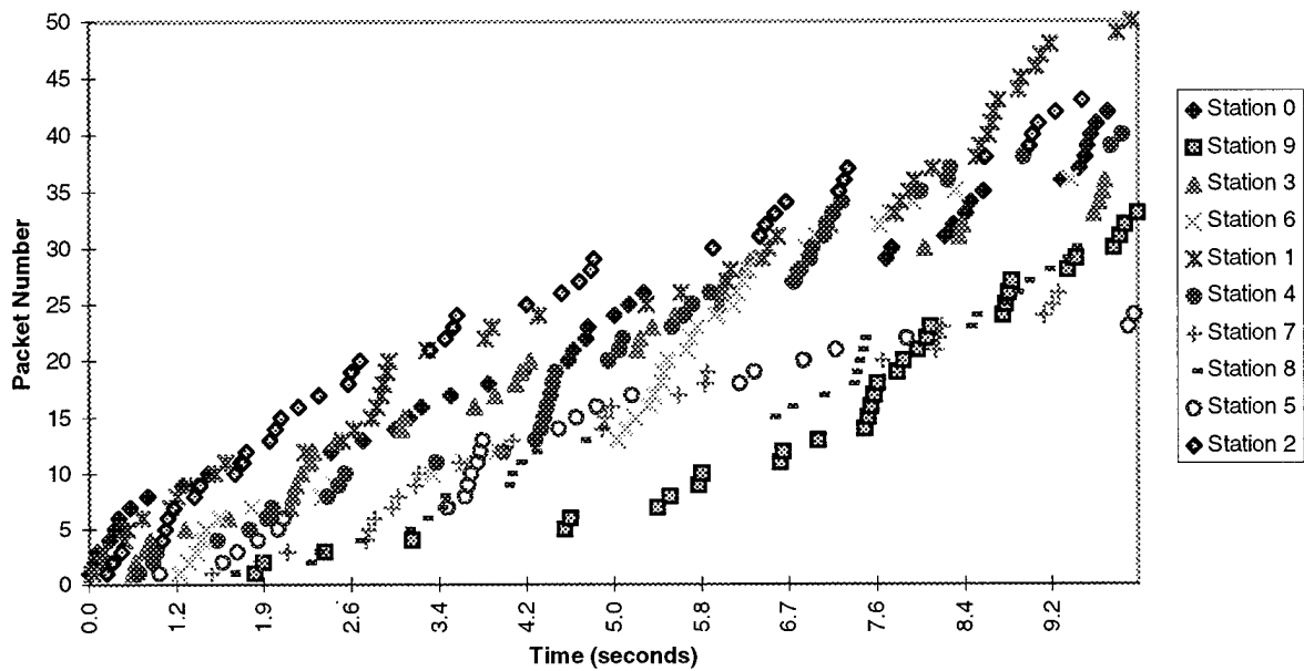
Figure 6-15. Microscopic View of System Fairness (Load=0.5, BER=0.0001, and Start=999)
