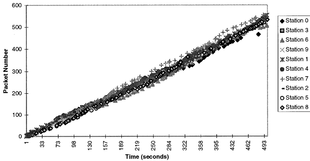
Figure 6-12. System Fairness for Load=0.1, BER=0.01, and Start =5
