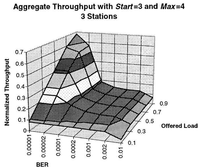
Figure 7-3. Three Station Simulation Results
