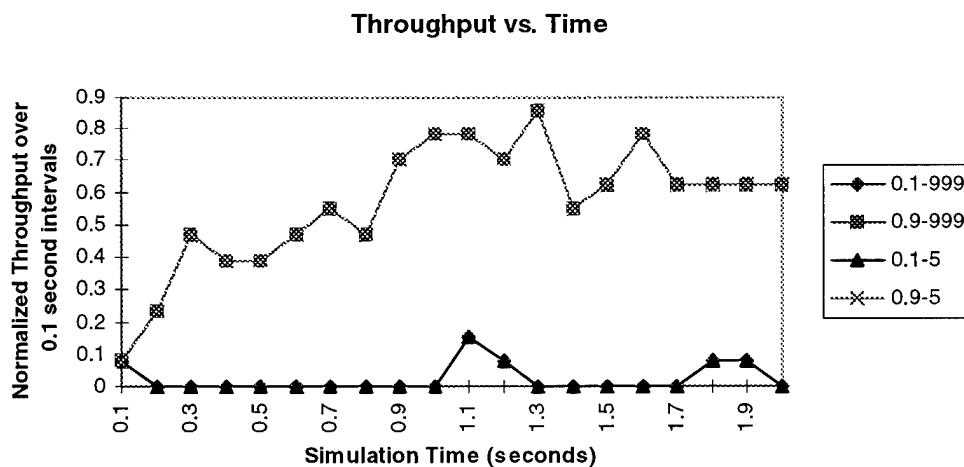
Figure 5-12. Zoomed Version of “Normalized Throughput versus Time over 0.1 second intervals (Start=5 and 999 Load=0.1 and 0.9)”
