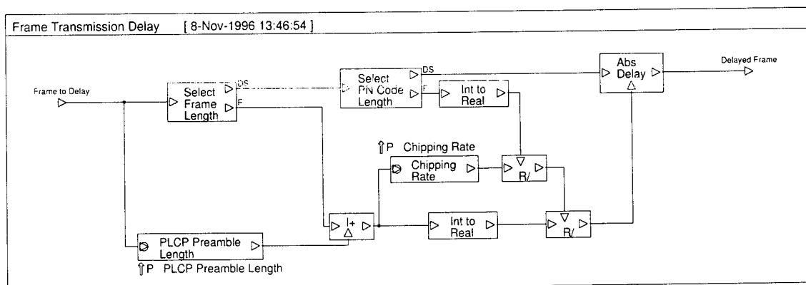
Figure A-17. Frame Transmission Delay Simulation Module
