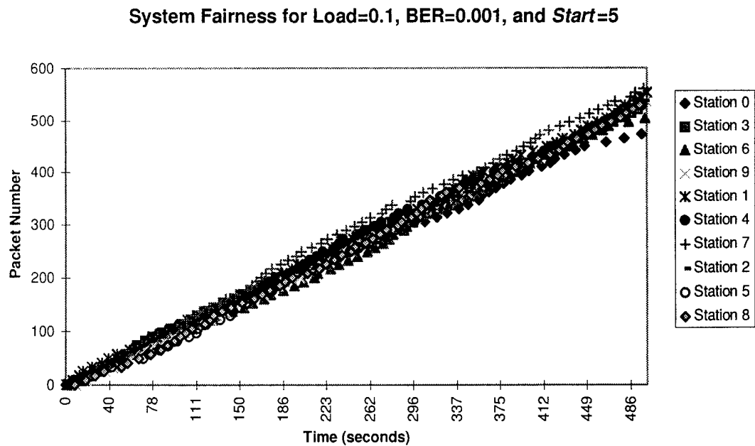
Figure F-2. System Fairness for Load=0.1, BER=0.001, and Start =5
