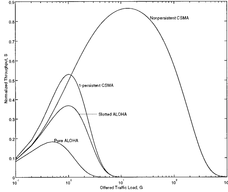
Figure 2-6. Performance of MAC Schemes [Kei89]
