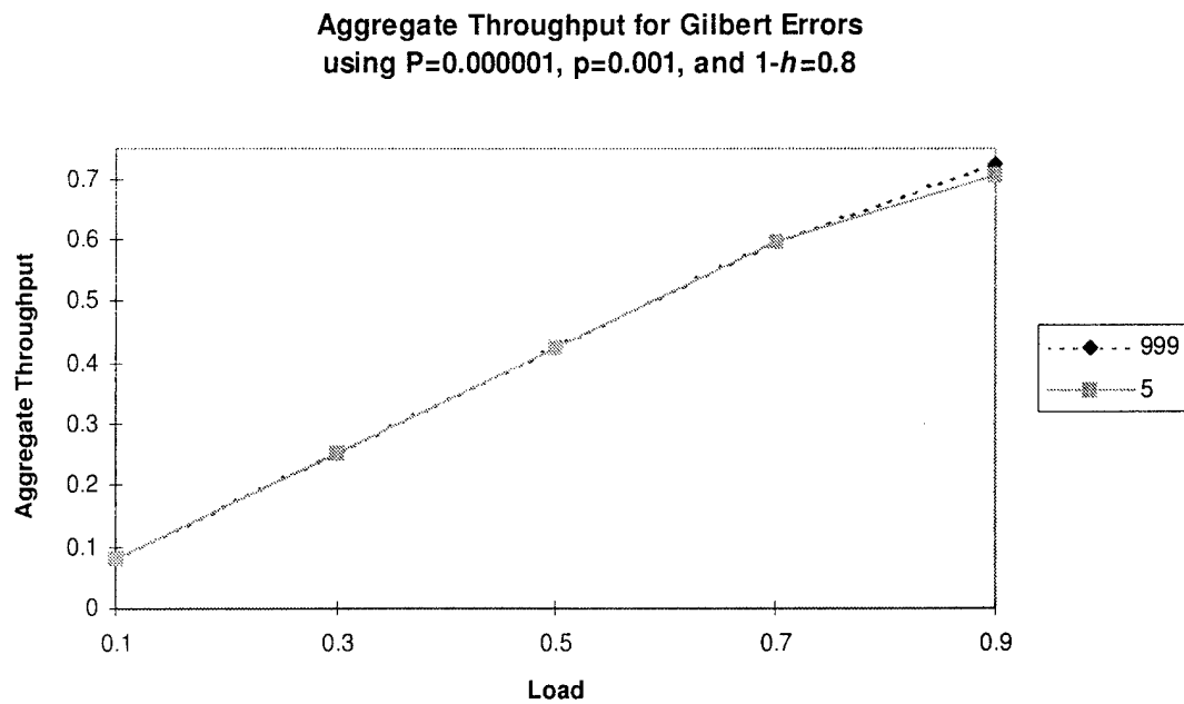
Figure E-12. Throughput for Gilbert Errors ( P=0.000001 , p=0.001 , and 1-h=0.8 )
