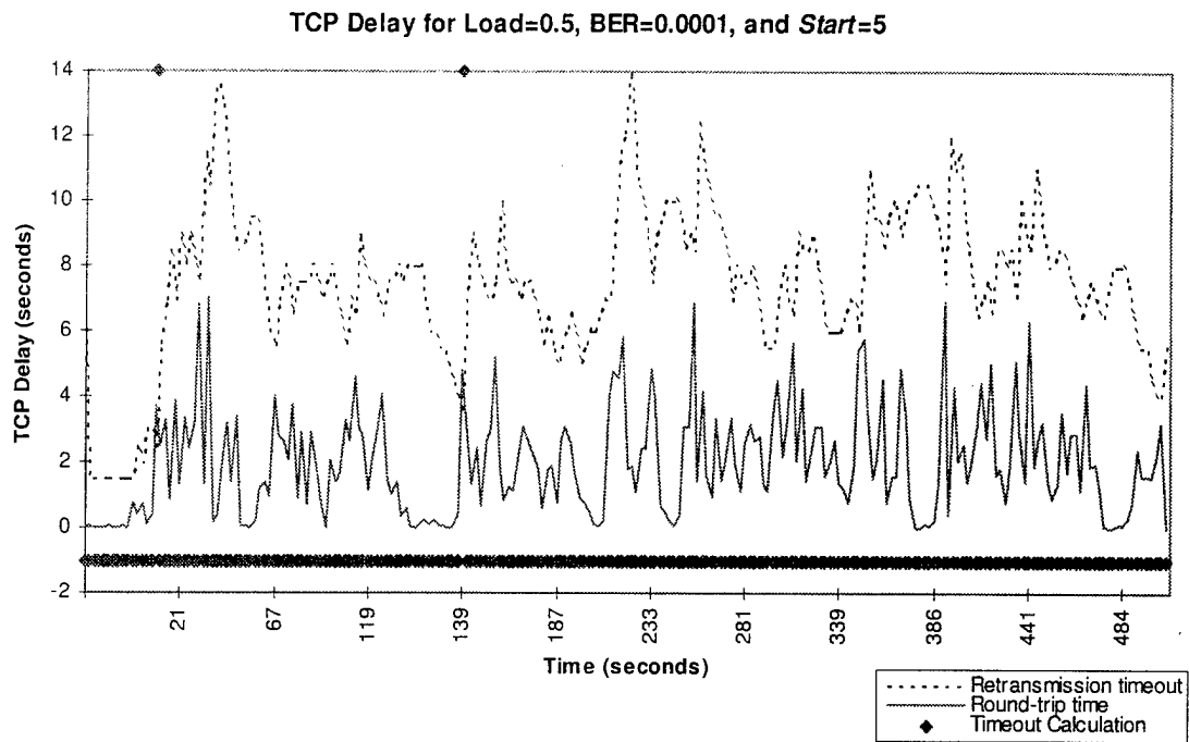
Figure G-7. TCP Delay for Load=0.5, BER=0.0001, and Start=5
