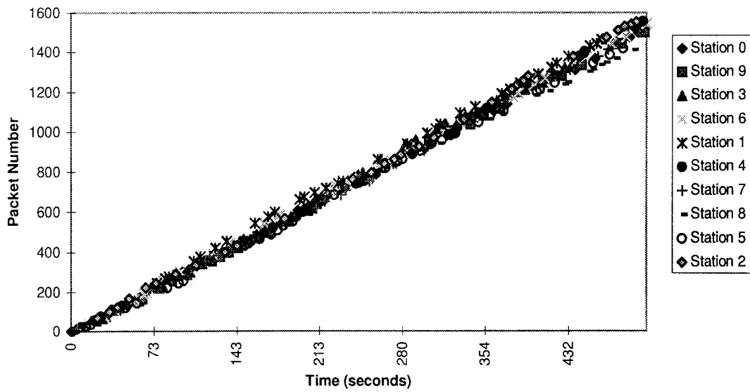
Figure F-9. System Fairness for Load=0.5, BER=0.0001, and Start =5
