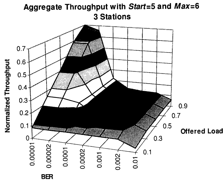
Figure 7-9. Three Station Simulation Results when Start =5 and Max =6
