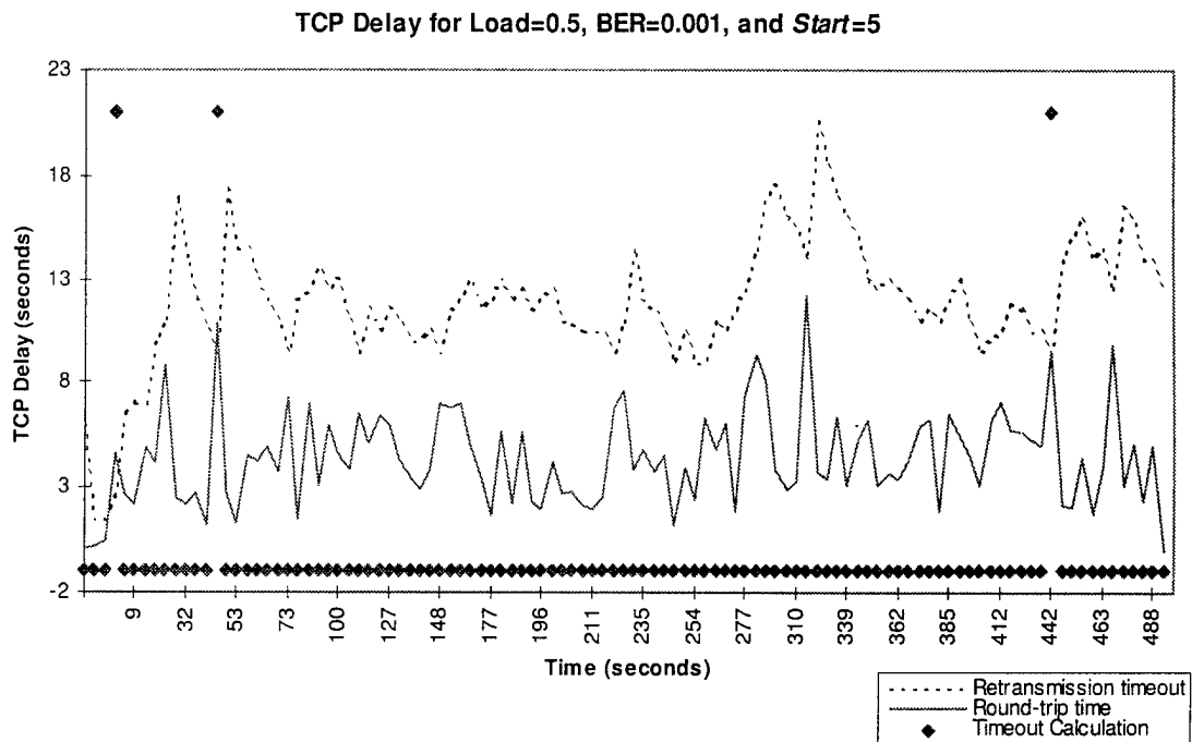
Figure G-6. TCP Delay for Load=0.5, BER=0.001, and Start=5
