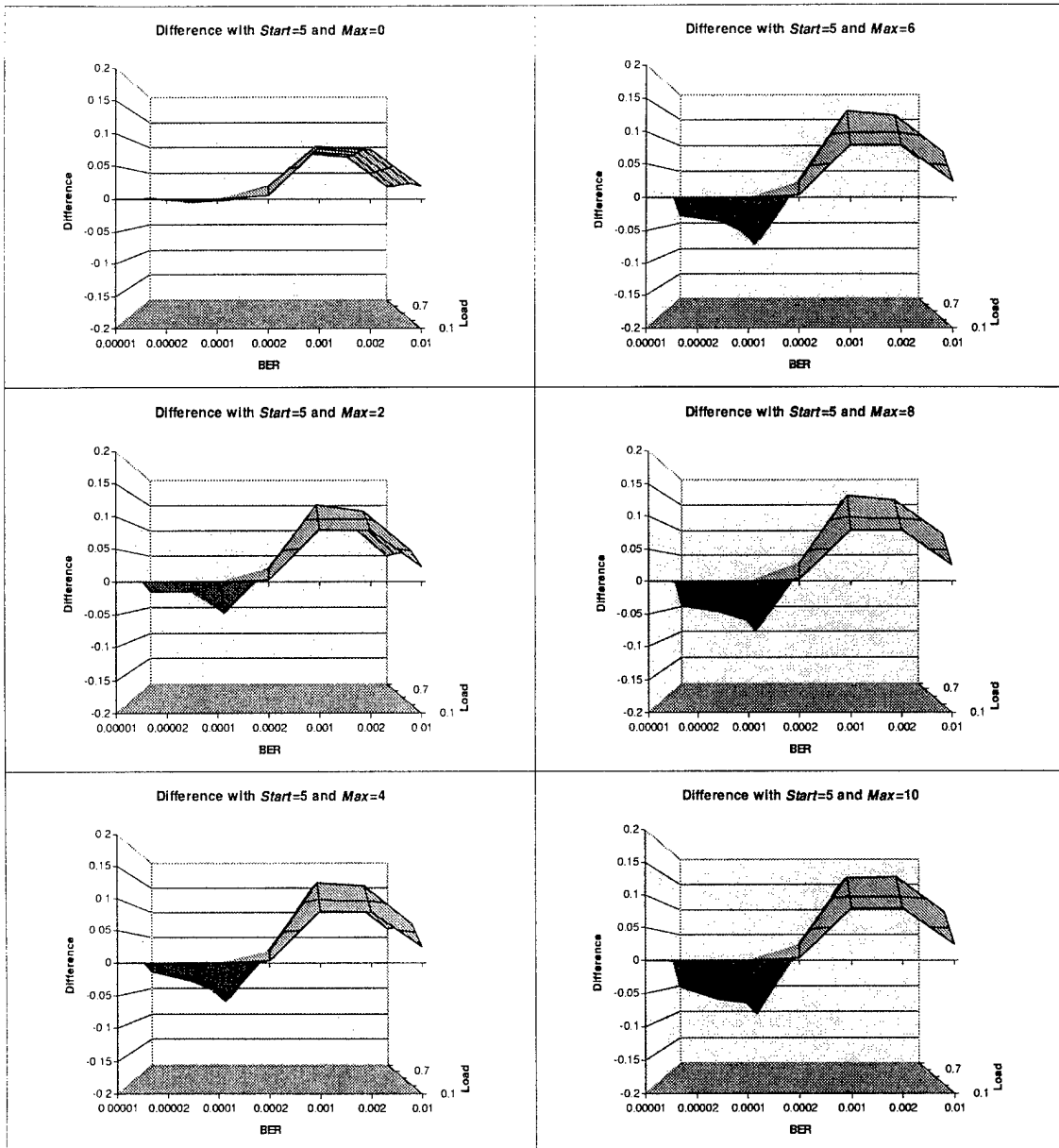
Figure D-3. Difference Plots with Start=5
