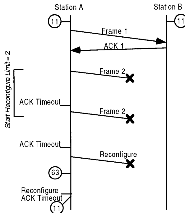
Figure 4-1. Unsuccessful Reconfigure Request Frame
