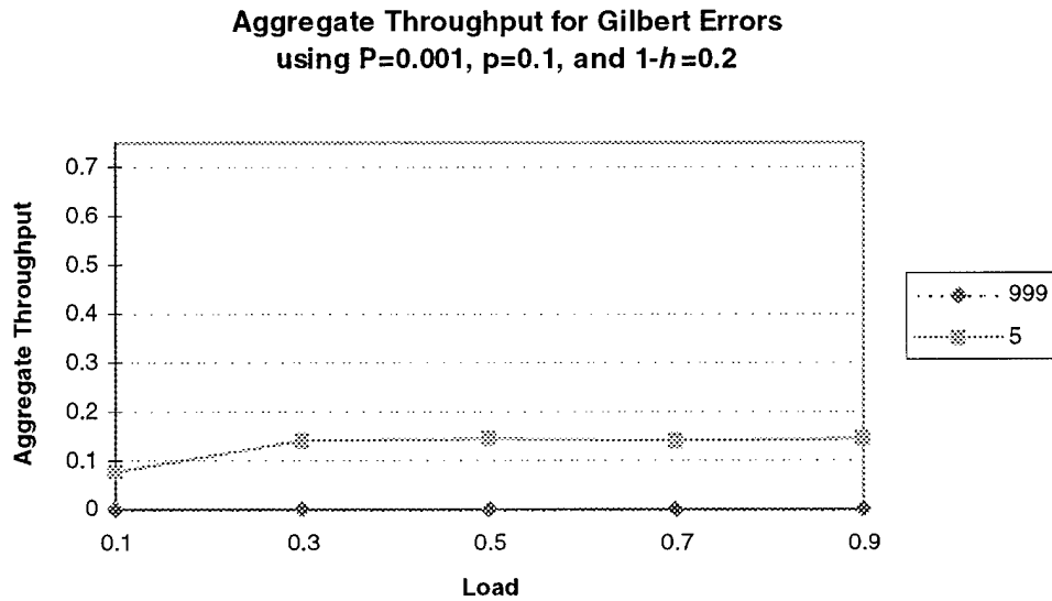
Figure 6-11. Aggregate Throughput for Gilbert Errors ( P=0.001 , p=0.1 , and 1-h=0.2 )
