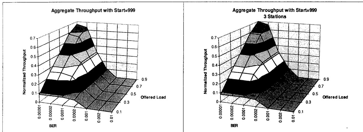
Figure H-9. Aggregate Throughput with Start=999
