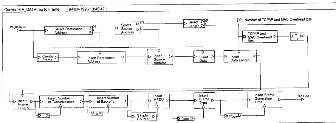
Figure A-13. Convert MA_DATA.req to Frame Simulation Module
