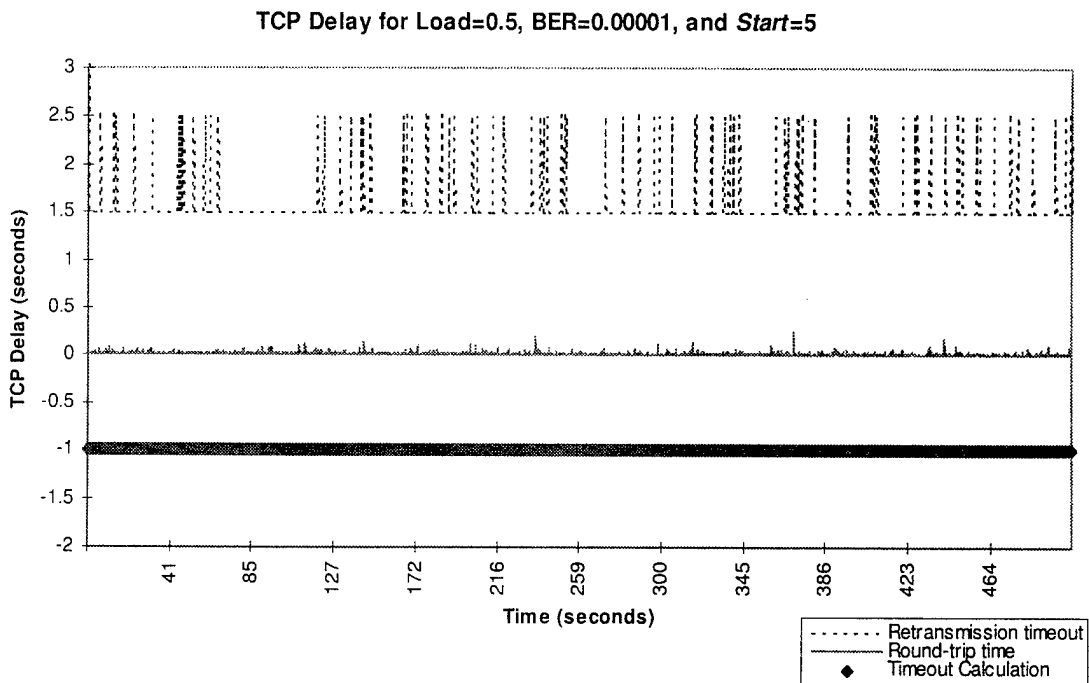
Figure G-8. TCP Delay for Load=0.5, BER=0.00001, and Start=5
