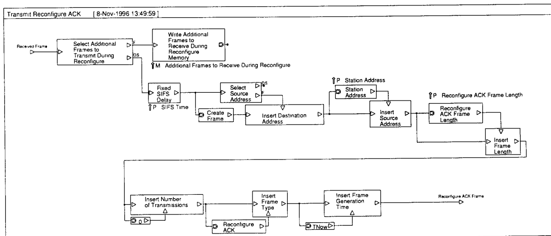
Figure A-26. Transmit Reconfigure ACK Simulation Module
