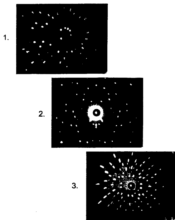
FIG. 10. Several steps in orienting the cubic Si sample for polishing. The reader may be able to identify a distorted axis of twofold symmetry in the first photo; in the second this axis has been aligned so that a second, perpendicular one may be found. Eventual success in this endeavor is shown in the third photo. At this stage in sample preparation, the sample was about 3 mm thick.
