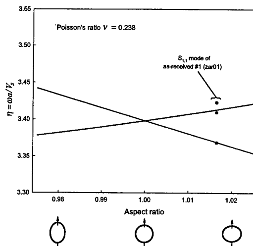
FIG. 40. Nondimensional frequency \eta versus aspect ratio of a spheroid, for the sphere mode S_{1,1} . The dots represent the non-dimensional frequencies corresponding to the peaks in Fig. 39.
