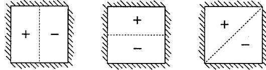
FIG. 73. Three possible degenerate modes of a square membrane; the one on the right is a linear combination of the first two (orthogonal) modes.
