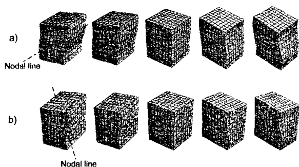
FIG. 74. Two equivalent degenerate shear eigenmodes of the isotropic elastic object considered elsewhere in this section. The figures may be viewed as animations by rapidly scanning back and forth.
