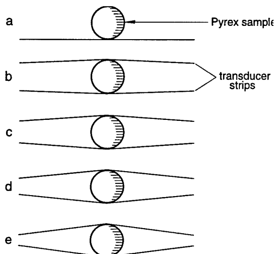
FIG. 41. A schematic representation of the manner in which increasing transducer contact force is applied to a Pyrex specimen in the RUS test cell. The movable transducer block (from Fig. 24) is advanced approximately one half of a screw turn between each measurement, except that there are one-and-a-half turns between (d) and (e).
