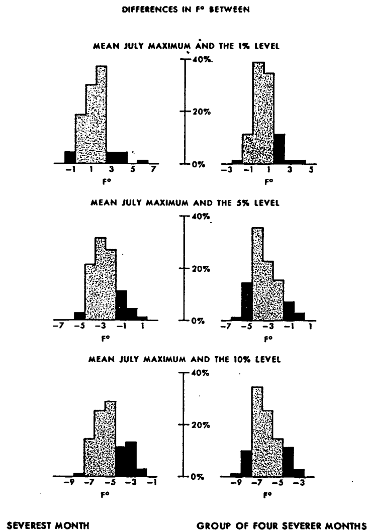
Figure. 5 Differences Between the Mean July Maximum and the 1-, 5-, and 10-Percentile High Temperatures (Williams, 1972)
