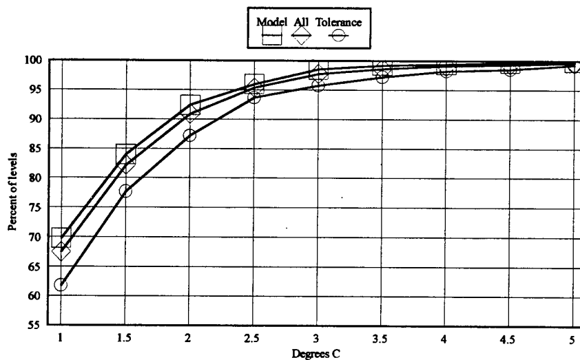
Figure 93. Cumulative Percent of Predicted Levels vs 0.5C Tolerances – April
