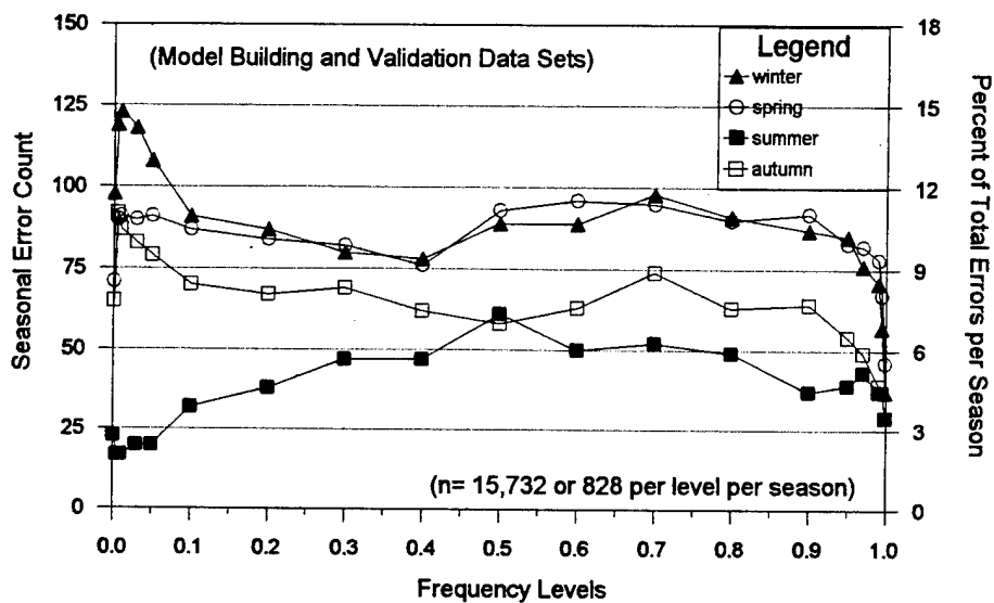
Figure 105. Seasonal Error Counts at Standardized Frequency Levels
