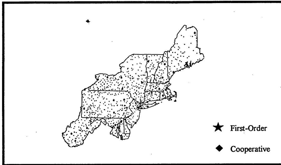
Figure 1. Map of Locations of First-Order and Cooperative Stations in the Northeast (Northeast Regional Climate Center, 1995)
