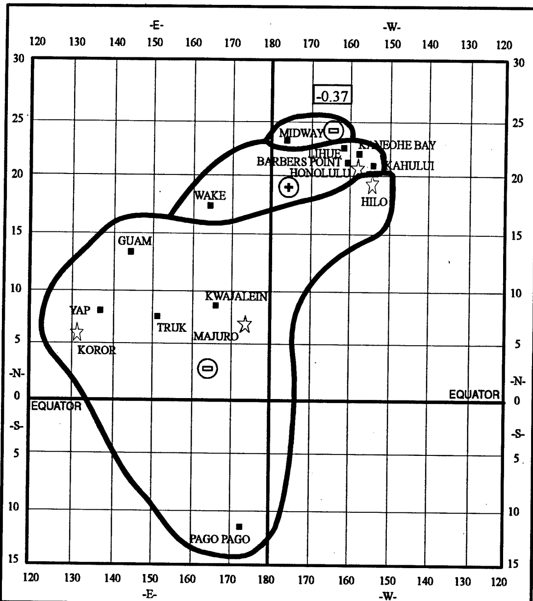
FIGURE 43. PACIFIC ISLANDS TEMPERATURE FREQUENCY GROUP SKEWNESS FOR MARCH
