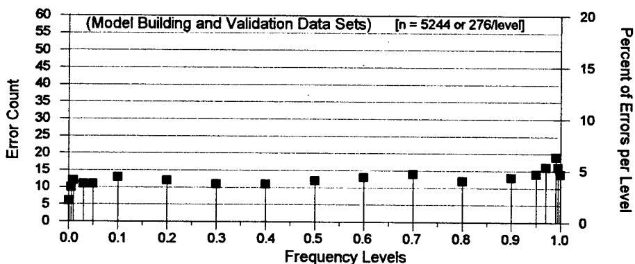
Figure 112. Error Counts at Standardized Frequency Levels for May
