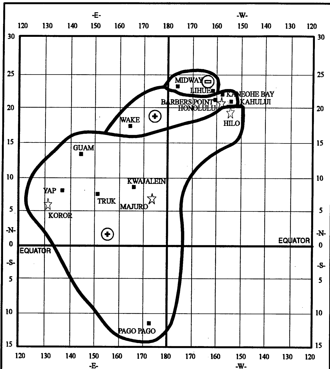
FIGURE 55. PACIFIC ISLANDS TEMPERATURE FREQUENCY GROUP SKEWNESS FOR JUNE
