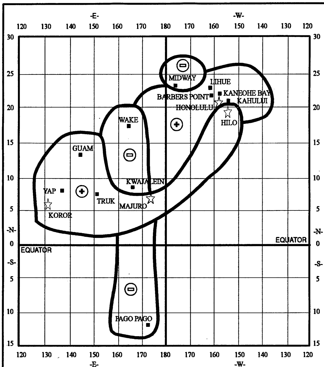
FIGURE 67. PACIFIC ISLANDS TEMPERATURE FREQUENCY GROUP SKEWNESS FOR SEPTEMBER
