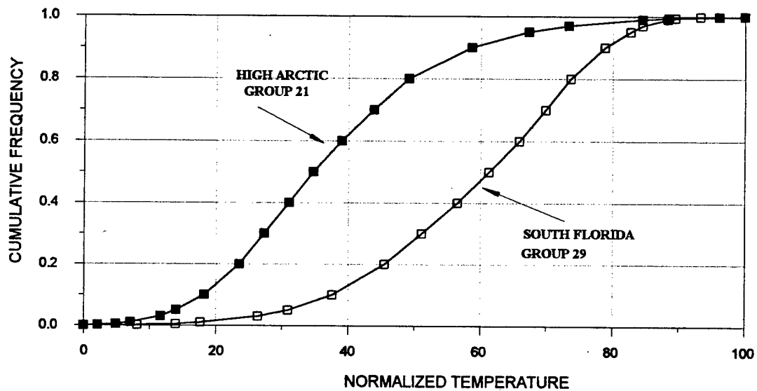
Figure 121. Outer Boundaries for Cumulative Frequency Curves: February
