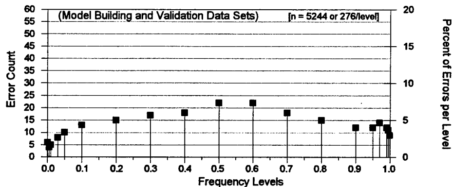
Figure 114. Error Counts at Standardized Frequency Levels for July
