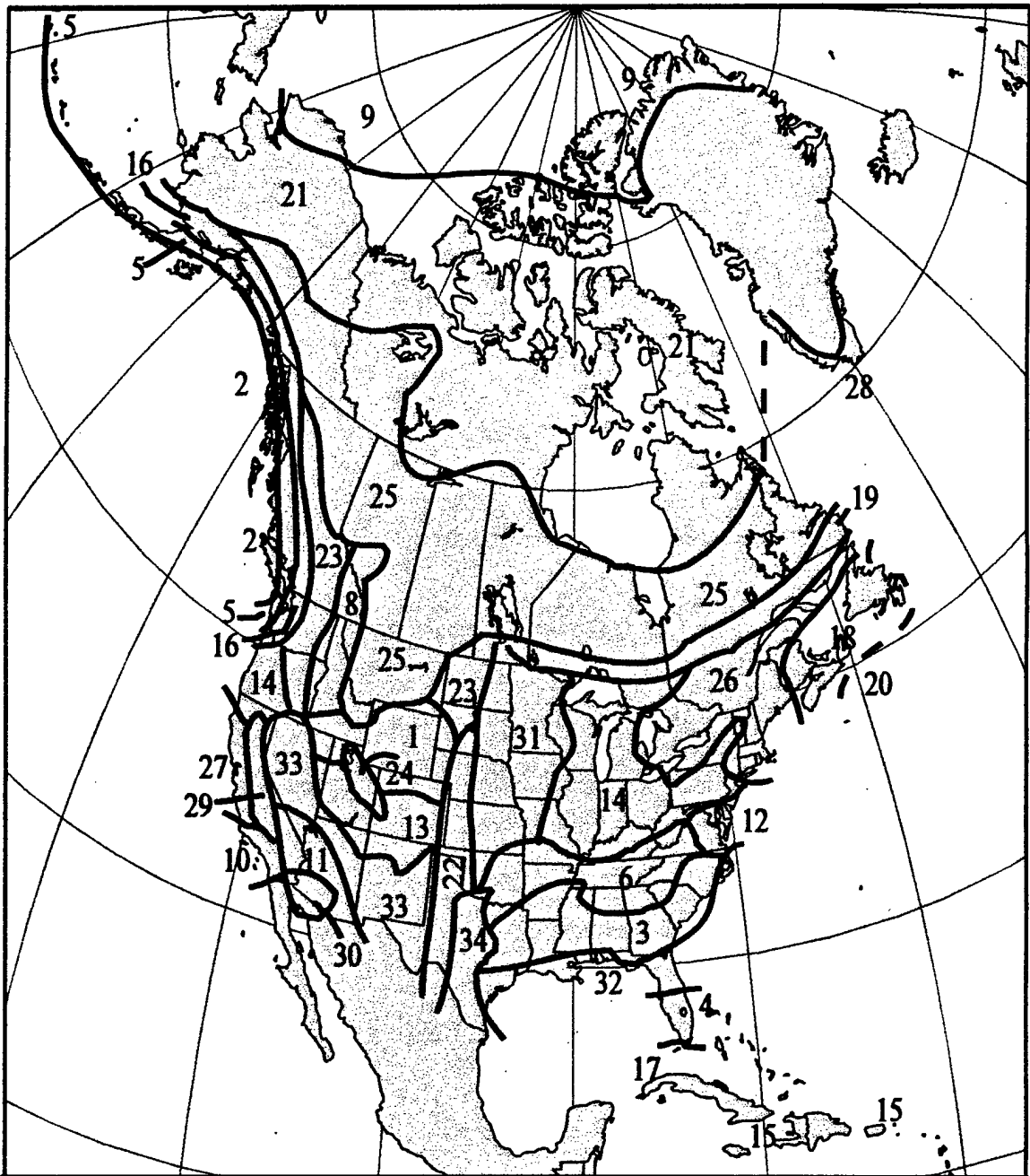
FIGURE 28. NORTH AMERICA TEMPERATURE FREQUENCY GROUPS FOR DECEMBER
