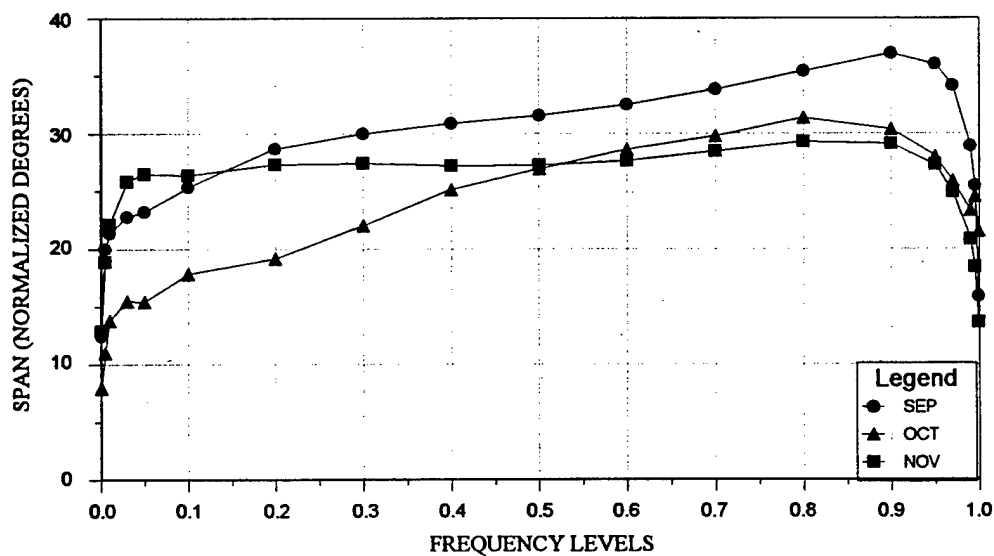
Figure 135, Span at Each Frequency Level: Autumn Months
