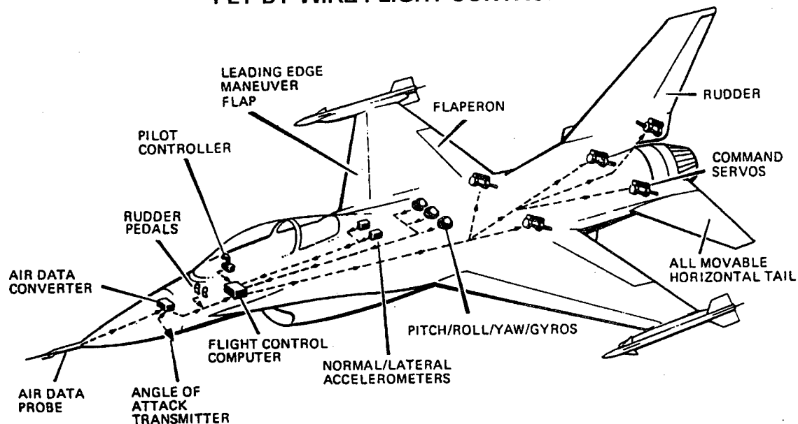
Figure 1: Case Study A Airplane Configuration
