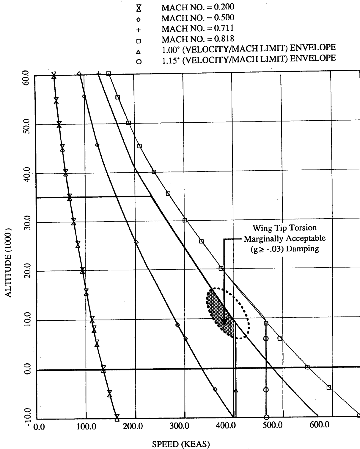
Figure 22: Marginally Acceptable Flutter Enclave For The New Aileron
