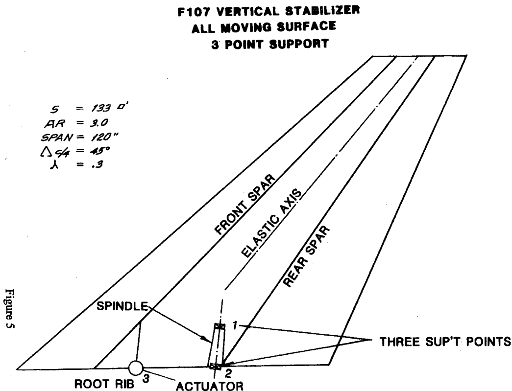
Figure 5: F107 Vertical Stabilizer
