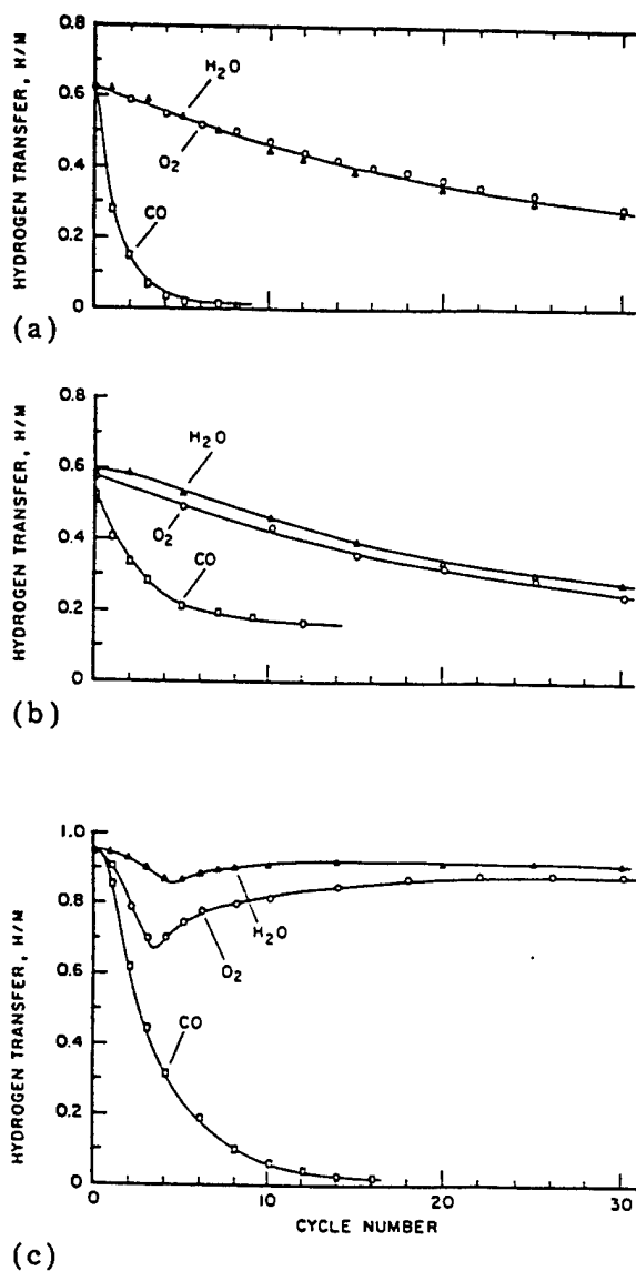
Figure 39 Effect of 300 ppm O_2 , H_2O and CO on the 25^\circ C (H-Capacity) rev of TiFe(a), TiFe_{0.85}Mn_{0.15} (b) and LaNi_5 (c) (Sandrock, 80 (203))
