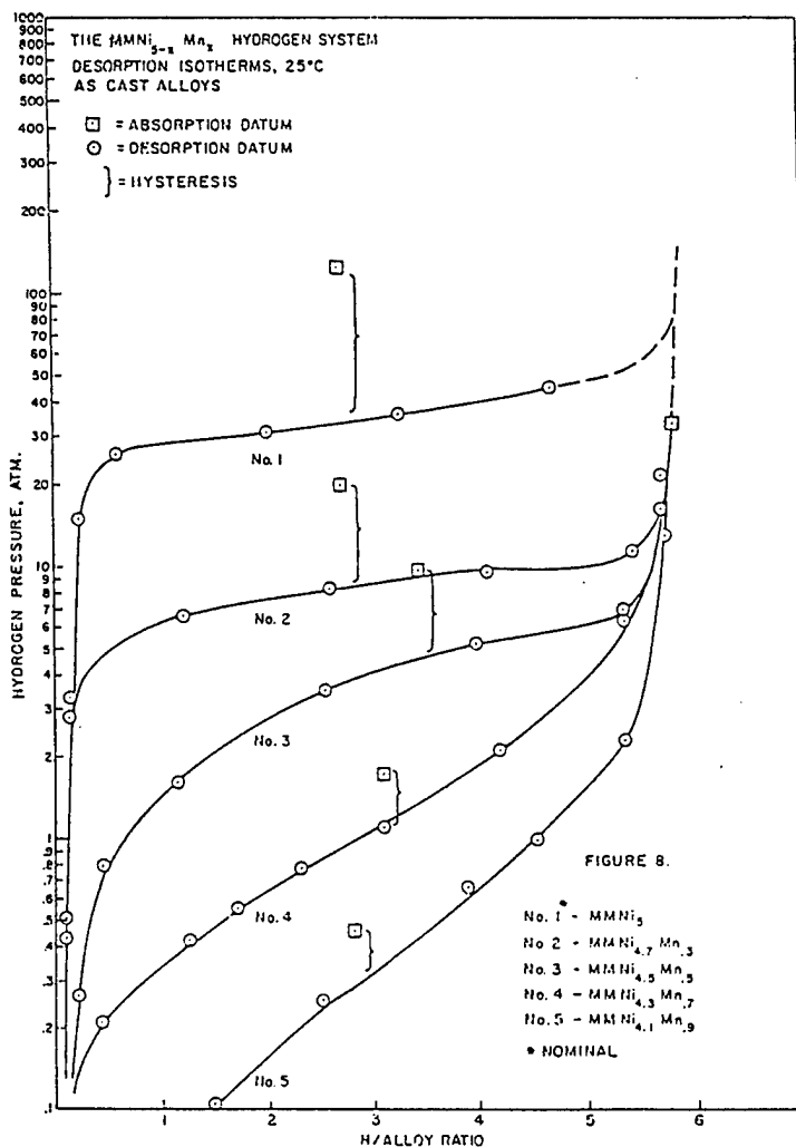
Figure 18 Effect of Mn-Content y on the 25^\circ\text{C} Isotherm of \text{MmNi}_{5-y}\text{Mn}_y (Lundin, 78 (272))
