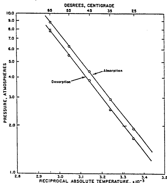
Figure 5: Van't Hoff Plots for \text{LaNi}_5 (Lundin, 75 (260))
