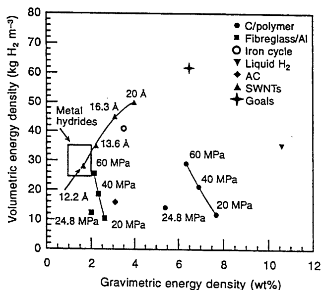
Figure 58 Volumetric and Gravimetric H-Densities for H-Storage Systems Storage Methods: C/polymer = C-wrapped polymer gas cylinders; Fibreglass/Al = fibreglass-wrapped Al gas cylinders; Iron cycle = steam-Fe reaction; AC = activated C; SWNTs = single-walled nanotubes (Dillon, 97)
