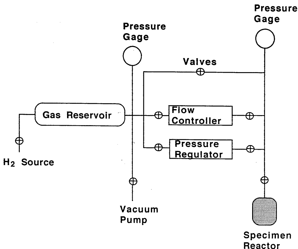
Figure 2: Multipurpose Gas Hydriding/Dehydriding Apparatus
