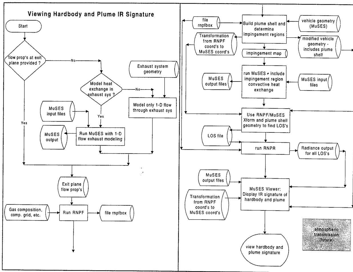
Figure 1. Program Flow of IR Plume Computations.
