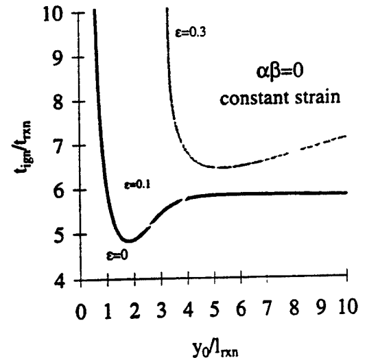
FIG. 3. Nondimensional time for ignition, t_{ign}/t_{rxn} , as a function of dimensionless initial fuel strip thickness y_o/l_{rxn} for different nondimensional constant strain rate values \bar{\epsilon} = \alpha_{rxn} . The case shown is for identical initial fuel and oxidizer temperatures (i.e., \beta = 0 ).
