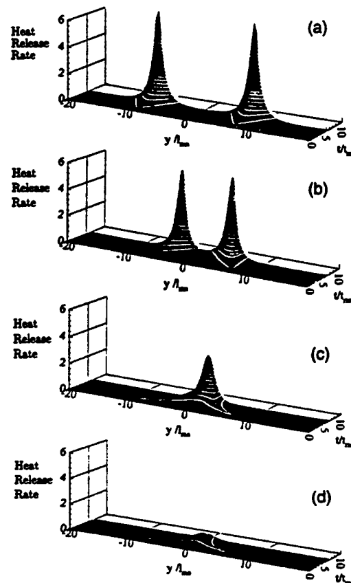
FIG. 2. Evolution of the nondimensional heat production rate (and possible thermal runaway) for the strained fuel strip with dimensionless thickness y_o/l_{rxn} = 8 and constant dimensionless strain rates \bar{\epsilon} = \alpha_{rxn} . Initial temperatures of reactants are equal. Cases shown are for (a) \bar{\epsilon} = 0 , no strain, yielding two independent ignition locations; (b) \bar{\epsilon} = 0.1 , yielding two ignition locations with interdependence of ignition boundaries; (c) \bar{\epsilon} = 0.3 , yielding one single (premixed) ignition point; and (d) \bar{\epsilon} = 0.5 , yielding strain rates too high to allow ignition to take place.
