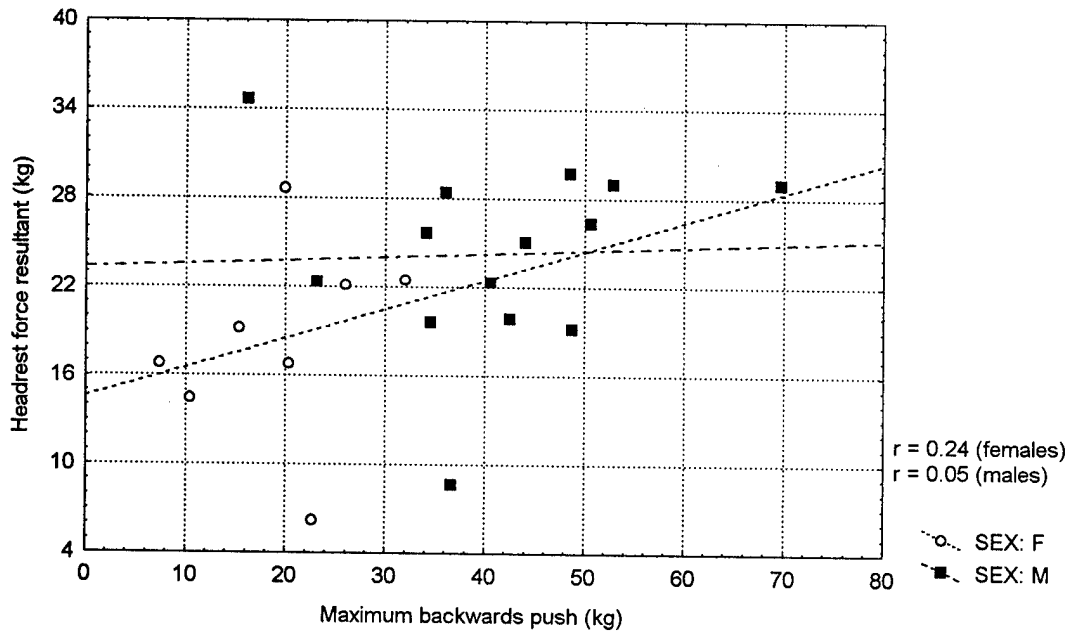
Fig. 9. Motivation Factor ( G_x = -6.5 ) (Headrest resultant force at impact vs. static strength)
