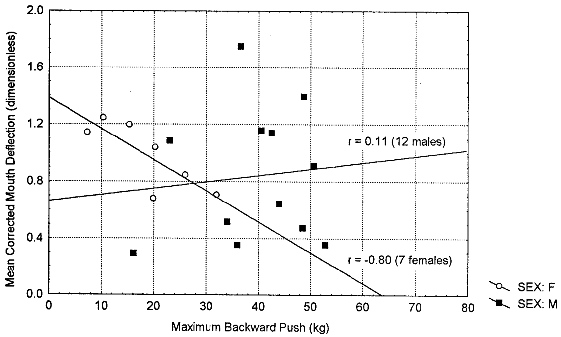
Fig. 4. Mean corrected mouth deflection vs. backward push ( G_x=-6.5 ) (Correlates poorly for males but reasonably well for females).
