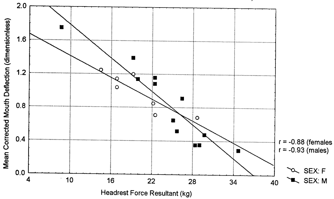
Fig. 7. Mean corrected mouth deflection vs. headrest force ( G_x = -6.5 ) (Head deflection correlates strongly with maximal dorsal-axis neck force).
