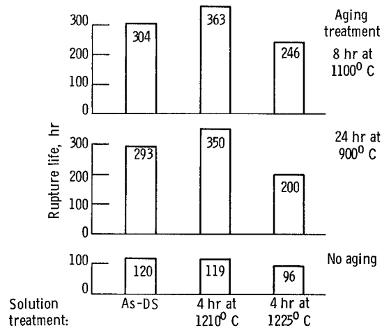
(b) Effect of heat treatment on stress rupture life. (Tests at 870 o C and 515 MN/m 2 (75 000 psi).)
