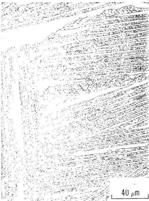
(c) Aging, 8 hours at 1120° C.
