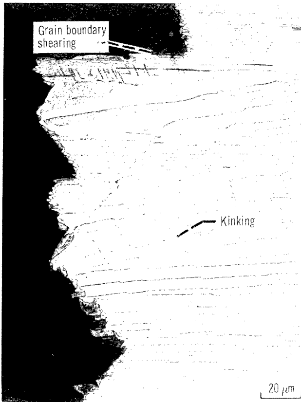
Figure 10. - Microstructural appearance of typical tensile fracture (925°C). (Longitudinal section.)
