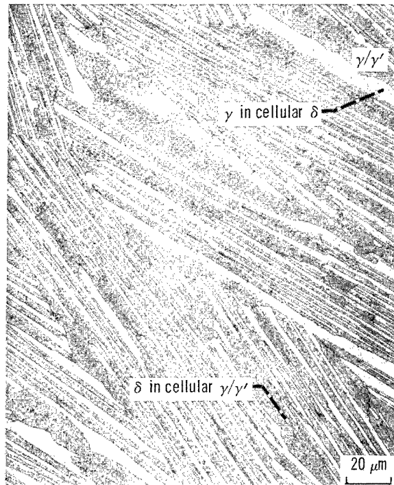
(b) Light micrograph.
