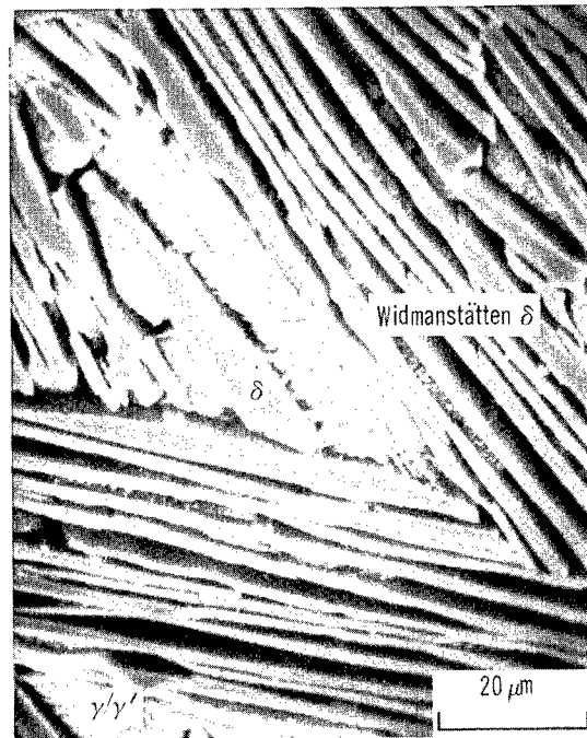
(b) SEM micrograph ( \gamma/\gamma' matrix etched out).
