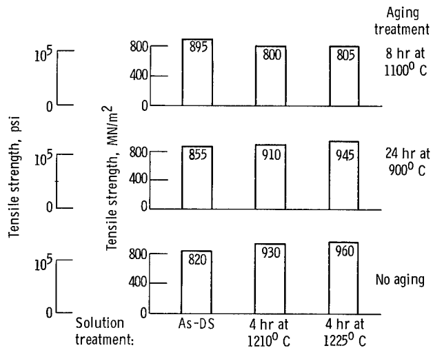
(a) Effect of heat treatment on 925 o C tensile strength.
