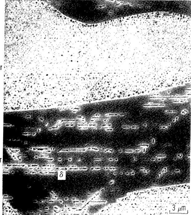
(b) \gamma' solutioned (4 hr at 1225°C) and aged. (Transverse section, SEM micrograph.)
