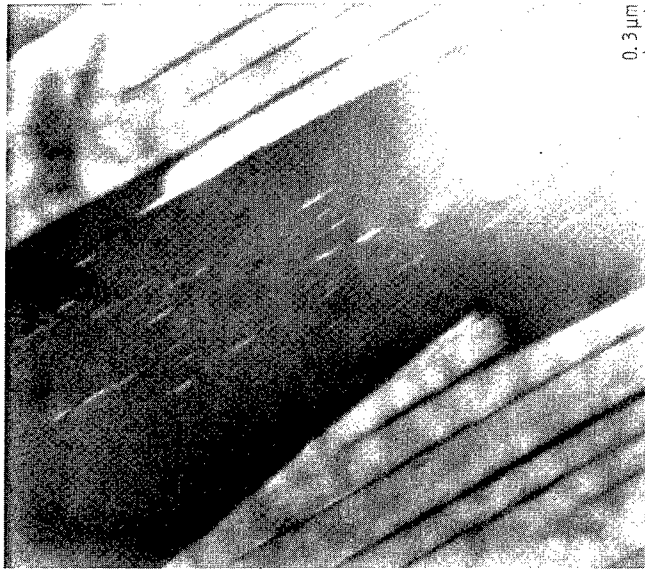
(c) Dark field electron micrograph showing fine precipitates in \delta region (see (a)) using (002) \gamma' diffraction point shown in (b).
