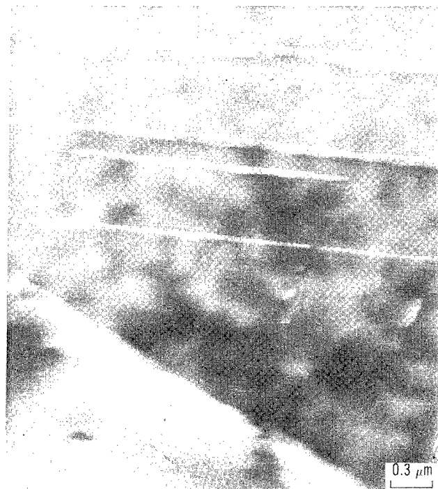
(c) Dark field electron micrograph of lath-like precipitates using [002] \delta diffraction spot shown in figure 14.
