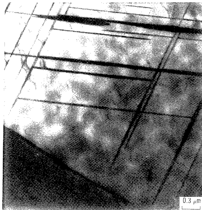
(a) Bright field electron micrograph of lath-like precipitates in \gamma/\gamma' .
