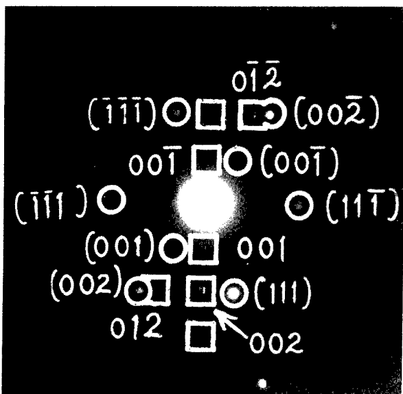
(b) Electron diffraction pattern attained from \gamma/\gamma' region containing lath-like precipitates shown in (a).
