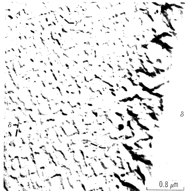
(d) \gamma' solutioned (4 hr at 1225°C) and aged. (Electron micrograph of transverse section.)
