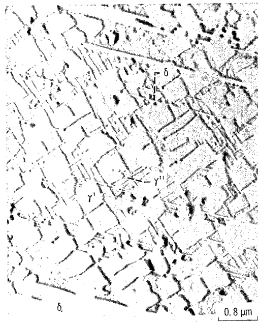
(b) As directionally solidified plus 24 hours at 850° C.
